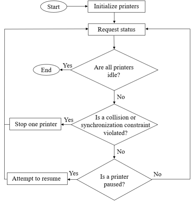
FIGURE 10: ALGORITHM FLOWCHART
