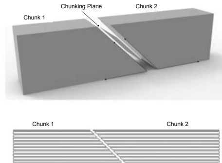
FIGURE 4: SLOPED CHUNKING AND SLICING [8]. CHUNK 2 CANNOT BE PRINTED UNTIL CHUNK 1 HAS BEEN PRINTED.
