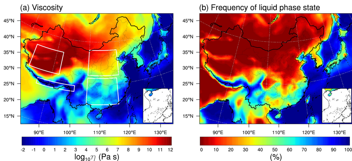
Figure 5. WRF-Chem-predicted (a) median surface values of viscosity and (b) the percent time that an organic aerosol particle is in the liquid phase state during 20 May–23 June 2018. The white boxes in panel (a) specify the selected regions in northern China, southern China, the northern Qinghai–Tibet Plateau, and the southern Qinghai–Tibet Plateau.
