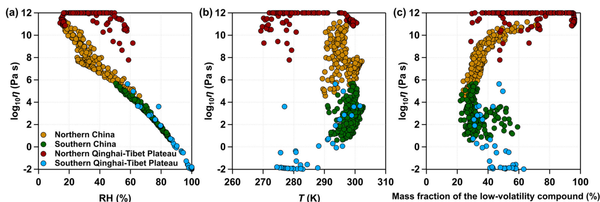
Figure 6. The median values of viscosity as a function of (a) RH, (b) T , and (c) the mass fraction of SOAX ( C^* = 0.1 \mu\text{g m}^{-3} at 298 K) calculated for selected regions in northern China, southern China, northern Qinghai–Tibet Plateau, and southern Qinghai–Tibet Plateau as specified by white boxes in Fig. 5a during 20 May–23 June 2018.
