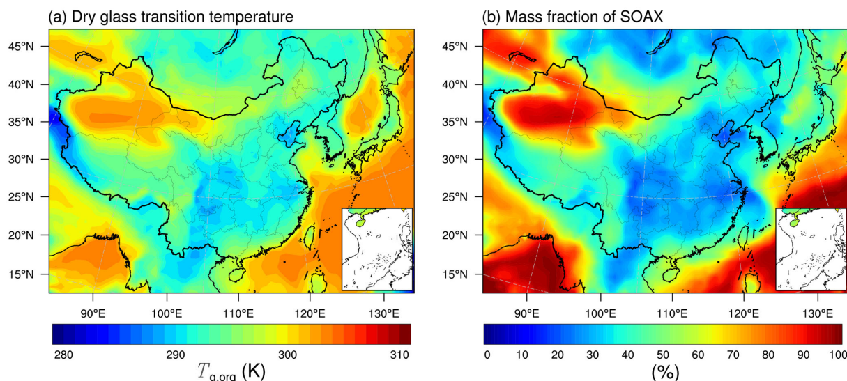
Figure 4. The predicted median surface values of the (a) glass transition temperature of SOA particles at dry conditions and (b) mass fractions of SOAX ( C^* = 0.1 \mu\text{g m}^{-3} at 298 K) during 20 May–23 June 2018 simulated in the base case (Table 1).
