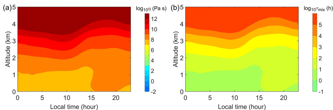
Figure 3. Median diurnal and vertical profiles of estimated (a) SOA viscosity and (b) mixing timescales for organic molecules within 200 nm SOA particles at the IAP site during 20 May–23 June 2018. Note that altitude is approximate and estimated from WRF pressure layers.
