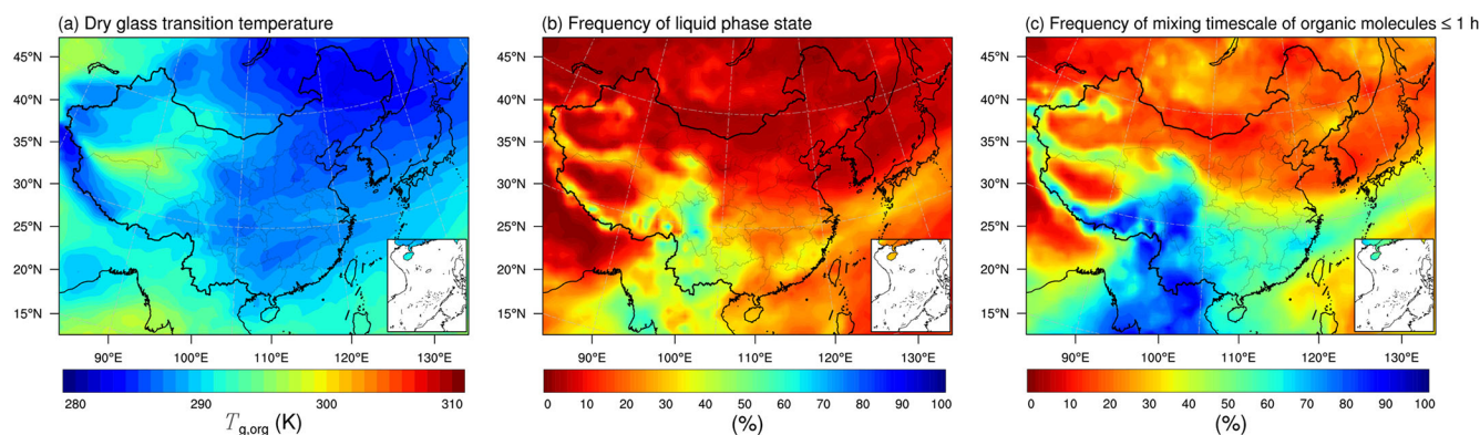
Figure 8. WRF-Chem-predicted median values of (a) the glass transition temperature of SOA particles at dry conditions, (b) the percent time that an organic aerosol particle is in the liquid phase state, and (c) the percent time that the mixing timescale of organic molecules in a 200 nm particle is less than 1 h at 500 hPa during 20 May–23 June 2018.
