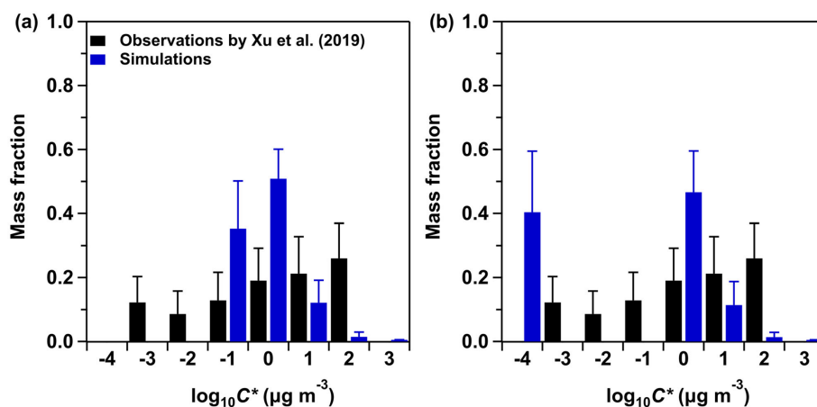
Figure 1. Comparison of the average volatility distributions of observed OOA and simulated SOA at the IAP site during 20 May–23 June 2018. The black bars represent the volatility distributions of observed OOA adopted from Xu et al. (2019). The blue bars represent the volatility distributions of SOA simulated by WRF-Chem, with five C^* bins set to be 0.1, 1, 10, 100, and 1000 \mu\text{g m}^{-3} at 298 K in panel (a) and 0.0001, 1, 10, 100, and 1000 \mu\text{g m}^{-3} at 298 K in panel (b). The blue error bars represent the 1 standard deviation.
