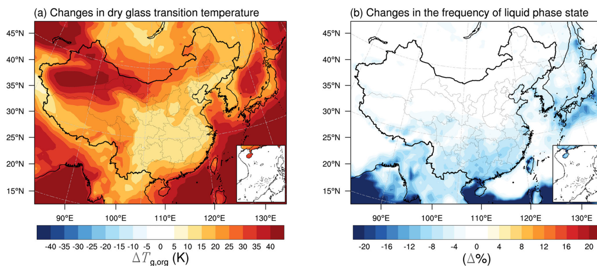
Figure 9. Modeled median differences of (a) the glass transition temperature of SOA particles at dry conditions and (b) the percent time that an organic aerosol particle is in the liquid phase state between a sensitivity case with the lowest C^* of 0.0001 \mu\text{g m}^{-3} at 298 K ( \Delta H_{\text{vap}} of 40 \text{ kJ mol}^{-1} , case A in Table 1) and a base case with the lowest C^* of 0.1 \mu\text{g m}^{-3} at 298 K ( \Delta H_{\text{vap}} of 142 \text{ kJ mol}^{-1} , Table 1).
