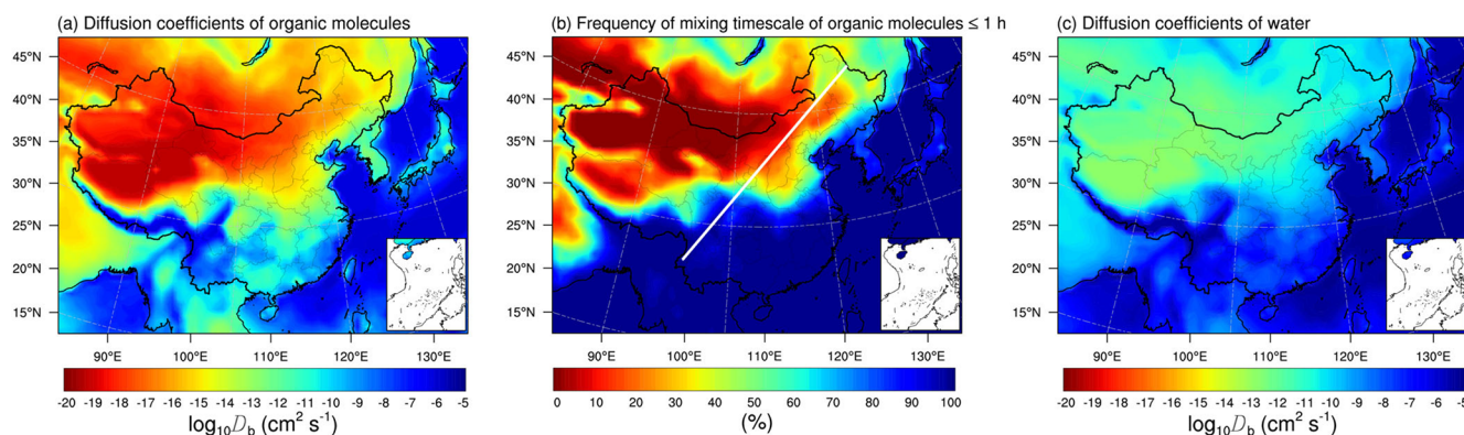
Figure 7. WRF-Chem-predicted median surface values of the diffusion coefficients of (a) organic molecules and (c) water molecules in SOA particles. (b) The percent time that the mixing timescale of organic molecules in a 200 nm particle is less than 1 h during 20 May–23 June 2018. The white line indicates the Hu Huanyong Line (Hu, 1935).
