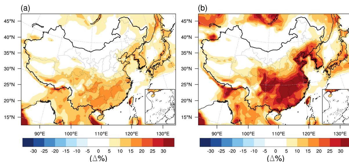
Figure 10. (a) Impacts of RH on the percent time that an organic aerosol particle is in the liquid phase state: modeled median differences between a case with the WRF-Chem-simulated RH increased by a factor of 10 % (case B, Table 1) and a base case (Table 1) with the WRF-Chem-simulated RH. (b) Impacts of the water absorbed by inorganics on the percent time that an organic aerosol particle is in the liquid phase state: modeled median differences between a case considering the water absorbed by both SOA particles and inorganics (case C, Table 1) and a base case (Table 1) considering the water absorbed by SOA particles solely.
