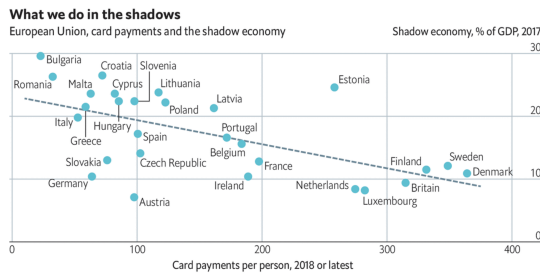
Figure 5: The scatterplot depicting the trend between card payments and the percentage of the shadow economy.
