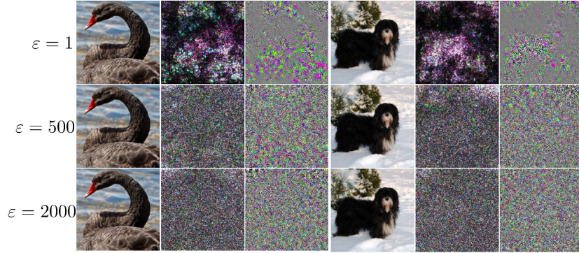
Fig. 6: Stability measure of Equation 7 [best viewed in color]. We only observe salient images for small \varepsilon , as for larger \varepsilon the input x_0 is likely no longer a local optimum. We use the same sample scheme and choices of \varepsilon as Figure 4
