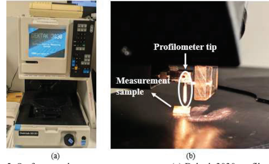
Fig. 5: Surface roughness measurement setup (a) Dektak 3030 profilometer (b) Profilometer tip used for surface roughness measurement of a sample
