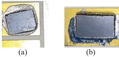
Fig. 12: Shear test results for different Si chip size (a) 6.3 \times 4.5 \text{ mm}^2 , (b) 8.2 \times 4.4 \text{ mm}^2
