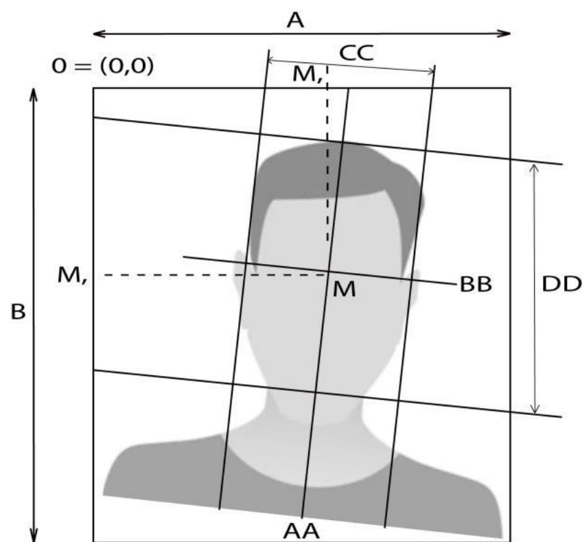
Figure 4. Geometric measurements of the full-frontal face image based on ISO/IEC-19794-5 [34].
