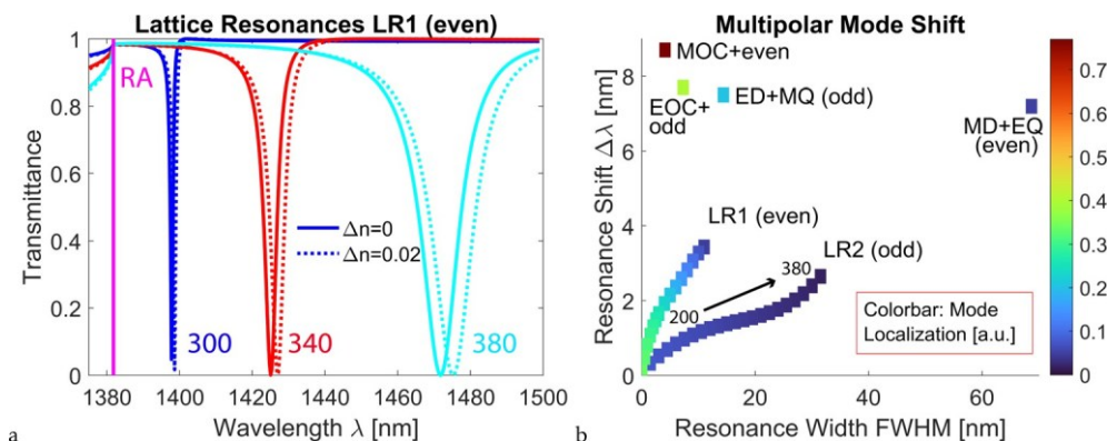
Fig. 3 (a) Transmittance spectra of the nanoantenna arrays supporting lattice resonances. Here, D_x = 940 nm and D_y = 750 nm. The wavelength of the Rayleigh anomaly ( RA ) \lambda_{RA} = n_s D_x is denoted as a vertical magenta line. Three sets of nanoantennas are considered: 300, 340, and 380 nm in dimensions a_x = a_y = a_z . The solid and dashed lines show the spectral features for the unbiased ( Dn = 0 ) and biased ( Dn = 0.02 ) crystal. (b) Summary of resonance shifts for different multipoles: four modes of the dense array and two lattice resonances are considered. The shift is determined for Dn = 0.02 . MD + EQ mode is analyzed for a_x = a_y = a_z = 470 nm, ED + MQ for 550 nm, MOC + odd for 683 nm, and EOC + even for 716 nm. Different dimensions of the nanoantennas are considered to shift their resonances to the same spectral position of \sim 1430 nm. D_x = D_y = 750 nm for all calculations of the dense array. Branches 'LR1' and 'LR2' corresponding to lattice resonances of even and odd multipoles are calculated by varying the nanoantenna dimensions. Branch 'LR1 (even)' is for D_x = 940 nm and D_y = 750 nm, and branch 'LR2 (odd)' is for D_x = 750 nm and D_y = 940 nm. For both branches 'LR1 (even)' and 'LR2 (odd)', the nanoantenna dimensions a_x = a_y = a_z range from 200 to 380 nm. The resonances for the sparse arrays form branches rather than one point, as in the case of a dense array.
