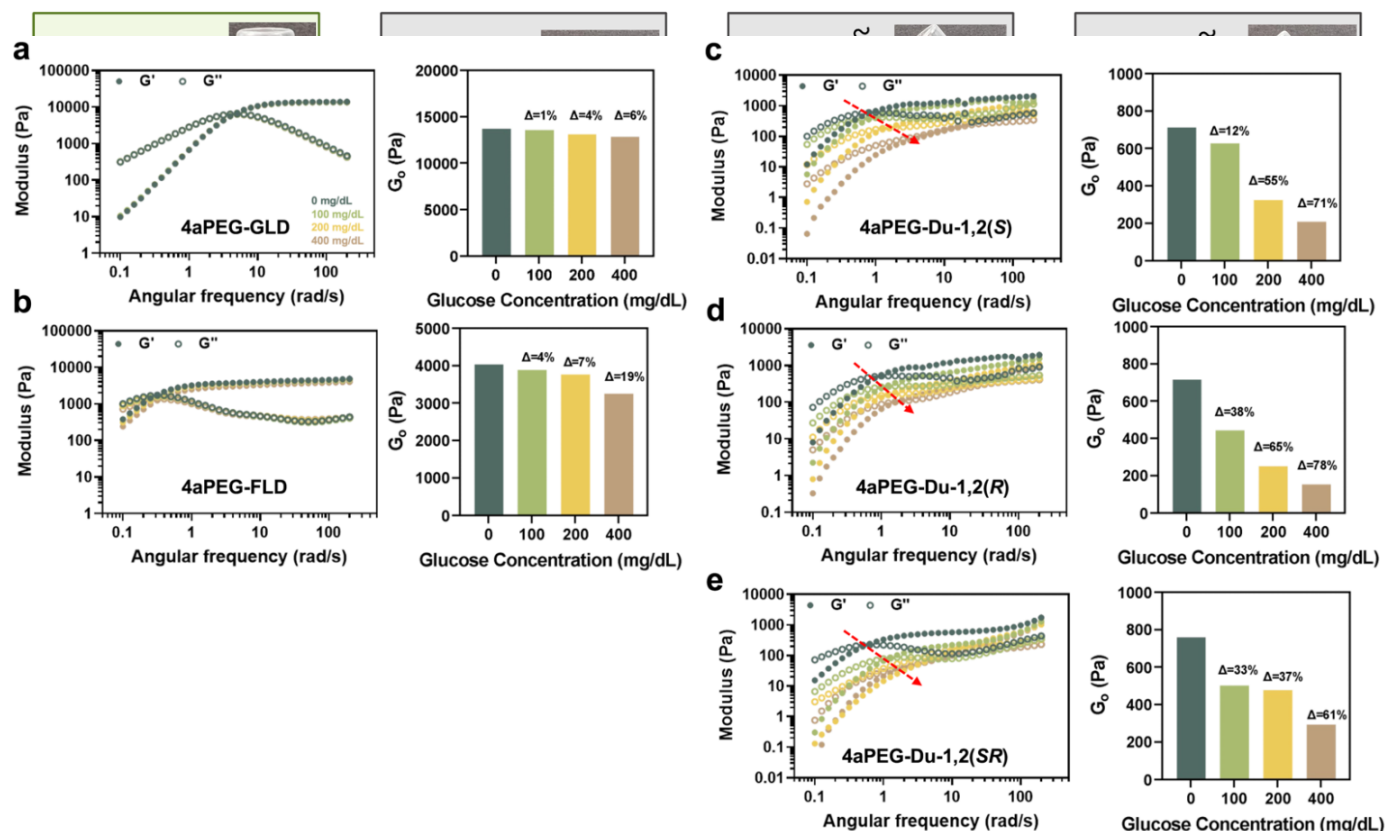
Figure 3. Glucose-dependent oscillatory rheology frequency sweeps ( left ) and comparative G' values (at 20 rad/s) for hydrogels prepared from 4aPEG-FPBA and different 4aPEG-diols, consisting of (a) 4aPEG-GLD, (b) 4aPEG-FLD, (c) 4aPEG-Du-1,2(S), (d) 4aPEG-Du-1,2(R), or (e) 4aPEG-Du-1,2(SR). All samples were prepared at 10% (w/v) in phosphate buffer (0.1 M, pH 7.4). Glucose values ranged from 0–400 mg/dL. For frequency sweeps, G' (closed circles) and G'' (open circles) are both plotted. Red arrows indicate the shift in the G' – G'' crossover ( \omega_c ) in more responsive hydrogels.
