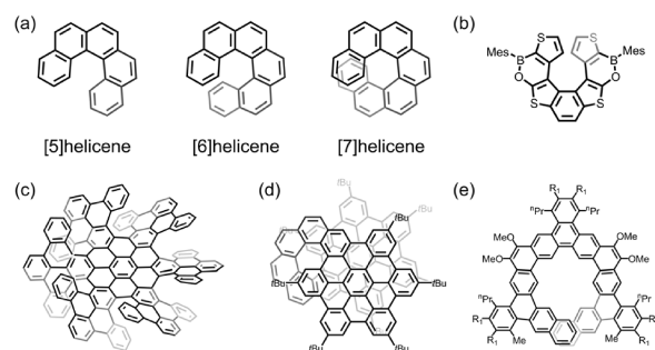
Scheme 1 Depictions of (a) classical carbohelicenes and selected examples of (b) heterohelicene, 1–3 (c) multiple helicene, 15 (d) “hybrid” helicene with periphery 27 and (e) backbone \pi -extension. 40
