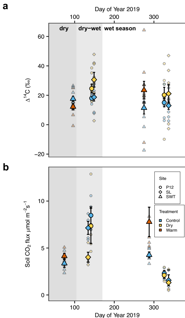
Fig. 4 | Total soil-respired CO 2 flux and 14 C values over 2019 at SWELTR, P12, and San Lorenzo. a. Single time-point 14 C of respired CO 2 at SWELTR ( n = 10 /treatment and time point) and at P12 and San Lorenzo ( n = 4 /site, treatment, and time point). b. Total soil-respired CO 2 flux rates are monthly averages for SWELTR ( n = 5 /treatment and time point) and single time-point measurements at P12 and San Lorenzo ( n = 4 /site, treatment, and time point). The figures show means as large symbols with standard errors and individual measurements as small symbols. Dark gray shading denotes the dry season, light gray shading denotes the dry-to-wet seasonal transition period, and no shading denotes the wet season.
