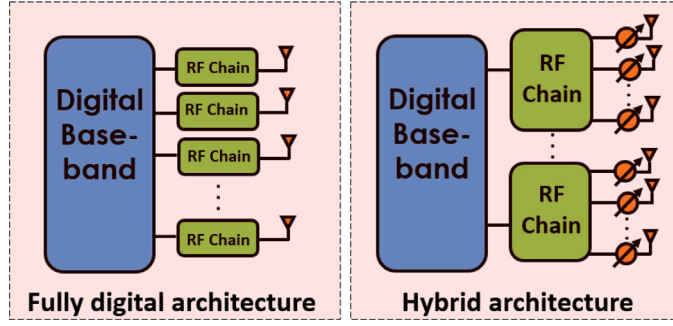
Fig. 1. Illustration of fully digital and hybrid architectures. In fully digital (left), the precise amplitude and phase of signal on each antenna element can be fully controlled. In hybrid (right), the same signal is fed to all antennas connected to the same RF chain, however, the phase of each signal is adjusted by a phase shifter.
