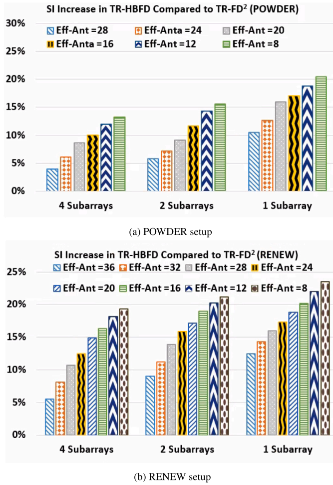
Fig. 6. POWDER and RENEW SI results for joint Tx and Rx beamforming. There is less residual SI compared to using Tx beamforming only. In other words, the gap in terms of SI cancellation between fully digital and hybrid beamforming systems is even less when joint transmit and receive beamforming is used.
