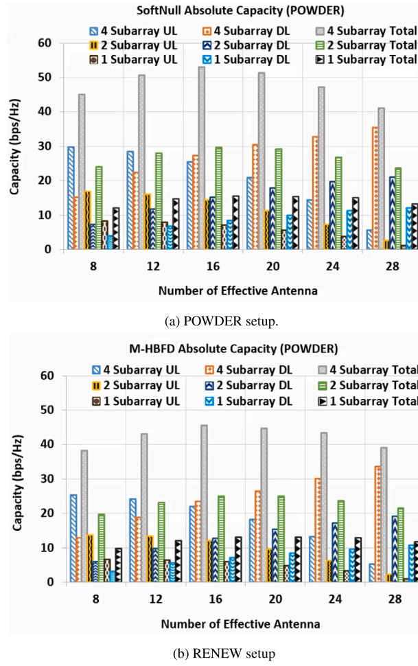
Fig. 8. POWDER absolute capacity results for Tx beamforming only comparing SoftNull and M-HBFD.
