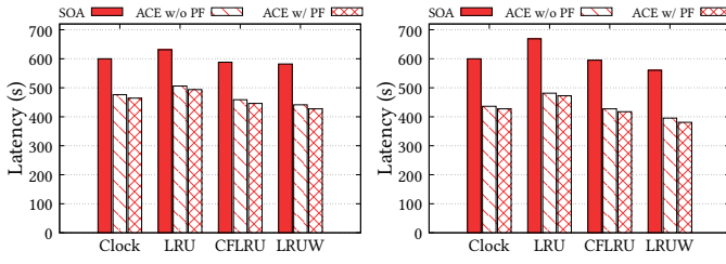
(A) ACE achieves high gain in the mixed workload. (B) Gain of ACE is higher in the write-intensive workload WIS.
