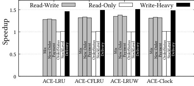
Fig. 6: ACE attains high speedup for TPC-C mixed transaction, while benefiting the write-heavy transaction the most.
