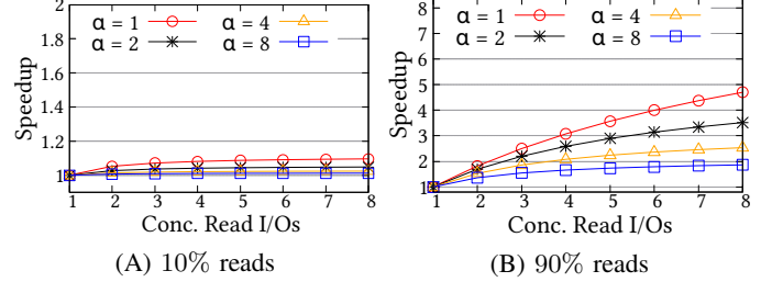
Fig. 3: Highest speedup in read-heavy workloads for Batchable Reads applications. Lower asymmetry results in higher gain.
