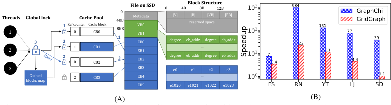
Fig. 7: (A) CAVE's Architecture: block-based file structure (right side) and concurrent cache pool (left side). (B) CAVE performs well across all datasets for PBFS, especially for sparse graphs (RN), while, GridGraph is optimized for dense graphs (SD).
