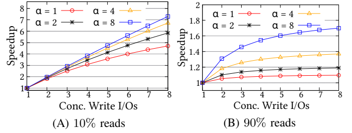
Fig. 2: Speedup is highest for write-intensive workloads and it depends on the asymmetry for Batchable Writes applications.
