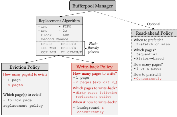
Fig. 4: Bufferpool design space in terms of the design decisions and various options (RED denotes new components)
