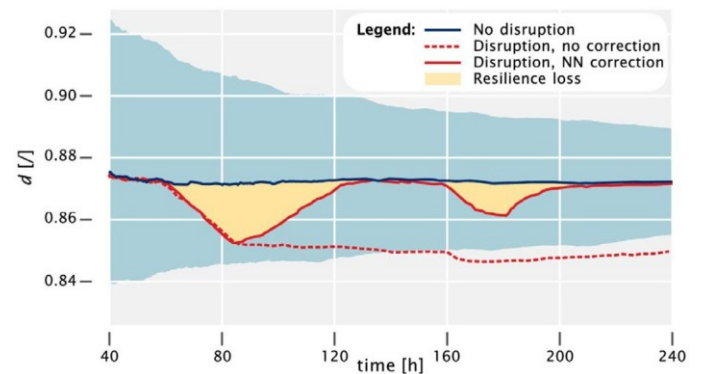
Fig. 9. Reduction of resilience loss after disruption through NN-based DT parameter
