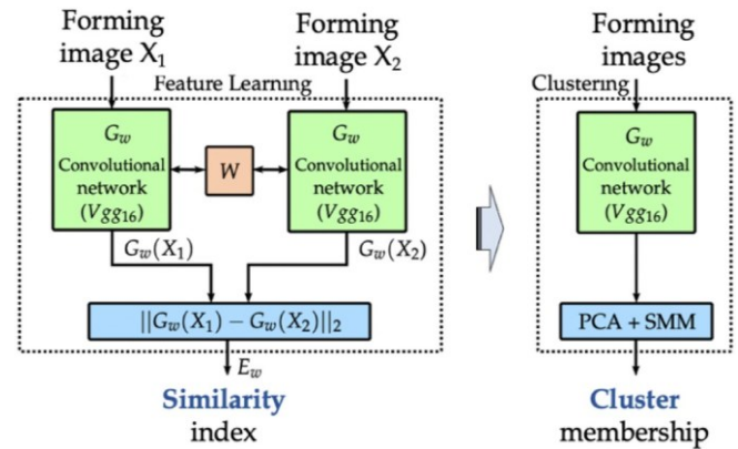
Fig. 13. Supervised feature learning and unsupervised clustering for determination of forming limits,
