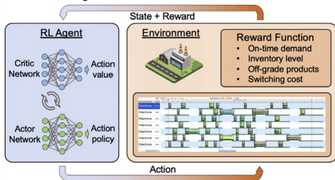
Fig. 33. Actor-critic RL for production scheduling, adapted from [agePRAEnTd 118].
