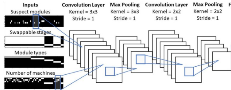
Fig. 10. Deep Q-learning for optimal strategy selection in handling machine breakdown [ be successful in efficiently managing resources of biological material production in a highly uncertain environment [181].gePTRAEnda
