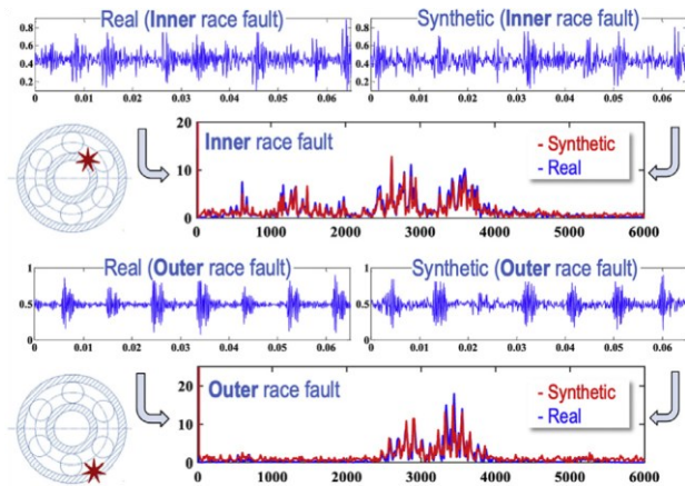
Fig. 22. Consistency between real and synthetic vibration data in time and frequency domains,
