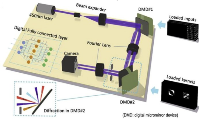
Fig. 40. Setup for optical convolution operation [TRAEndageP 97].
