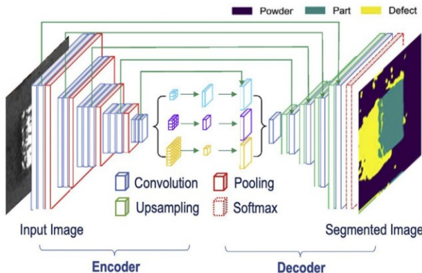
Fig. 19. U-Net for defect segmentation for AM, adapted from [EdagnePTRA 211].
