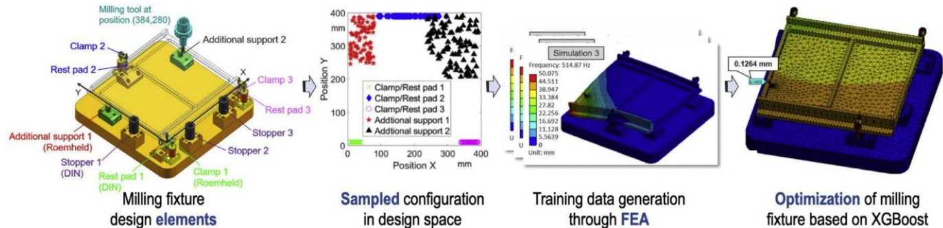
Fig. 12. Fixture design optimization for milling process using FE analysis and XGBoost, adapted from [agednEARTP 60].
