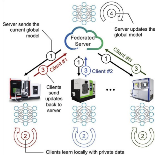
Fig. 20. Schematic of federated learning, adapted from [TdeARnPeGa 127,173].
