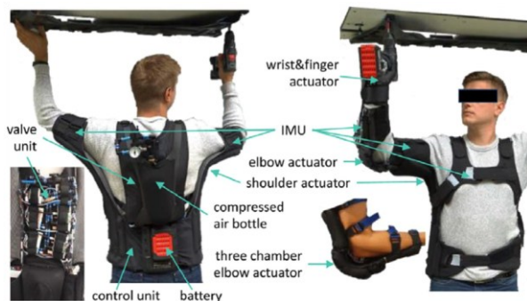
Fig. 32. Soft robotic assist system PowerGrasp. Left: dual arm system, right: single arm
