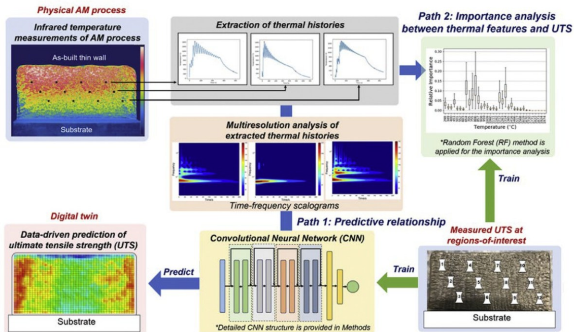
Fig. 15. Mechanistic data-driven method for tensile property prediction in AM, adapted from
