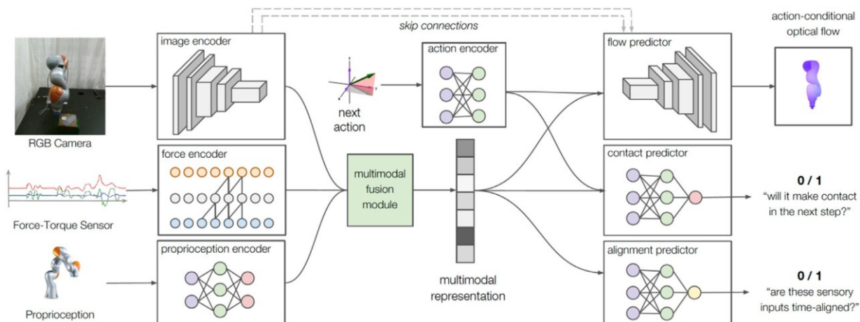
30. Neural network architecture for self-supervised multimodal representation learning of a robotic peg in hole insertion task [AEndagePTR 144].
