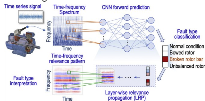
Fig. 23. LRP for interpretable CNN-based motor fault identiRAEndPageT fication [79].
