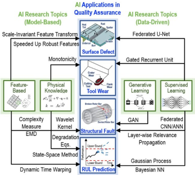
Fig. 18. AI-related research for quality assurance and maintenance.gePTRAEnda
