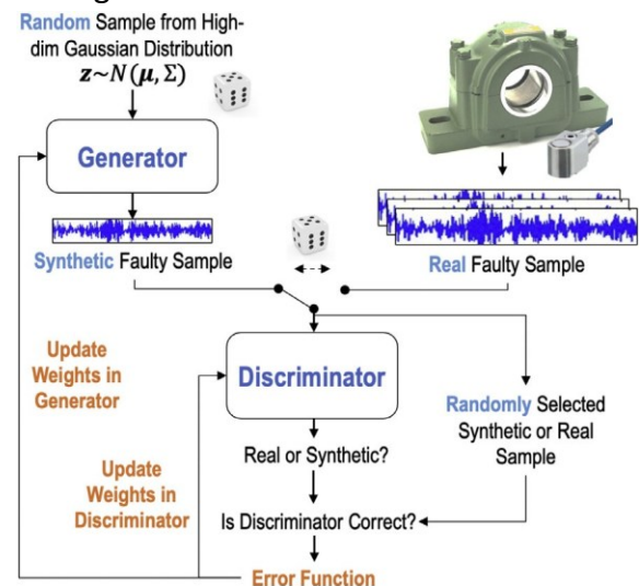
Fig. 21. Schematic of GAN for data synthesis, adapted from [aEgePTRAnd 78].
