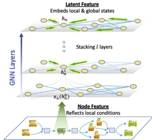
Fig. 5. GNN representation of a manufacturing system [AgaEPendTR 98].
