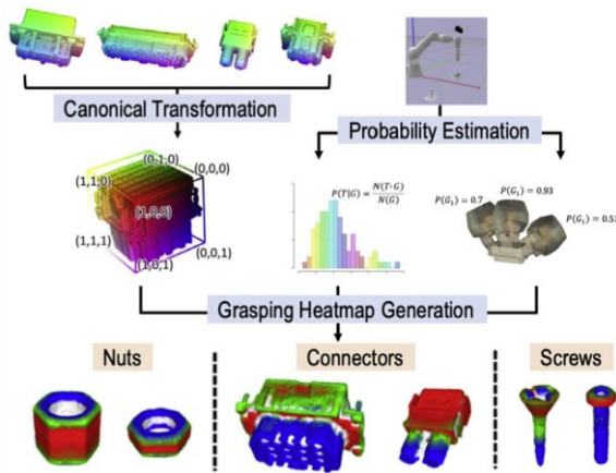
Fig. 28. Robotic grasping learning based on canonical transformation and simulation-
