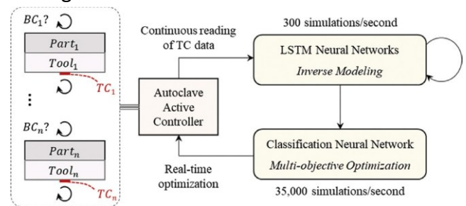
Fig. 17. Schematic of ML framework for inverse modeling of composites processing,
