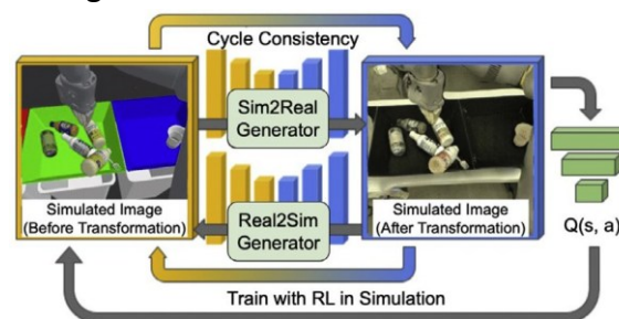
Fig. 27. Transformation of simulated image to support simulation-based robotic grasping learning [209].
