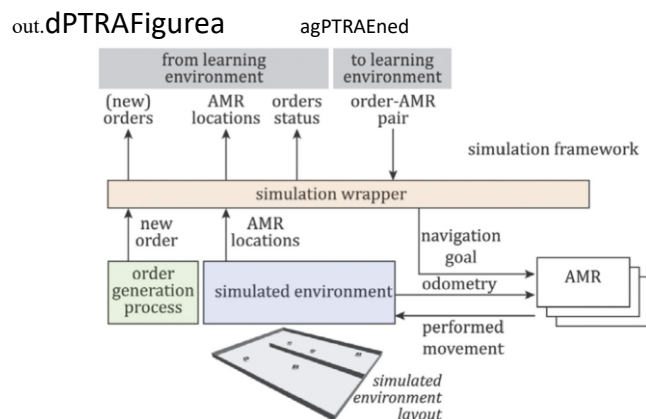
Fig. 26. MARL-based order dispatching, adapted from [TRAndEgeaP 168].
