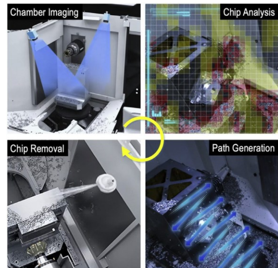
Fig. 34. “AI chip removal” system from DMG Mori [ePTRAEndag 50].
