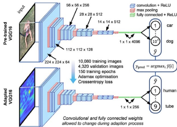
Fig. 31. VGG16 structure and adaption to time-frequency images [dPageTRAEn 262].
