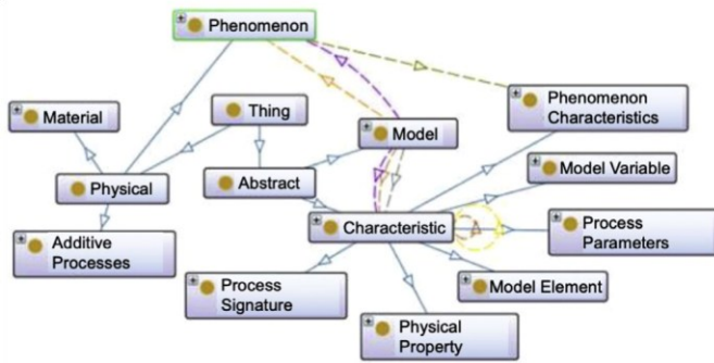
Fig. 4. OWL for additive manufacturing, adapted from [ndagePTRA 162].
