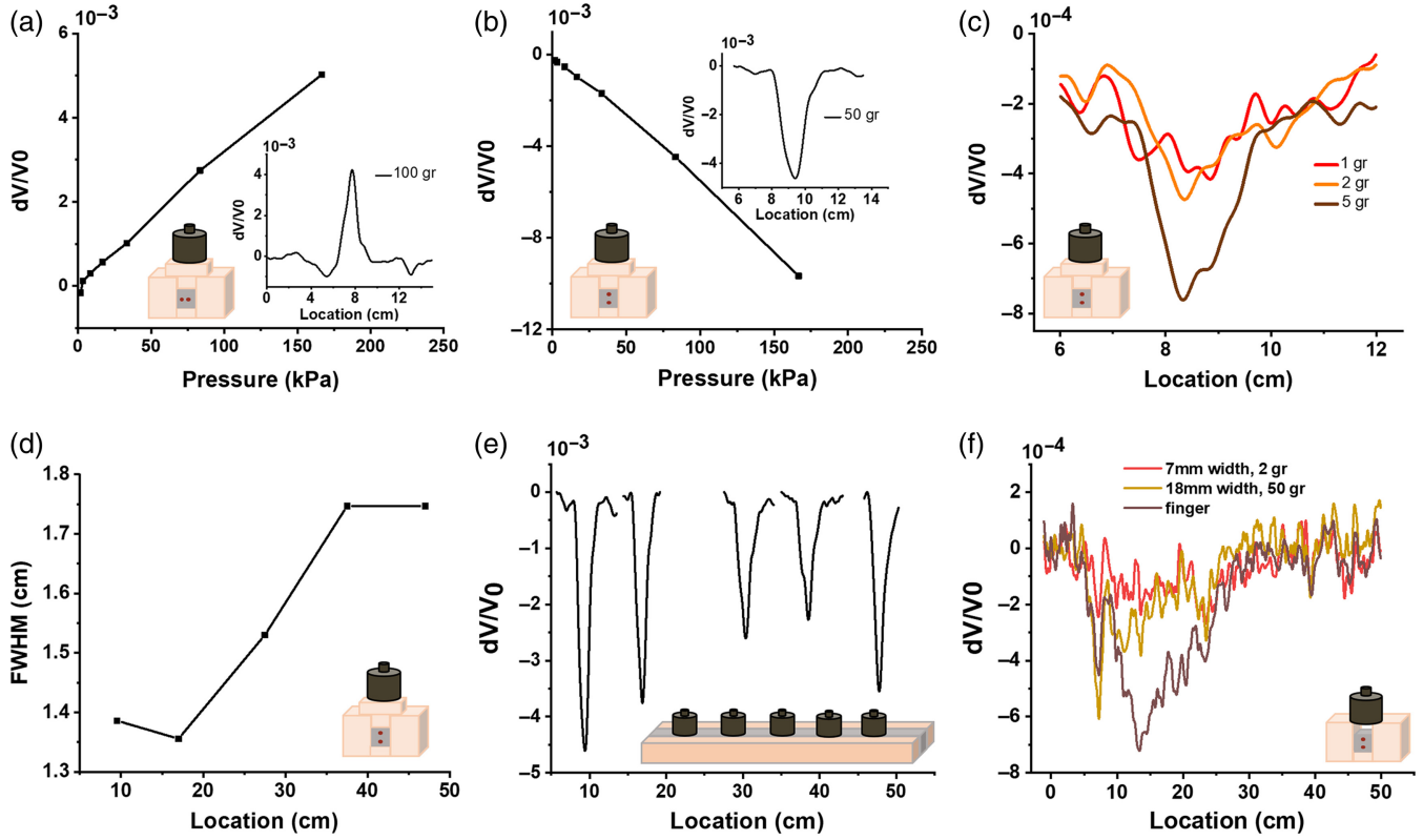
Fig. 5 TDR measurements of the multimodal fiber antenna under different configurations. (a) The sensitivity curve when the metal wires are placed horizontally (horizontal configuration). Inset, an example of a measurement with 100 gr. (b) The sensitivity curve when the metal wires are placed vertically (vertical configuration). Inset, an example of a measurement with 50 gr. (c) Sensitivity measurements in the vertical configuration, using light weights of 1, 2, and 5 gr. (d) Spatial resolution in the vertical configuration. (e) Distributed pressure measurement using 50 gr at 9.5, 17, 27.5, 37.5, and 47 cm in the vertical configuration. (f) Proximity measurement without the plastic pedestal used in the pressure measurements. The weights used in this case have a footprint diameter of 7 and 18 mm for the 2 and 50 gr weights, respectively. In addition, an index finger with a width of \sim 13 mm is used in the measurements.
