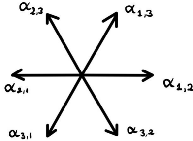
Figure 2: Root system of \mathrm{GL}_3
