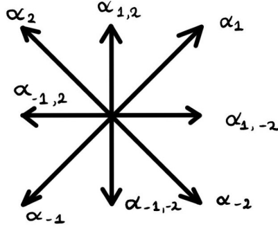
Figure 3: Root system of \text{Sp}_4
