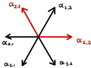
Figure 4: Root system of \text{GL}_3 with a choice of basis \Delta = \{\alpha_{1,2}, \alpha_{2,3}\} in red
