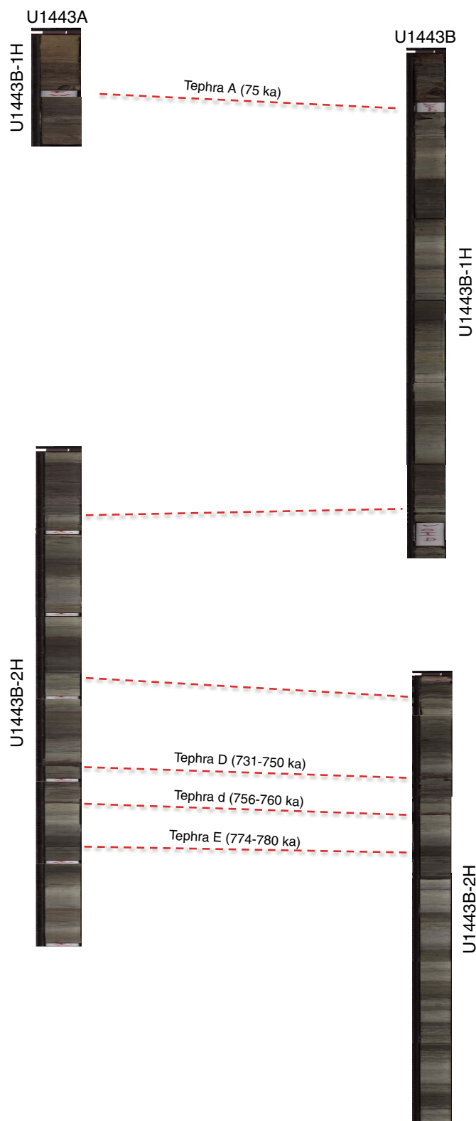
Figure F20. Holes U1443A/U1443B correlation of Cores 353-U1443A-1H through 2H and 353-U1443B-1H and 2H, indicating a 5.4 m gap at the base of Core 353-U1443A-1H.
