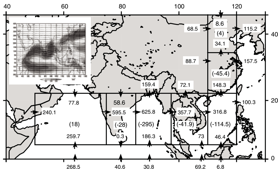
Figure F8. Summer monsoon moisture budget and transport path (inset) after Ding et al. (2004). Moisture budget averaged for 1990–1999 (June, July, and August; units are 10^6 \text{ kg/s} ). The southern Indian Ocean is the dominant moisture (latent heat) source. The Bay of Bengal, Indochina, the South China Sea, and China are all moisture sinks. No significant Pacific moisture source is indicated. Summer monsoon moisture transport patterns (inset) averaged for 1990–1999 (the 5th pentad of May through the 2nd pentad of July; units are \text{kg/m/s} ).
