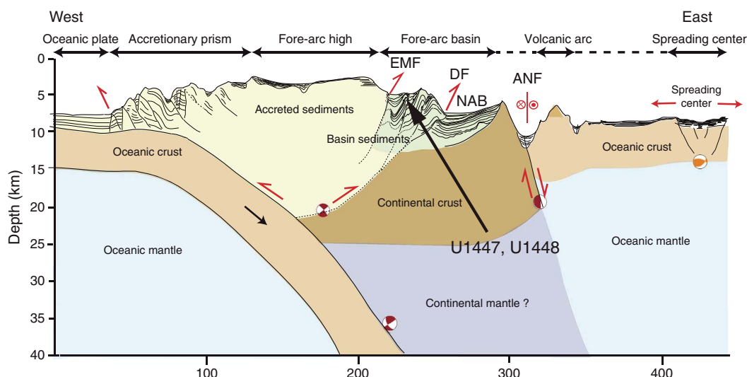
Figure F7. Summary sketch after Singh et al. (2013) showing the subduction zone through the back-arc basin to ~40 km depth. EMF = Eastern Margin fault, DF = Diligent fault, NAB = Nicobar Andaman Basin, ANF = Andaman-Nicobar fault.
