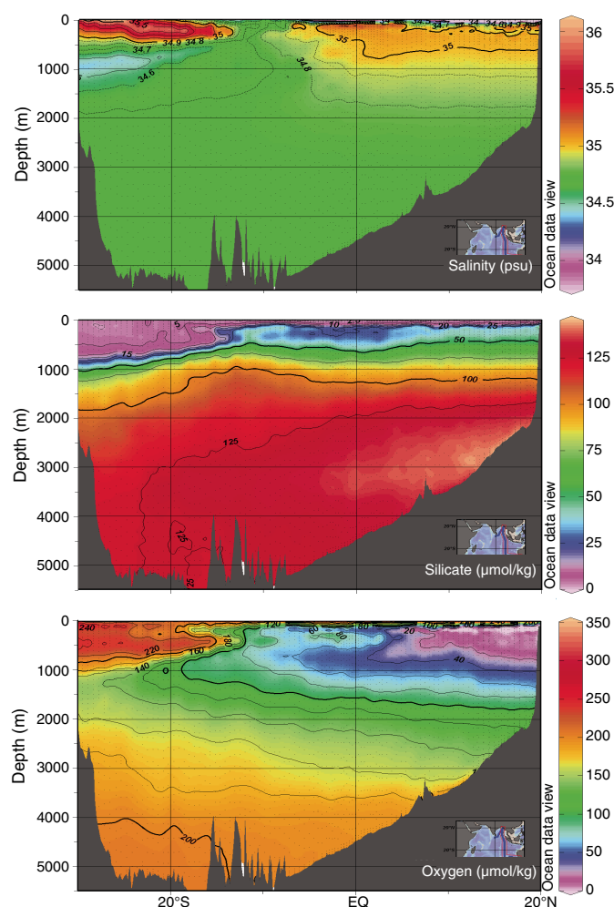
Figure F13. Salinity, silicate, and oxygen from eastern Indian Ocean WOCE meridional Transect I09, eastern Indian Ocean (from eWOCE Gallery, http://www.ewoce.org/gallery [Schlitzer, 2000]).
