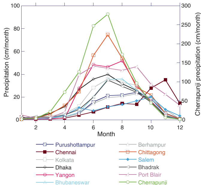
Figure F9. Monthly precipitation data for 1948–2011 (as available) for locations with drainage into the Bay of Bengal. Cherrapunji precipitation is scaled separately. Data from World Meteorological Organization ( http://climexp.knmi.nl ).
