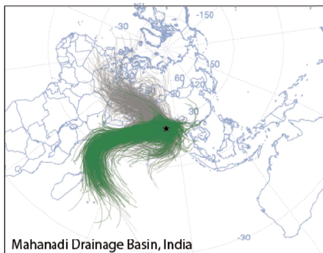
Figure F5. Ten-day National Oceanic and Atmospheric Administration HYSPLIT backtracks (2007–2011). Green indicates rain-bearing air trajectories. Rain-bearing trajectories over India are dominated by summer season (southwest) winds, whereas both winter (northerly) and summer (southerly) air masses carry precipitation to the monsoonal region of eastern China. This is consistent with World Meteorological Organization rainfall records indicating that June, July, and August rainfall only accounts for 50% of the total annual rainfall in eastern China. The Bay of Bengal location isolates summer season dynamics.
