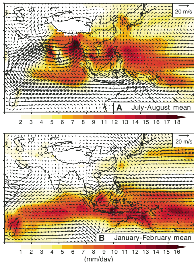
Figure F3. Climatological (A) July–August and (B) January–February mean precipitation rates (shading in mm/day) and 925 hPa wind vectors (arrows). Precipitation and wind climatology are derived from CMAP (Xie and Arkin, 1997) (1979–2000) and NCEP/NCAR reanalysis (1951–2000), respectively.
