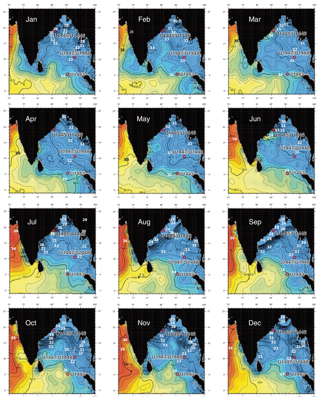
Figure F4. World Ocean Atlas Monthly Mean Salinity for 1955–2006 (Antonov et al., 2010). Areas drilled in the Andaman Sea (Sites U1447 and U1448), Mahanadi basin, northern Bay of Bengal (Sites U1445 and U1446), and Ninetyeast Ridge (Site U1443) are shown.
