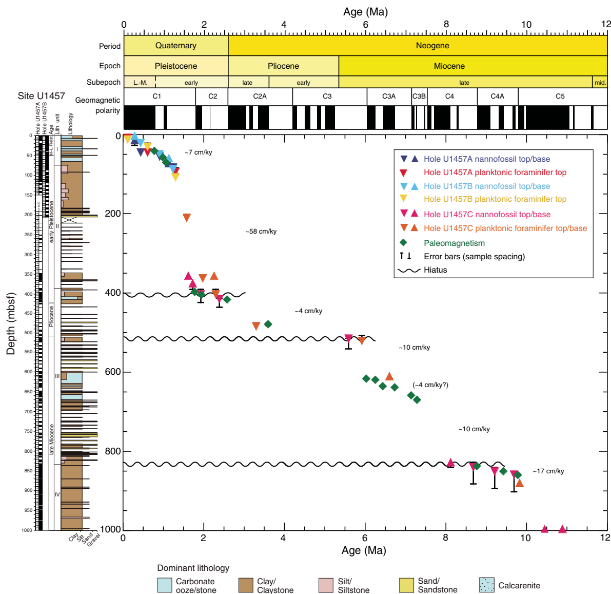
Figure F12. Age-depth model for Site U1457 created by synthesizing nanofossil and foraminifer bioevents with magnetic chron assignments. Note that the age depth model only extends to 1000 mbsf due to a long hiatus near the base of the cored section, with the top of lithologic Unit V at ~1062 mbsf dated to the early Paleocene. Top = last occurrence, base = first occurrence.
