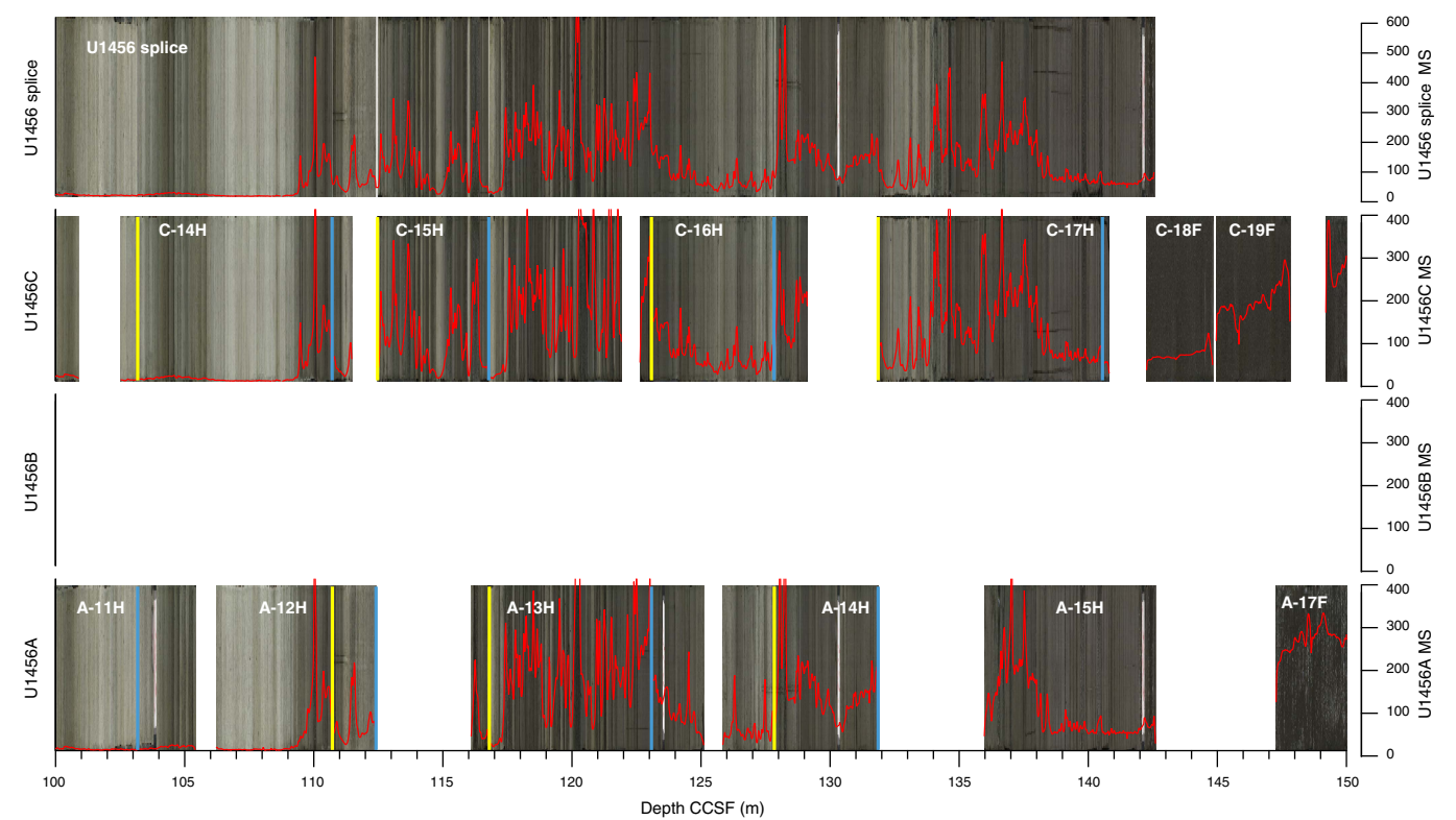
Figure F24. Core images and MS for 100–150 m CCSF in Holes U1456A and U1456C, with the assembled splice at the top. Yellow lines = beginning of a sediment interval included in the splice, blue lines = the base of the splice interval. The splice ends at the base of Core U1456A-15H. Splice intervals can be found in Table T14.
