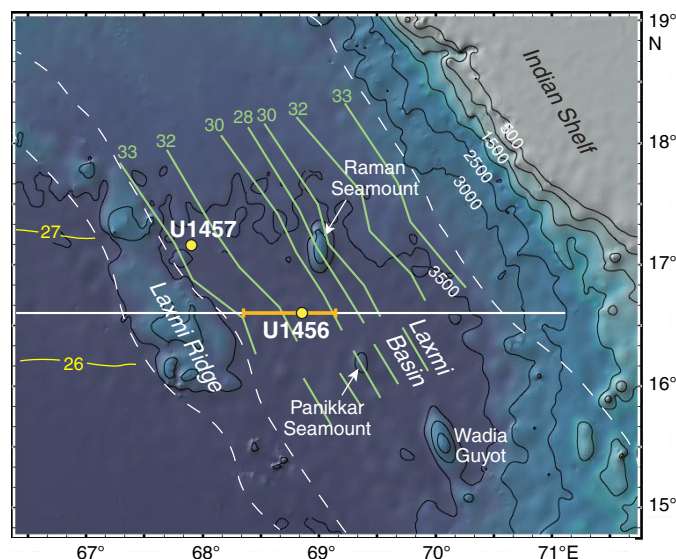
Figure F2. Shaded bathymetric map of the region around Laxmi Basin showing the location of Site U1456 in relation to other major bathymetric features, especially Laxmi Ridge. White dashed lines = various possible locations of the continent/ocean boundary depending upon whether the crust in Laxmi Basin has continental or oceanic affinity. White line = seismic profile Line W06; orange bar = portion of the profile illustrated in Figure F3. Magnetic anomalies (yellow lines) in the Arabian Basin are from Miles et al. (1998), whereas those in Laxmi Basin (green lines) are from Bhattacharya et al. (1994). Bathymetric data from GeoMapApp (Ryan et al., 2009).
