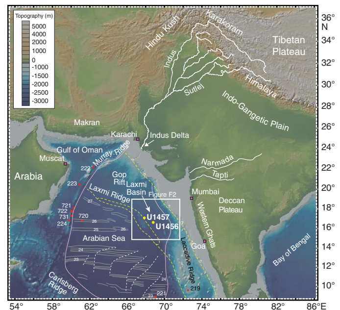
Figure F1. Shaded bathymetric map of the Arabian Sea and the surrounding landmasses from GeoMapApp (Ryan et al., 2009). Yellow circles = sites drilled during this expedition. Red stars = earlier scientific drilling sites. Pink line = approximate extent of the fan after Kolla and Coumes (1987). Yellow dashed lines/question marks = speculated locations of the continent/ocean boundary depending on whether Laxmi Basin is floored by oceanic or continental crust. Gray lines with numbers = magnetic anomalies from Royer et al. (2002). Box shows location of detailed map in Figure F2. Numbers indicate Chron numbers.
