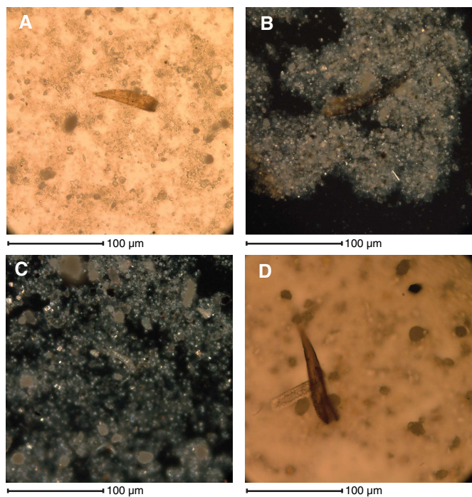
Figure F36. Meiofaunal organisms observed at 500× magnification, Hole U1456B. A. 2H-4, 130–140 cm (PL). B. 4H-1, 130–140 cm (dark field). C. D. 4H-6, 130–140 cm (C: dark field, D: PL).
