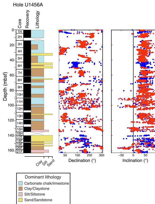
Figure F37. Results of pass-through magnetometer measurements of archive halves, Hole U1456A. Declination and inclination measured after demagnetization at 25 mT. Blue symbols = data as measured, red symbols = edited data.
