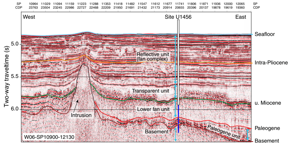
Figure F3. Seismic reflection profile Line W06 with location of Site U1456 and main seismically defined horizons described in text. Purple bar shows proposed penetration at Site U1456; white box shows actual penetration. SP = shotpoint, CDP = common depth point.
