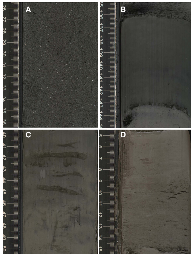
Figure F13. Dominant lithologies in Unit II, Hole U1456A. A. Sand with silt (56F-1, 26–36 cm). B. Clay (20F-2, 135–145 cm). C. Nannofossil-rich clay (15H-3, 40–50 cm). D. Nannofossil-rich clay with silt (22F-1, 5–15 cm).
