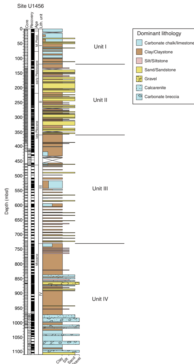
Figure F6. Synthesis lithostratigraphic log for Site U1456 showing combined recovery in Holes U1456A–U1456E.
