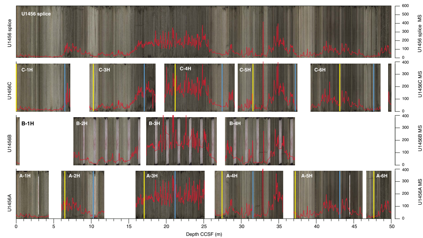
Figure F22. Core images and magnetic susceptibility (MS) for 0–50 m CCSF in Holes U1456A–U1456C, with the assembled splice at the top. Yellow lines = beginning of a sediment interval included in the splice, blue lines = the base of the splice interval. Despite heavy sampling, the records from Hole U1456B can be correlated to Holes U1456A and U1456C. Splice intervals can be found in Table T14.
