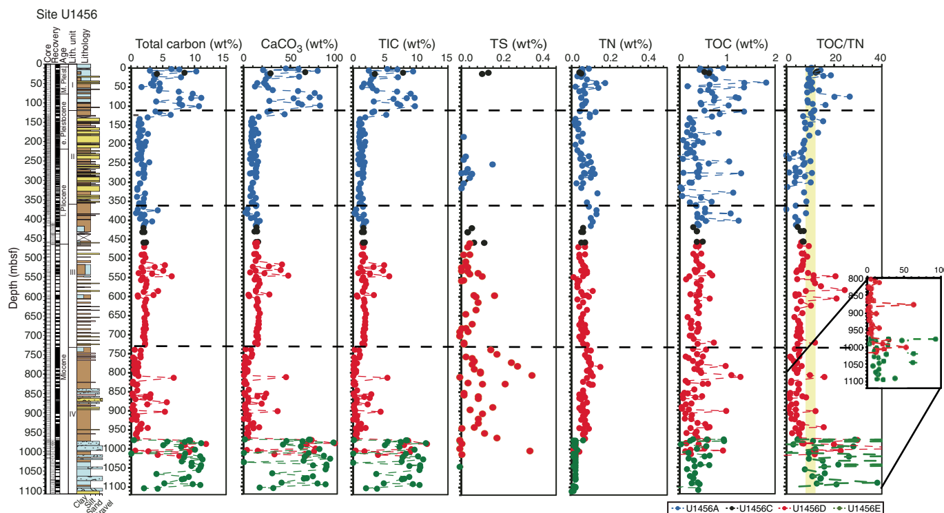
Figure F28. Total carbon, \text{CaCO}_3 , TIC, total sulfur, total nitrogen, TOC, and TOC/TN, Site U1456. Yellow line = boundary between the contribution of predominantly marine organic carbon (<8) and terrestrial organic carbon (>12) (Müller and Mathesius, 1999). Dashed lines = lithologic unit boundaries.
