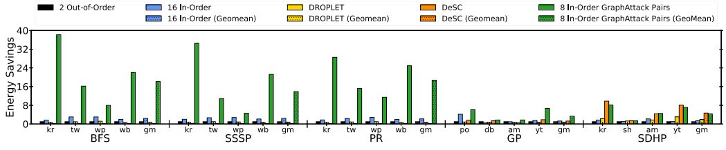
Fig. 9. Energy efficiency comparisons between 2 parallel OoO cores, 16 parallel InO cores, DROPLET prefetching (2 OoO), DeSC (1 OoO pair), and 8 GraphAttack (InO) pairs (ratios that equalize for area). With hardware-efficient innovations, GraphAttack achieves significant energy efficiency gains over all other techniques.
