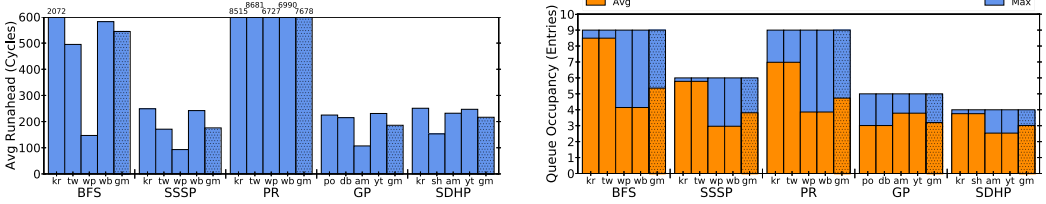
Fig. 7. LHS: GraphAttack achieves significant Producer runahead, with average runahead distances far greater than the DRAM latency of 200 cycles (100 ns). RHS: GraphAttack requires very small (<10 entries) AABs.
