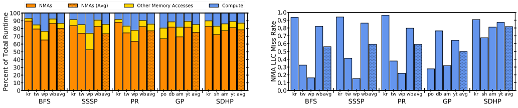
Fig. 3. LHS: Runtime analysis of an InO core running benchmark graph/sparse applications and inputs demonstrates that NMAs can significantly increase runtime if not effectively mitigated. RHS: NMAs have severe LLC miss rates, often times >50\% .
