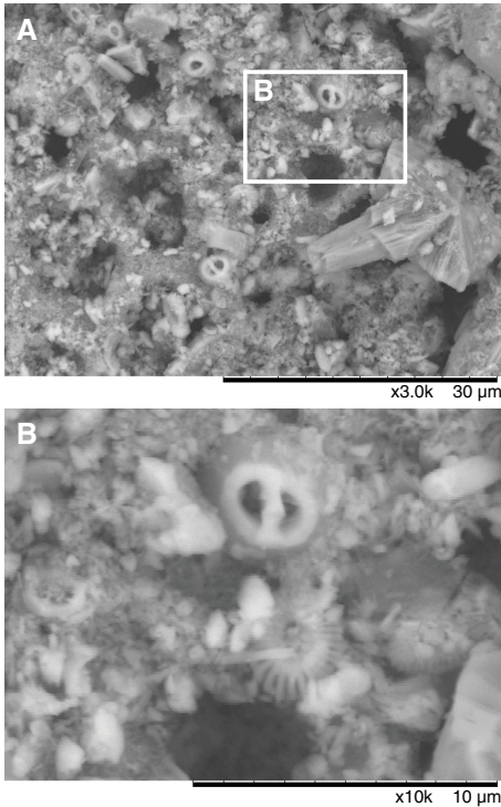
Figure F5. SEM photomicrograph, mudline (356-U1458A-1H-1). A. Recent–Pleistocene placoliths and calcareous sponge spicules. B. Close-up (see inset in A) of Gephyrocapsa oceanica (top) and Emiliania huxleyi (center and right).
