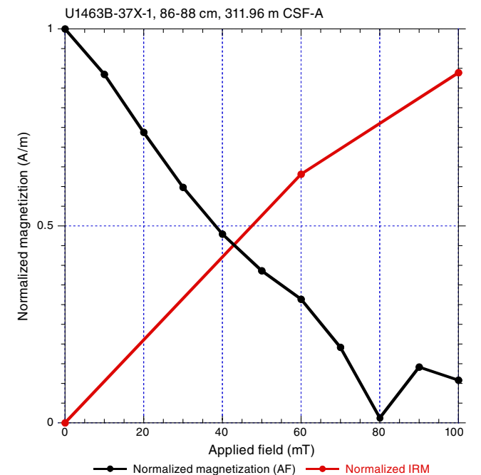
Figure F25. IRM curve and corresponding AF demagnetization trend, Sample 356-U1463B-37X-1, 86–88 cm (311.96 m CSF-A).
