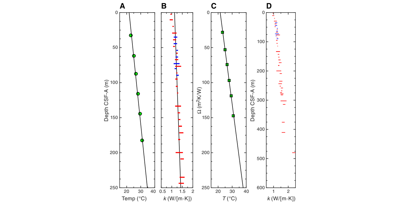
Figure F32. A. In situ temperatures measured with APCT-3, Hole U1463C. B. Thermal conductivity ( k ) measured on Hole U1463B (red) and U1463C (blue) cores and used in heat flow calculation. C. Thermal resistance ( \Omega ) vs. temperature ( T ) (Bullard plot). D. Thermal conductivities as measured throughout entire cored interval. In B and D, only data with standard deviations <0.1 W/(m·K) are shown. Symbol width indicates standard deviation of each measurement.
