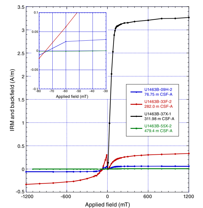
Figure F24. IRM acquisition curves for four discrete samples from Hole U1463B and their respective backfield curves. Inset shows enlarged view of negative x-axis, showing the coercivity of remanence estimation for each sample.
