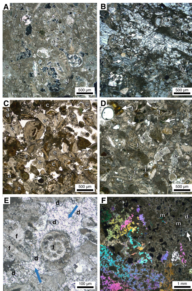
Figure F7. Representative thin section photomicrographs, Hole U1463B. A. Unit II: skeletal packstone with abundant medium sand-sized benthic and planktonic foraminifers (f) and few echinoderm fragments (e) (9H-1); XPL. B. Subunit IIIa: skeletal packstone with abundant planktonic and benthic foraminifers (f) and pore space filled by large bluish to grayish single celestite crystals (arrows) (31F-1); XPL. C. Subunit IIIb: foraminiferal grainstone with abundant benthic foraminifers Amphistegina (a) and Cibicidoides (c) and rare echinoderm fragments (e); planktonic foraminifers are rare; note abundant greenish glauconitic and brownish iron oxide staining and high interparticle porosity (46X-3). D. Unit IV: foraminiferal packstone with abundant LBFs and rare planktonic foraminifers (f), common echinoderm fragments (e), and abundant glauconitization (white arrows) as well as brownish iron oxide staining (47X-3). E. Unit V: skeletal packstone with abundant small benthic foraminifers (f) and echinoderm fragments, and euhedral dolomite (d); pore space is cemented mainly with calcite and partly with celestite (blue arrows) (54X-CC). F. Unit V: dolomitic limestone with intensive anhydrite (a) replacement, micrite (m), dolomite (d) and celestite (white arrow) (55X-6).
