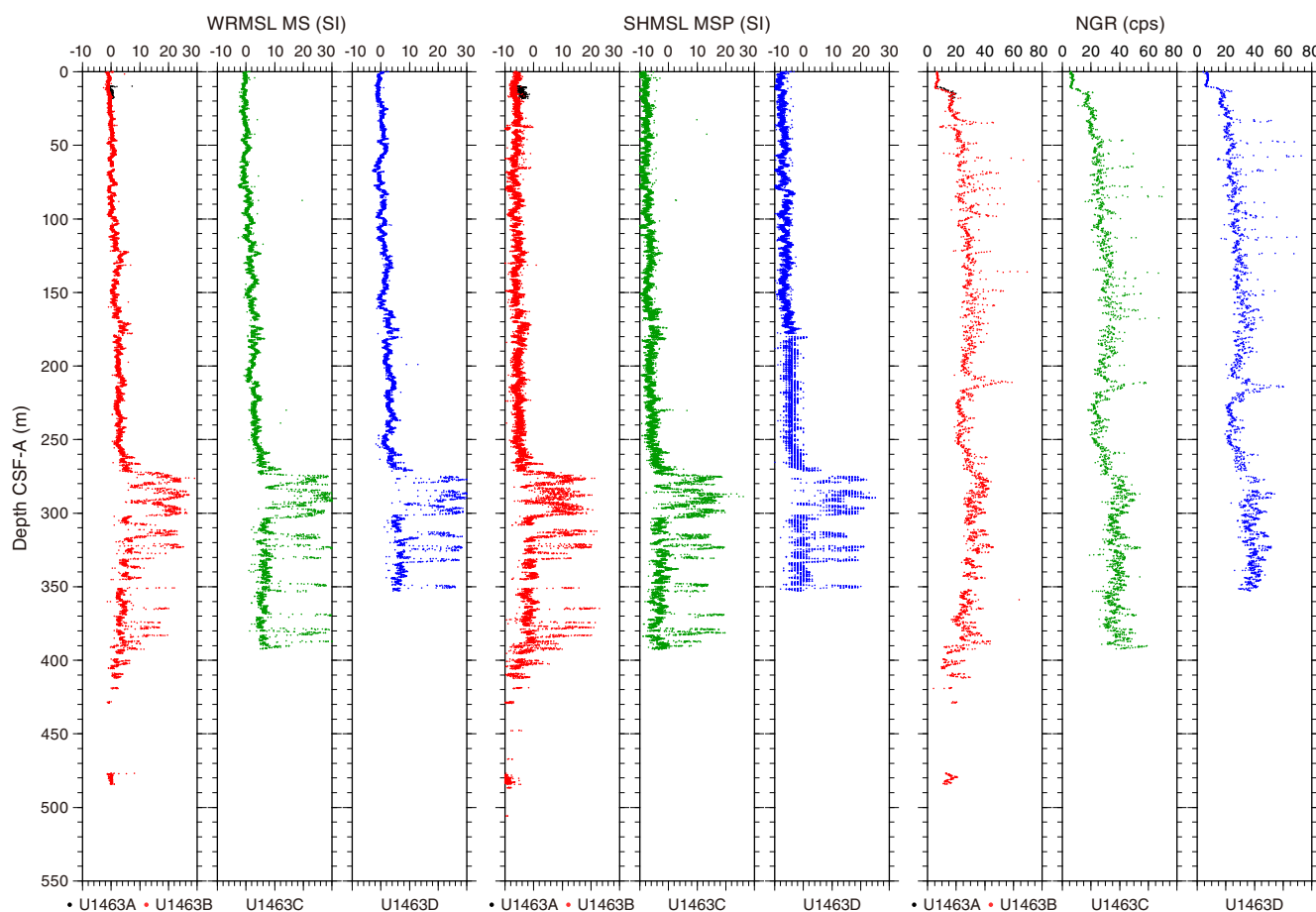
Figure F27. WRMSL MS, SHMSL point magnetic susceptibility (MSP), and NGR results, Site U1463. SHMSL data are raw MS from Hole U1463A and drift-corrected MS from all the other holes.
