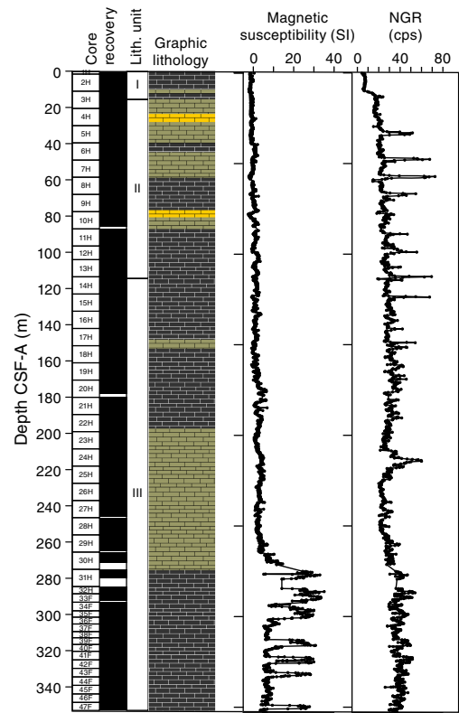
Figure F42. Hole U1463D summary showing core recovery, graphic lithology, and lithostratigraphic units, plotted against MS and NGR. No biostratigraphy or magnetostratigraphy was performed on this hole. See Figure F7 in the Expedition 356 methods chapter (Gallagher et al., 2017a) for lithology key.
