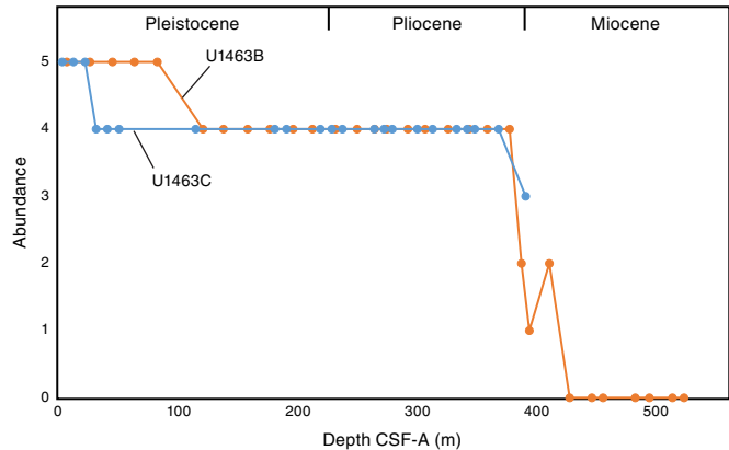
Figure F12. Planktonic foraminiferal abundance, Site U1463. 0 = barren, 1 = very rare, 2 = rare, 3 = few, 4 = common, 5 = abundant (see Biostratigraphy and micropaleontology in the Expedition 356 methods chapter [Gallagher et al., 2017a] for definitions).
