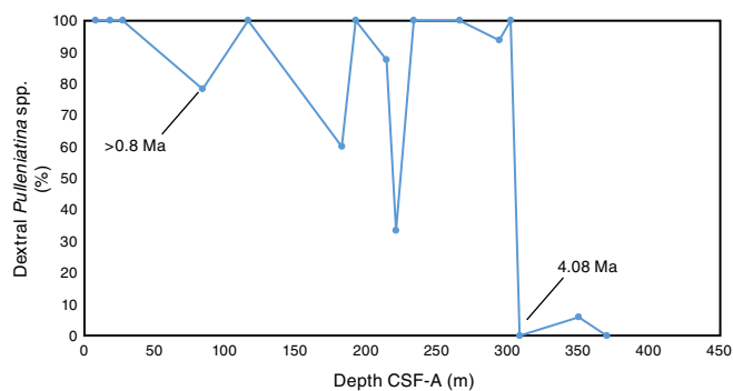
Figure F14. Variation in the coiling direction of planktonic foraminiferal genus Pulleniatina , Site U1463. Samples to 265 m CSF-A are P. obliquiloculata , samples deeper than 308 m CSF-A are P. primalis , and samples in between are a mixture of both species. Note that specimens of P. finalis were included with P. obliquiloculata (Kennett and Srinivasan, 1983). Ages are based on Saito (1976) and Pearson (1995) and recalibrated following Wade et al. (2011).
