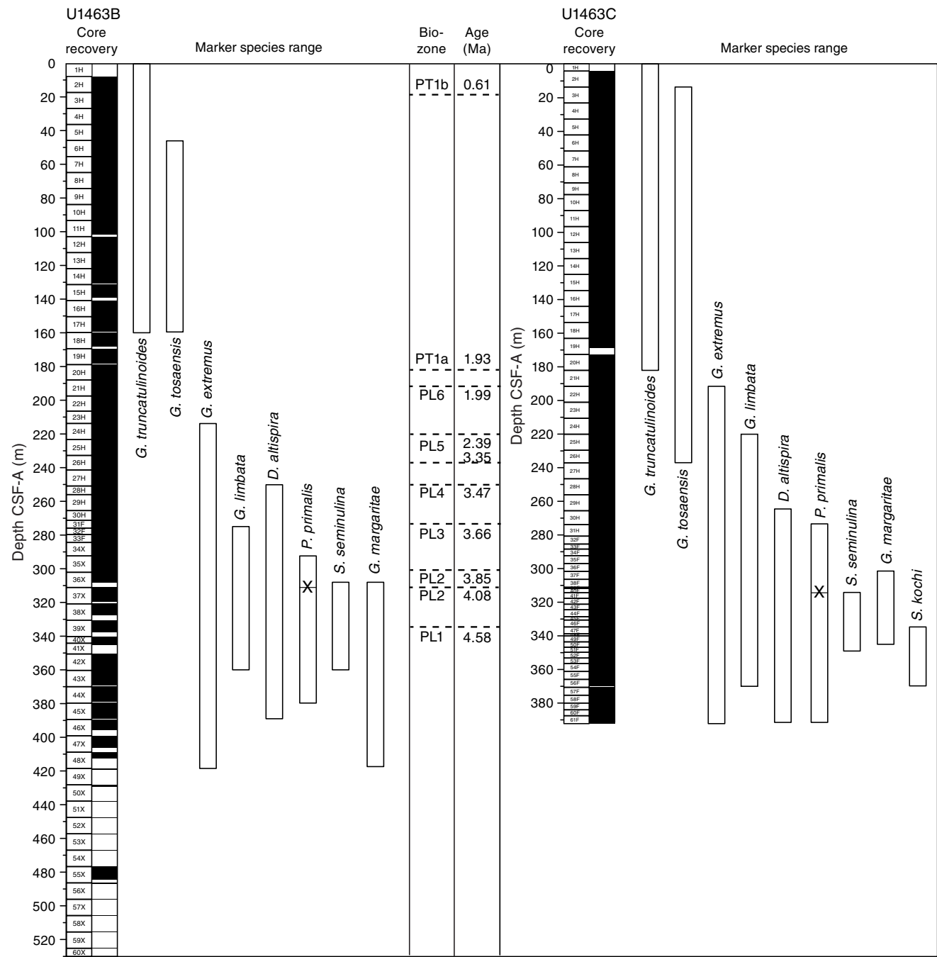
Figure F13. Planktonic foraminiferal marker species ranges, Holes U1463B and U1463C. Ages are based on published values (Gradstein et al., 2012).
