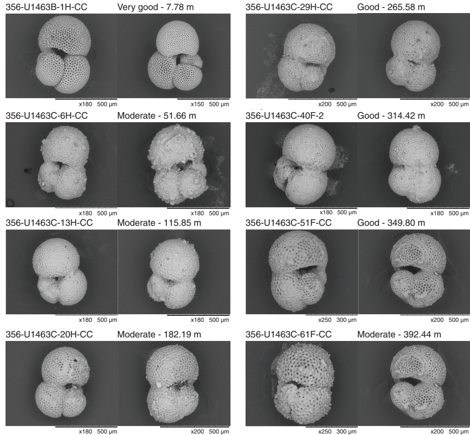
Figure F12. Planktonic foraminiferal abundance, Site U1463. 0 = barren, 1 = very rare, 2 = rare, 3 = few, 4 = common, 5 = abundant (see Biostratigraphy and micropaleontology in the Expedition 356 methods chapter [Gallagher et al., 2017a] for definitions).
