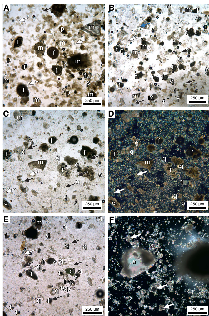
Figure F6. Representative smear slide photomicrographs of units, Hole U1463B. A. Unit I: sediment rich in small peloids (p) with abundant miliolid benthic and planktonic foraminifers (f), well-preserved mollusk shell fragments (m), a single siliceous sponge spicule (s); note very fine-grained authigenic glauconite (black arrow) and mica (white arrows) (7H-2, 71 cm). B. Unit II: dominant planktonic and benthic foraminifers (f) with fewer well-preserved shell fragments (m); quartz (q), ascidian spicules (blue arrow), and mica (white arrow) are common accessory to minor components; note small authigenic glauconite grains, often in aggregates with clay-sized sediment (black arrows) (3H-2, 71 cm). C. Subunit IIIa: benthic and planktonic foraminifers (f) and shell fragments (m) in a coarse (fine silt sized) matrix; accessory echinoderm spine (e) and sponge spicule (s) fragments; note common quartz (q), mica (white arrows), and accessory authigenic glauconite (black arrows) (17H-2, 71 cm). D. Cross-polarized light (XPL) image of C, illustrating silt-sized quartz (q) in a carbonate matrix with sand-sized bioclasts. E. Subunit IIIb: benthic and planktonic foraminifers (f) with poorly preserved shell fragments (m); note increased siliciclastic components dominated by quartz (q) and feldspar (fsp), with mica (white arrow) and rare chlorite (cl); authigenic glauconite and glauconitized foraminifers are also common (black arrows) (40X-2, 71 cm). F. Unit V: large anhydrite (a) grains in a dolomite matrix (white arrows) (59X-CC); XPL.
