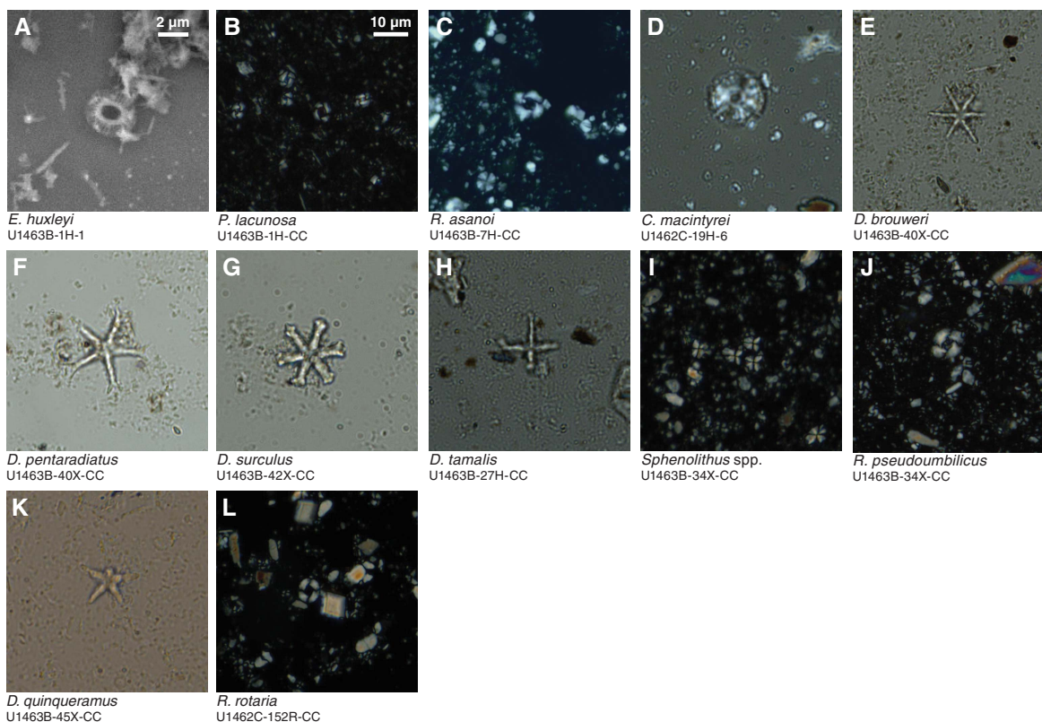
Figure F10. SEM and plane-polarized light (PPL) photomicrographs of calcareous nannofossils, Site U1463. A. Emiliania huxleyi . B. Pseudoemiliania lacunosa . C. Reticulofenestra asanoi . D. Calcidiscus macintyre . E. Discoaster brouweri . F. Discoaster pentaradiatus . G. Discoaster surculus . H. Discoaster tamalis . I. Sphenolithus spp. J. Reticulofenestra pseudoumbilicus . K. Discoaster quinquaramus . L. Reticulofenestra rotaria .
