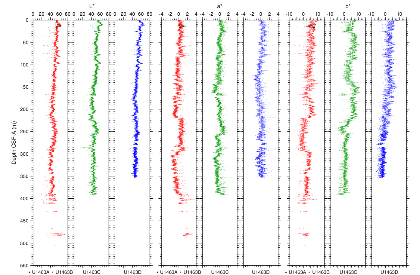
Figure F31. Reflectance spectroscopy and colorimetry ( L^* , a^* , and b^* ), Site U1463. Hole U1463C data were corrected by rescanning affected core sections (see text for details).
