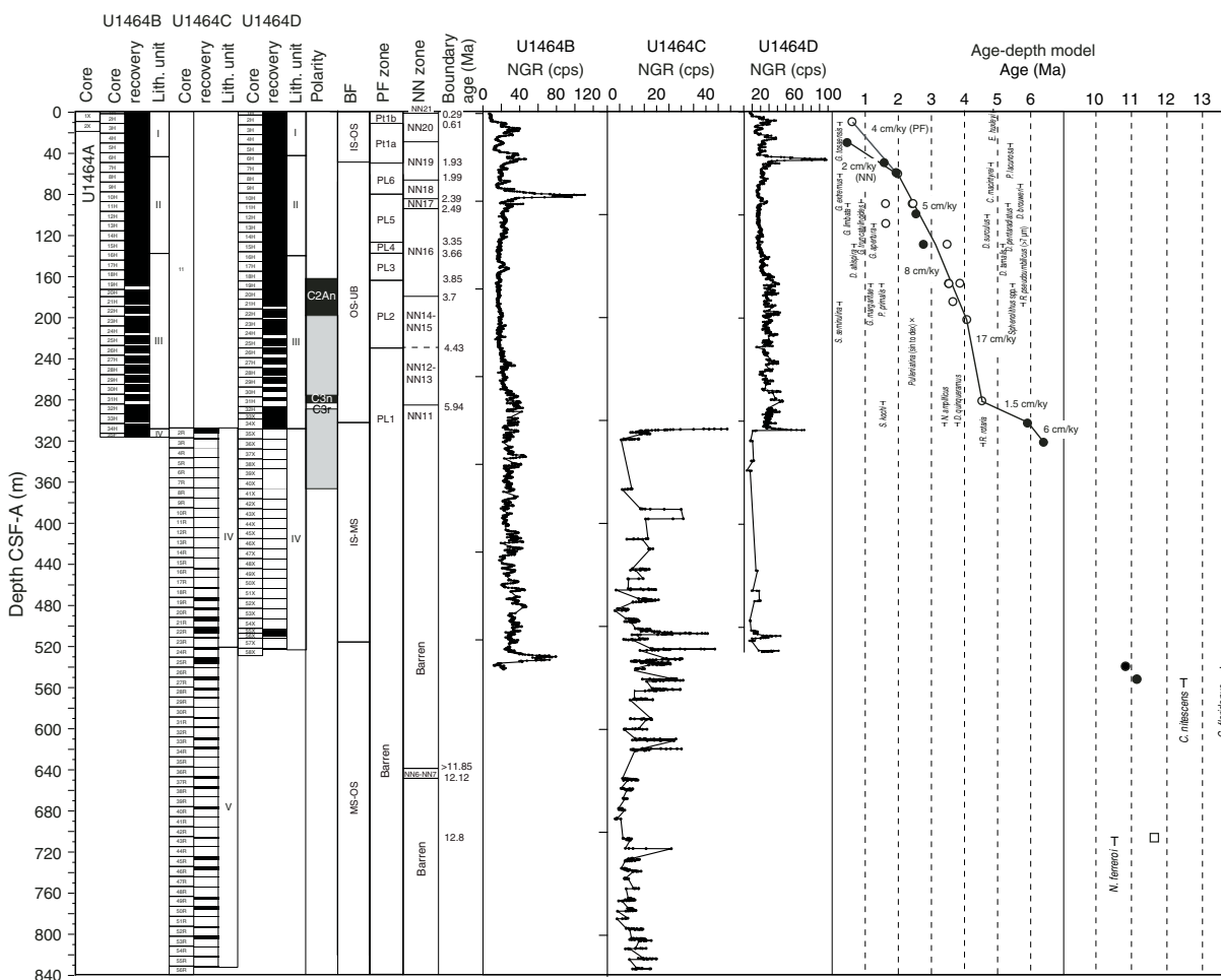
Figure F40. Site U1464 summary showing core recovery, graphic lithology, lithostratigraphic units, age, magnetostratigraphy, biostratigraphy, and NGR. Magnetic polarity is shown in black and white, gray intervals = uncertainty in the data (see Paleomagnetism ). Biostratigraphic zone boundary ages are shown. Age-depth model was produced from biostratigraphic datums only (see Biostratigraphy and micropaleontology ) and assumes a linear sedimentation rate between datums (solid circles = calcareous nannofossils, open circle = planktonic foraminifers, open square = benthic foraminifer). Sedimentation rates are calculated separately for calcareous nannofossils and planktonic foraminifers where the datums diverge. Note the break in horizontal scale for the age-depth model. Benthic foraminiferal assemblages were smoothed to generate this synthesis, resulting in slight differences from data presented in hole summaries.
