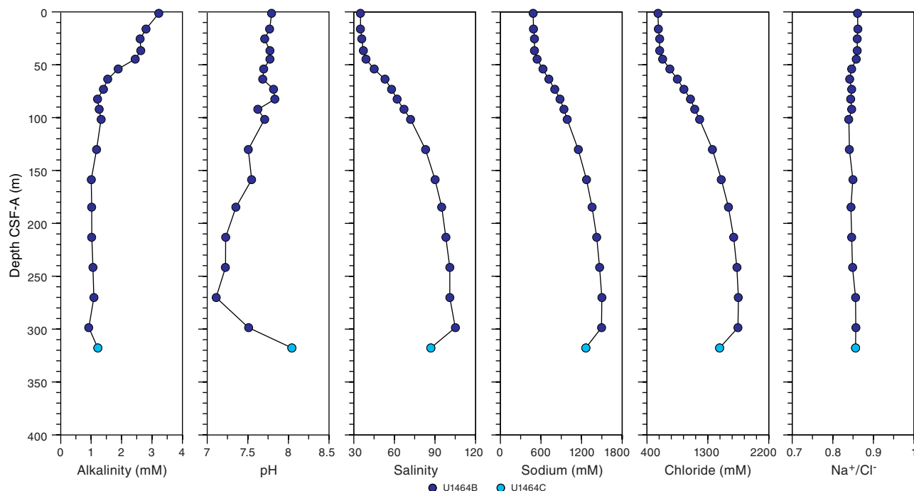
Figure F20. Alkalinity, pH, salinity, sodium, chloride, and sodium to chloride ratio, Site U1464.
