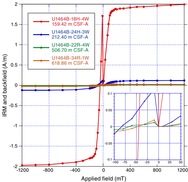
Figure F25. IRM acquisition curves for 4 discrete samples from Hole U1464B and their respective backfield curves. Inset shows an enlargement of back-field IRM curves, identifying coercivity of remanence values for each sample.
