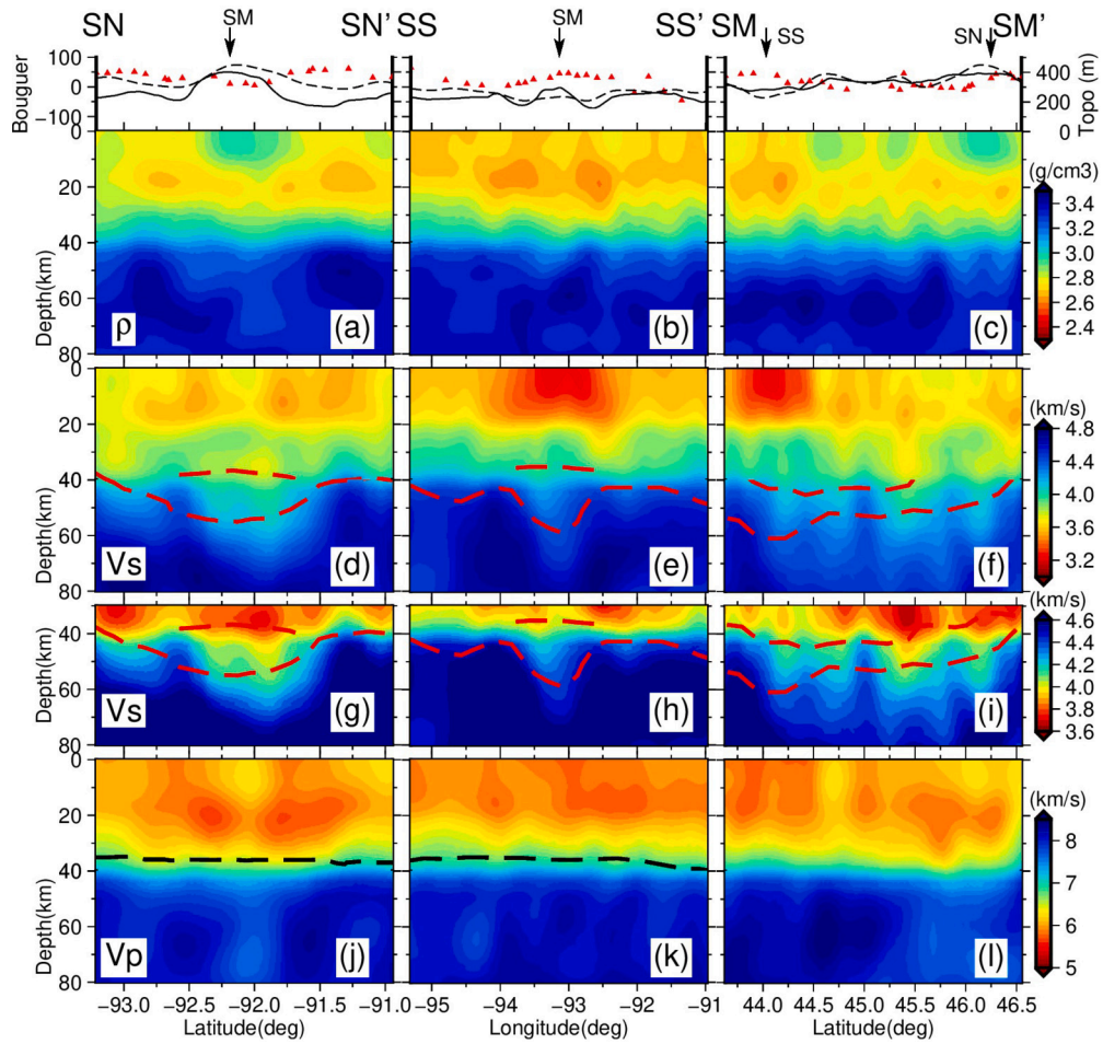
Fig. 7. Vertical cross-sections of absolute density (first row), Vs (second row) and Vp (fourth row) values for the final model, AKinv , along the SN-SN' (first column), SS-SS' (second column), and SM-SM' (third column) profiles. In the top panel, the corresponding observed and synthetic (calculated from the final density model) Bouguer anomalies along the three profiles are shown as black solid and dashed lines. The red triangles indicate the dense array along each profile with their vertical coordinates showing the variation of topography. The third row (Panels g, h, and i) are zoom-in of the Vs images in the second row around the Moho. The dashed red lines overlain on the Vs models represent the interfaces obtained from P-to-S receiver functions (Zhang et al., 2016), while the dashed black line overlain on the Vp model denotes the interfaces obtained from S-to-P receiver functions (Chichester et al., 2018). The cross points of the profiles are indicated by black arrows on top of the figure. The corresponding color bars are shown to the right of each row.
