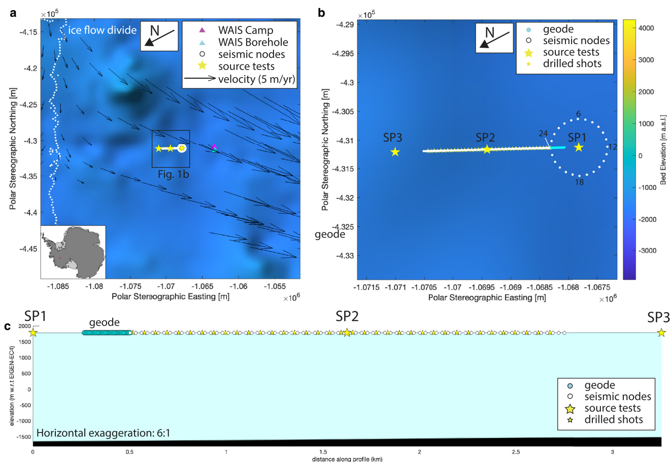
Figure 1. Location maps for surface seismic source testing near West Antarctic Ice Sheet (WAIS) Divide. (a) Map showing location of the seismic test site ~5-km northeast of WAIS Divide Camp. Bed elevation is from BedMachine v3 (Morlighem and others, 2020). Arrows show the ice flow measured near WAIS Divide (Conway and Rasmussen, 2009). Dashed white lines show the location of the ice flow divide. Ice southwest of the divide flows toward the Ross Sea, and ice northeast of the divide flows toward the Amundsen Sea. (b) Zoomed-in map of the seismic line and locations of sources and receivers used for shot testing. Maps were plotted in MATLAB using Antarctic Mapping Tools (Greene and others, 2017). Numbers indicate trace or node numbers for nodes in the circle. These numbers are used in Figures 3–5 for numbering the node circle traces. (c) Horizontally exaggerated (6:1) cross section along the line from shotpoint (SP) 1 to 3 showing locations of sources and receivers and bed depths from BedMachine v3 (Morlighem and others, 2020).
