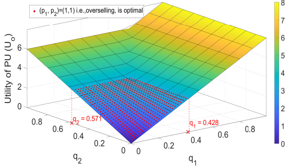
Fig. 3. Utility of the PU ( U_0 ) vs. communication uncertainties of the SUs
