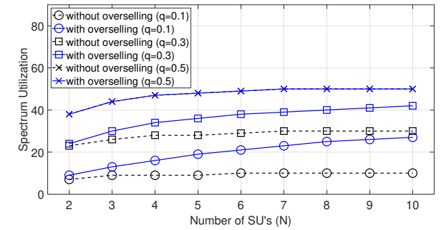
(c) Spectrum Utilization with and without overselling vs. N
