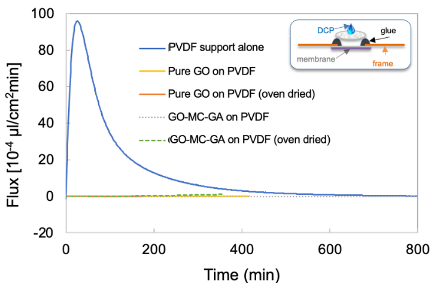
Figure 6. Diethyl chlorophosphate (DCP) permeation rates through GO (3 \mu\text{m} ) and GO-MC-GA (10 \mu\text{m} ) films under conditions of vapor-only contact. All films are supported on a porous PVDF filter during testing, which allows rapid DCP vapor permeation when used alone as a positive control. All films studied here are effective DCP vapor barriers.
