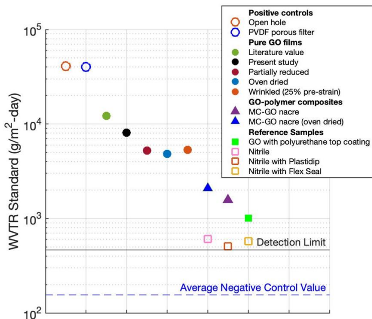
Figure 8. Summary of experimental Water Vapor Transmission Rates (WVTR, or breathability) obtained with the static permeation method for various pure GO films and GO-polymer composites. Data are for 37C and \Delta RH = 90\% . Positive control samples are uncovered top holes or top holes covered by a porous PVDF membrane (open circles), and negative control samples are measured with a metal foil barrier. The lower detection limit is set at 3x the negative control value. Literature data on GO film WVTR using a similar technique are from Spitz et al.[19]. Results for pure GO films and GO composites are shown as colored circles and triangles, respectively. Glove-derived nitrile substrate barely exceeds the detection limits. The standard errors are about +/- 5% of the mean for samples well above the detection limit.
