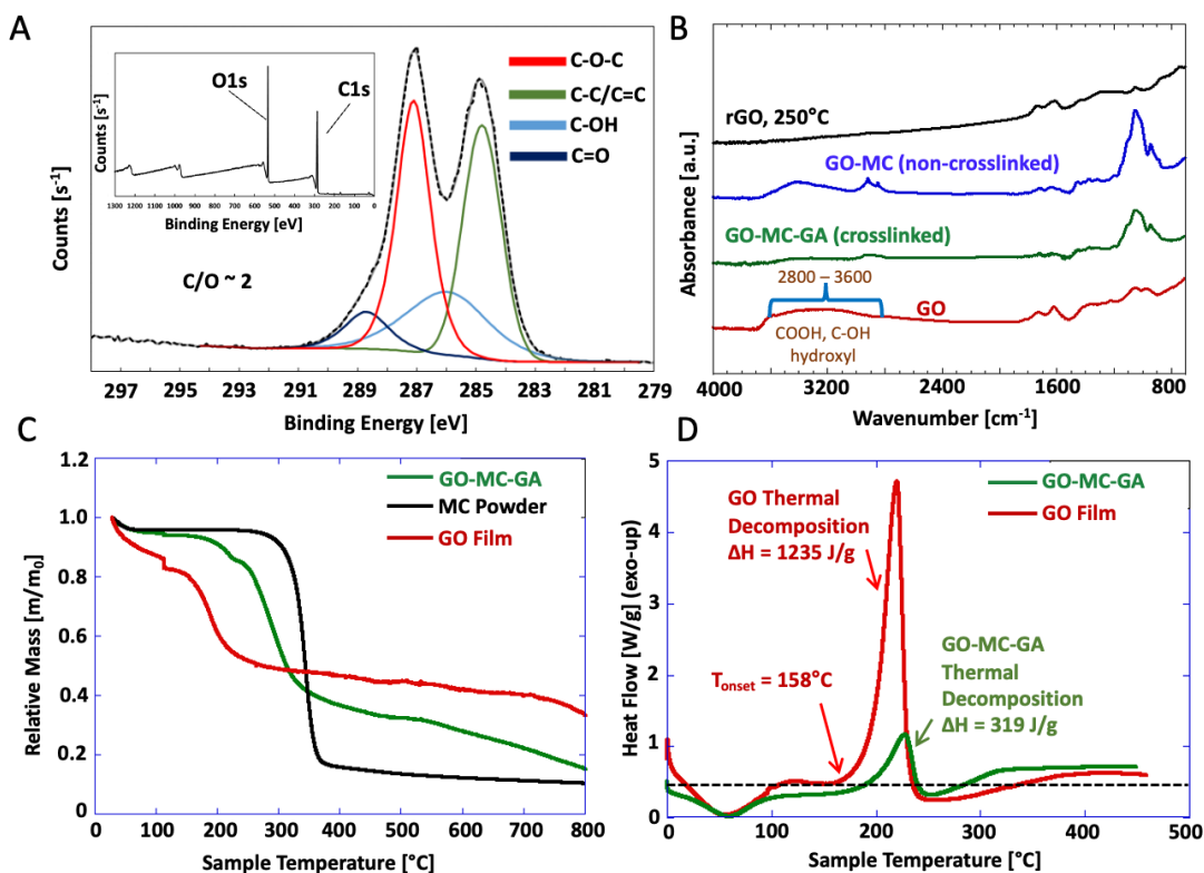
Fig. 4. Spectroscopic and thermal characterization of pure GO and composite films. A: XPS characterization of GO films: C1s high-resolution spectrum with peak deconvolution and survey spectrum inset. B: FTIR spectra of GO films, crosslinked (GO-MC-GA) and non-crosslinked (GO-MC) films, and rGO films (thermally reduced) as a reference. C: Thermal gravimetric analysis traces showing the decomposition behavior of the composite compared to pure GO and MC. D: Differential scanning calorimetry traces showing the characteristic exotherm of GO thermal decomposition in both the pure GO and GO-MC-GA composite films.
