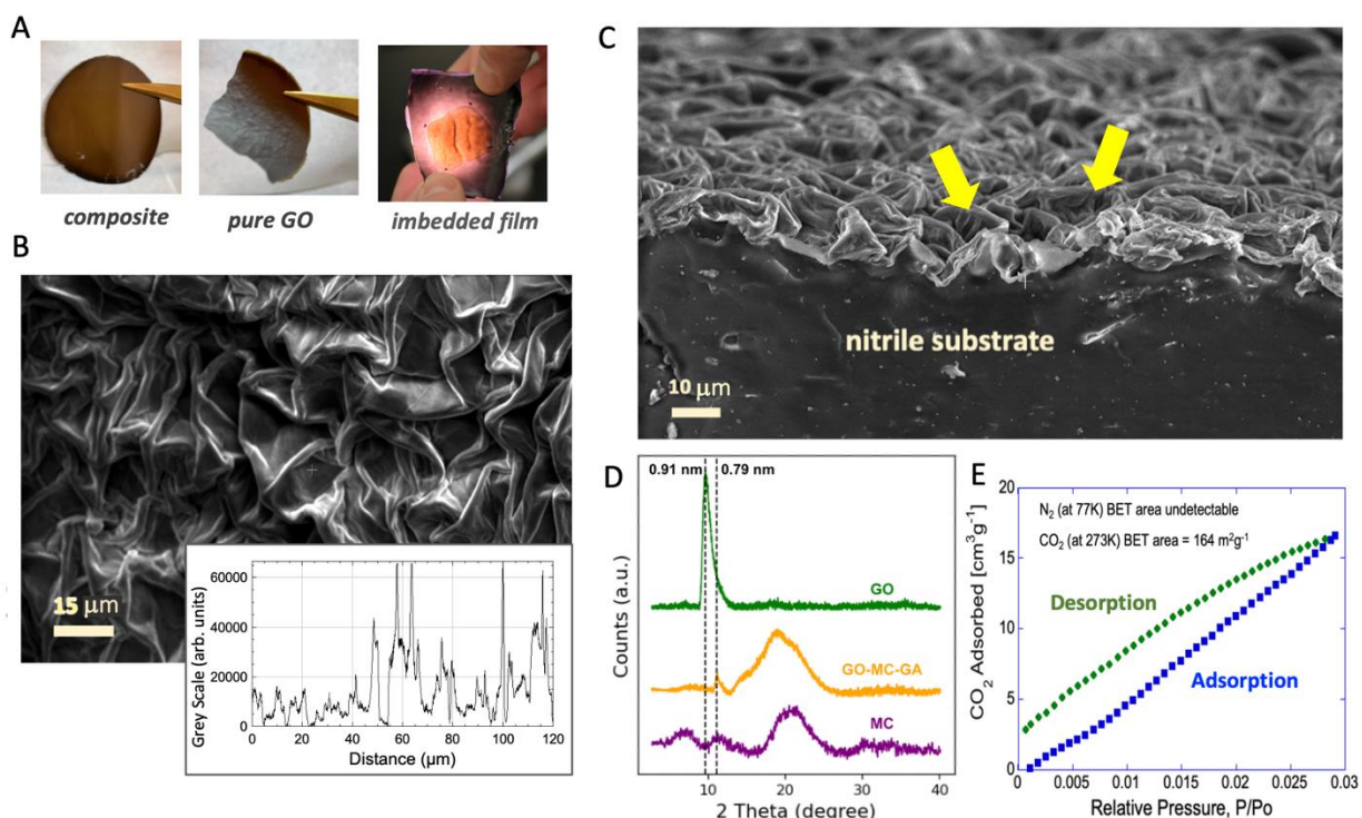
Figure 3. Structural characterization of graphene-based films. A: Photos of pure, composite and imbedded GO films. The composite films are noticeably less flexible (have higher bending stiffness) than pure GO films. B: Textured GO films fabricated by the mechanical stretch method at 66% isotropic pre-stretch. Inset is a grey-scale line profile showing a \sim 10 \mu\text{m} wavelength scale for the primary out-of-plane textural features. C: Cross-sectional view of a textured GO film (66% pre-stretch) after freeze fracture using tilt-stage SEM (yellow arrows show example complex, 3D cavities). D: XRD spectra for pure GO, the composite, and pure methyl cellulose, showing the interlayer spacing in pure GO films (0.91 nm), and its absence in the GO-MC-GA composite, indicating the loss of nanosheet when the polymer is introduced. E: Vapor adsorption isotherms and computed internal surface areas for the GO-MC-GA film.
