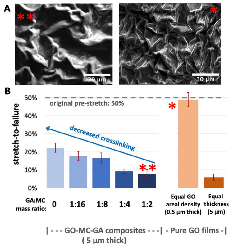
Figure 12. Role of binder, crosslinking and film thickness in the stretchability of textured graphene-based films. A: Textures of pure GO films (right) and GO-MC-GA composite films (left), showing different length scales of the textural features. B: Stretchability results shown as stretch-to-failure \Delta L/L_0 values. B-left: Reducing the concentration of the glutaraldehyde (GA) crosslinking reagent improves stretchability of the composite films. B-right: thickness is a major variable determining the \Delta L/L_0 stretch-to-fail value.
