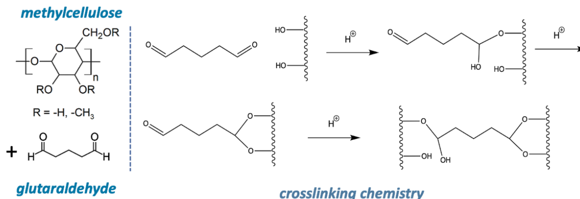
Figure 2. Molecular structures and crosslinking mechanism relevant to the GO-MC-GA composite coatings. Glutaraldehyde is reported to be effective as a crosslinker of hydroxyl groups[45, 46], and the mechanism is initiated by nucleophilic attack by hydroxyl oxygen on the carbonyl carbons, resulting in glutaraldehyde fixation to polymer and/or GO by ether linkages.
