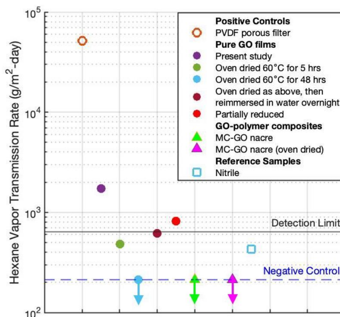
Figure 5. Experimental hexane vapor transmission rates of pure GO films and GO-MC-GA composite films measured by a gravimetric permeation method. The Y-axis shows the flux from a saturated vapor from a liquid hexane source at 20 C to the room air above the film. Test films are supported on a porous PVDF membrane of negligible diffusional resistance (see positive control for PVDF filter). Negative control samples are measured with a metal foil barrier. The lower detection limit is set at 3x the negative control value. Dry GO films and the GO-MC-GA composite are at or below the negative control value. The standard deviations are about +/- 5% of the mean for samples far above the detection limit.
