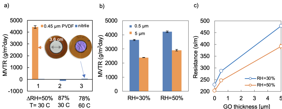
Figure 9. Water vapor transport rates (WVTR) and derived resistances measured by a dynamic flow technique for various GO films and average humidity values. Error bars from n \geq 2 . Most data are duplicate tests performed in two consecutive days. A: Reference samples of nitrile glove elastomer, and the porous PVDF filter support; B-C: pure GO films of 0.5 μm and 5 μm thicknesses (on 0.45 μm pore size PVDF support) under a relative humidity gradient of \Delta RH=50\% at 30 °C. The RH=30% and RH=50% labels in panel B-C indicate the average RH across the film.
