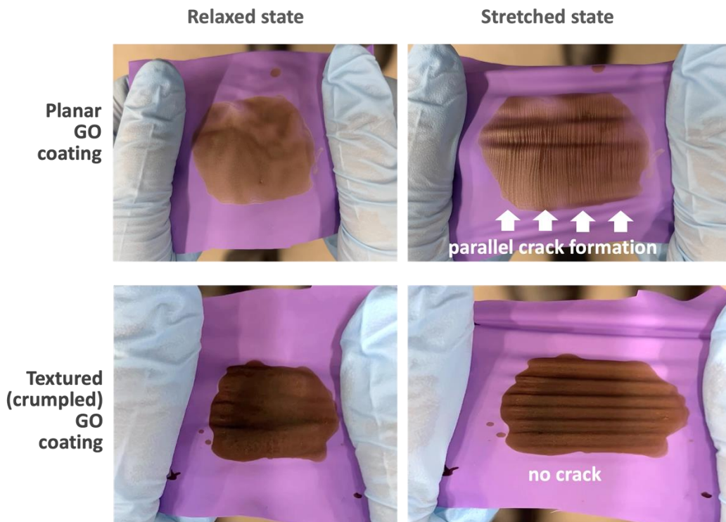
Figure 10. Demonstration that compressive pre-texturing of graphene oxide films renders them stretchable, with no cracks observed over multiple stretch and relax cycles. Films ( 0.5\ \mu\text{m} thick) were formed by solution casting of pure graphene oxide (no polymer additive) on nitrile glove cutouts. Still images extracted from video original (see Video S1, S2).
