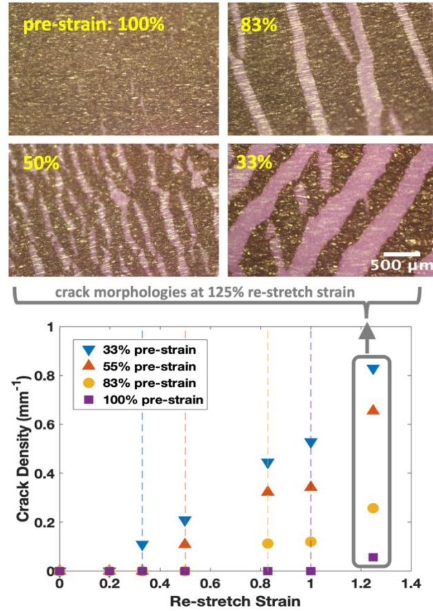
Figure 11. Stretchability limits for pure GO films (0.5 μm thickness) characterized by optical analysis of crack initiation and growth during stretching. Top images: examples of optical images of cracks formed on pre-stretched films after re-stretching at 125% strain. Bottom graph: crack densities for pure graphene oxide films on nitrile substrates fabricated with various pre-stain levels (33-100%) while undergoing re-stretch to and beyond the pre-stretch value. Reversible, crack-free stretchability can be achieved at linear strains up to 100%.
