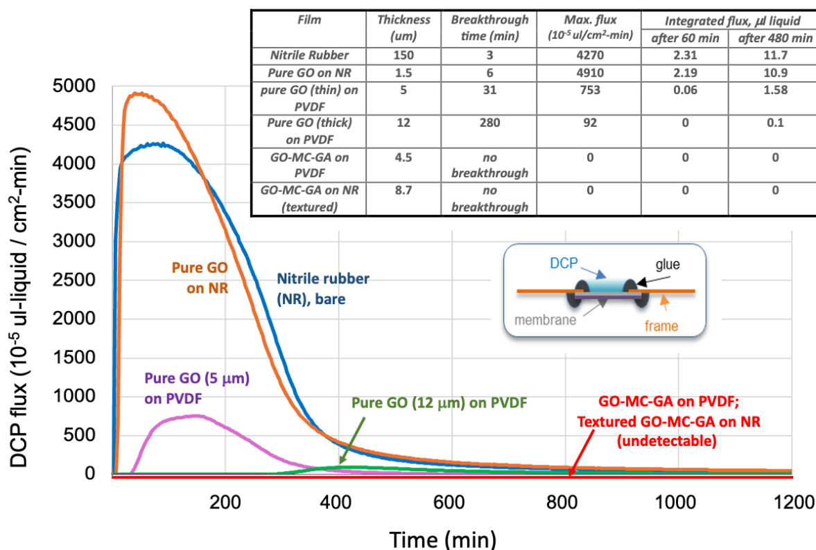
Figure 7. Permeation of the nerve agent simulant diethyl chlorophosphate through oven-dried graphene-based test films under conditions of direct liquid contact. The dynamic method gives DCP flux vs. time, and the table gives key quantitative metrics of performance. The inset shows the experimental configuration that produces direct continuous contact between the DCP liquid and top surface of the test membrane. The textured GO-MC-GA film was prepared using 50% pre-stretch. Small Z-offsets near the baseline were artificially introduced to enable visualization of the data for the best performing barriers.
