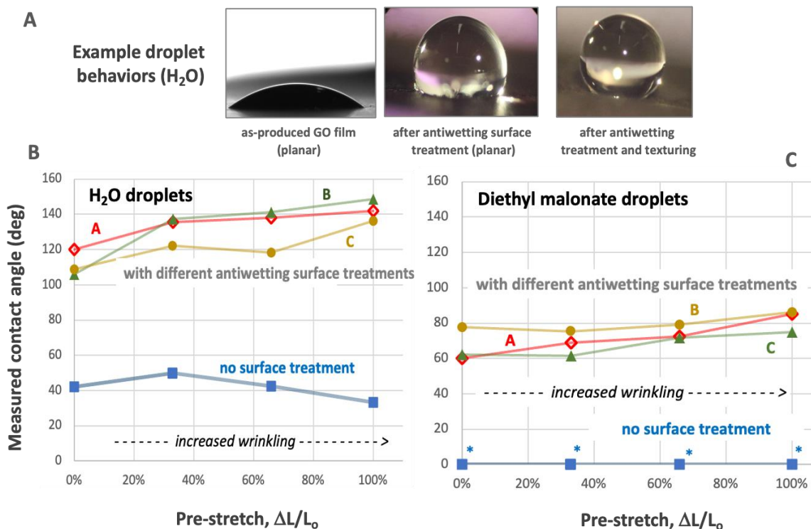
Figure 13. Liquid wetting of graphene-oxide-based films: effects of wrinkling (texturing) and antiwetting spray surface treatments. A: Example sessile liquid droplets showing suppression of wetting/spreading through antiwetting spray treatment (treatment C) and through the combination of the same treatment and compressive texturing (66% pre-stretch). Bottom: quantitative data on static advancing contact angles as a function of treatment type (three antiwetting agents) and extent of compressive texturing expressed as %-pre-stretch before relaxation. B: water; C: diethyl malonate as a polar organic compound and neurotoxicant simulant[69]. Wetting of both liquids on graphene-oxide-based films can be significantly suppressed by currently available antiwetting spray treatments and the suppression can be further enhanced by compressive film texturing. Standard errors for contact angle data (combined drop-to-drop and film-to-film) of \pm 3 degrees.
