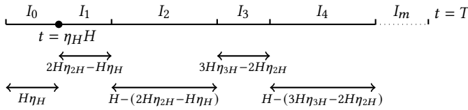
Figure 1: Intervals with fairness and learning phases along the timeline.
