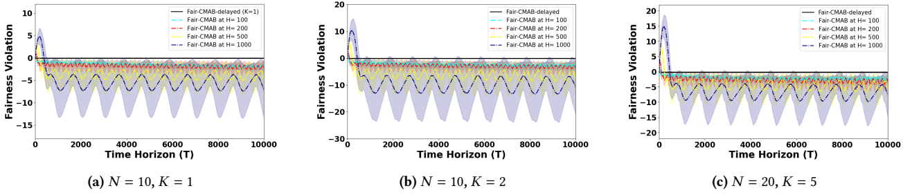
Figure 2: Fairness violations over time.
