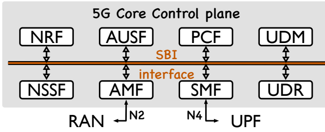
Fig. 1. The architecture of 5G core control plane
