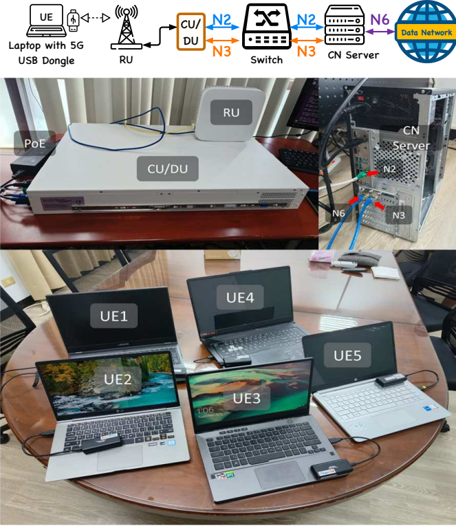
Fig. 5. (Top) The logical topology, and (Bottom) a snapshot of commercial testbed setup in L^2 5GC+ . RU: Radio Unit; DU: Distributed Unit; CU: Central Unit; CN: Core Network; PoE: Power over Ethernet; 5 laptops as UEs with 5G dongles
