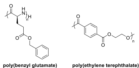
Figure 1: Chemical structures of poly(BG) and PET. Both polymers possess an aromatic group and an ester in the repeat unit.
