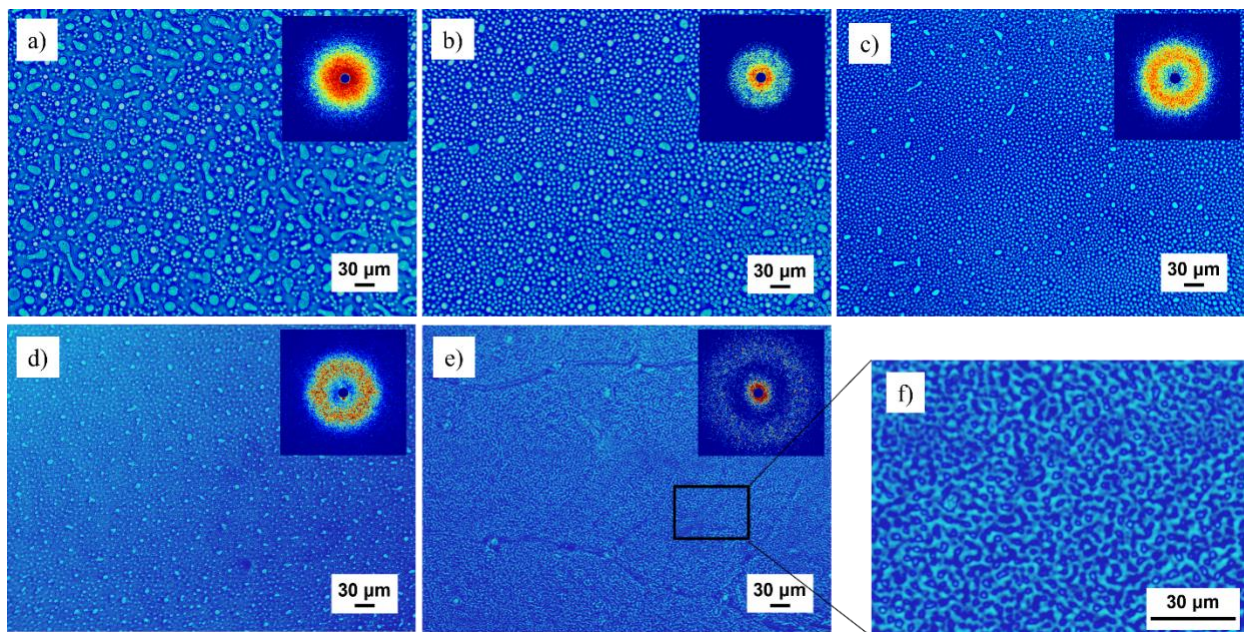
Figure 4: Phase contrast optical microscopy (PCOM) images and small angle laser light (SALLS) scattering patterns of ECel/PET-wt.% compatibilizer blends a) 70/30-0, b) 70/30-5, c) 70/30-10, d) 70/30-20, e) 70/30-30 and f) higher magnification of 70/30-30. Domain sizes decreased and the scattering patterns became more defined and larger by the addition of increasing amounts of ECel- block -poly(BG).
