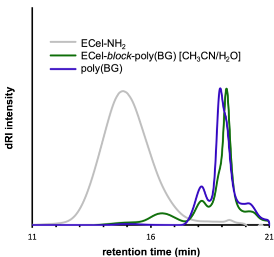
Figure 2: SEC traces of ECel-NH 2 macroinitiator (grey) and polymerization of BG-NTA in 50:50 CH 3 CN:H 2 O initiated by either ECel-NH 2 (green, Table 1 entry 10) or hexylamine (blue). 1 H NMR spectra of macroinitiator ECel-NH 2 and polymerizations can be found in Fig. S5, S11, and S15 . SEC eluent is THF.
