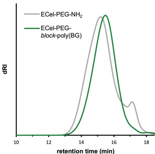
Figure 3: SEC-MALS traces (dRI trace shown) of polymerization of BG-NTA using macroinitiator E Cel-PEG-NH 2 (E Cel-PEG- block -poly(BG), green) along with SEC trace of macroinitiator E Cel-PEG-NH 2 (grey). 1 H NMR spectra can be found in Fig. S10 & S14 . SEC eluent was DMAc/LiCl. M n (NMR) was estimated to be 40.4 kg/mol using poly(BG):ECel ratio. M n (SEC-MALS) was estimated to be 36.7 kg/mol ( D = 1.4) using a weighted ratio dn/dc of poly(BG) and E Cel.
