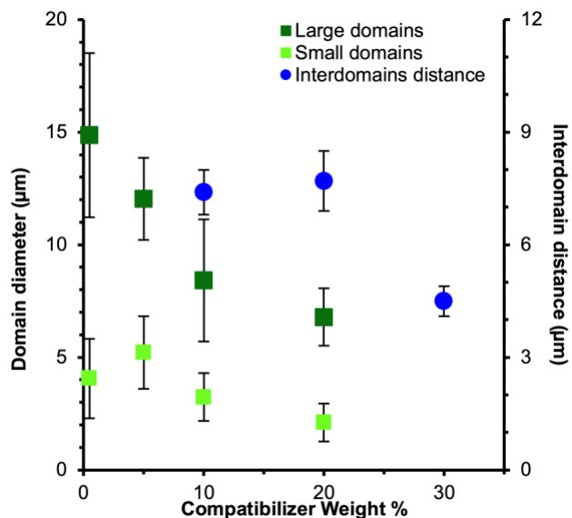
Figure 5: Average domain diameter (PCOM) and interdomain distance (SALLS) of ECEl/PET 70/30 blends as function of ECEl- block -poly(BG) concentration. Diameters and interdomain distance decreased as BCP compatibilizer content increased.
