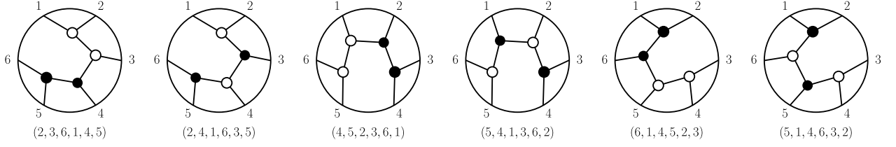
FIGURE 2. An example of a dissection of \Delta_{3,6} that cannot be obtained from the BCFW-style recursion in Theorem 4.5.
