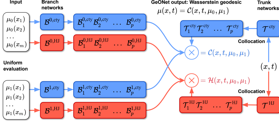
Figure 2: Architecture of GeONet. The solution to CE yields the geodesic. GeONet branches and trunks output vectors of dimension p , in which we perform multiplication among neural network elements to produce the solutions to CE and HJ.
