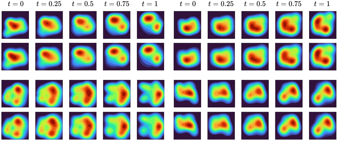
Figure 4: Geodesics predicted by GeONet on bivariate Gaussians over a square domain. The top of each pair is the reference solution computed by POT, and the bottom is GeONet.
