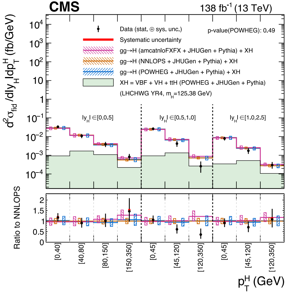
Fig. 60. Double-differential cross sections for Higgs boson production in the H \rightarrow ZZ \rightarrow 4\ell decay channel. The cross section is measured in bins of the rapidity of the Higgs boson |y_H| , as a function of the Higgs boson transverse momentum p_T^H . Source: Figure taken from Ref. [544].
