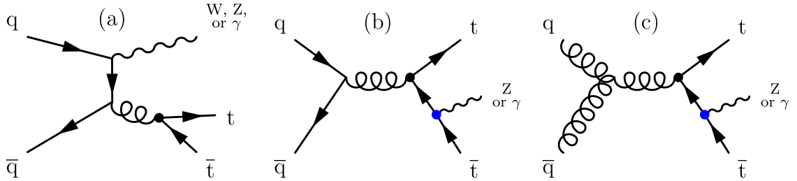
Fig. 43. Example Feynman diagrams for the production of t\bar{t} with a vector boson through initial state radiation (a) or a direct coupling to the top quark (b and c). The latter is only possible for neutral bosons V^0 = \gamma, Z .
