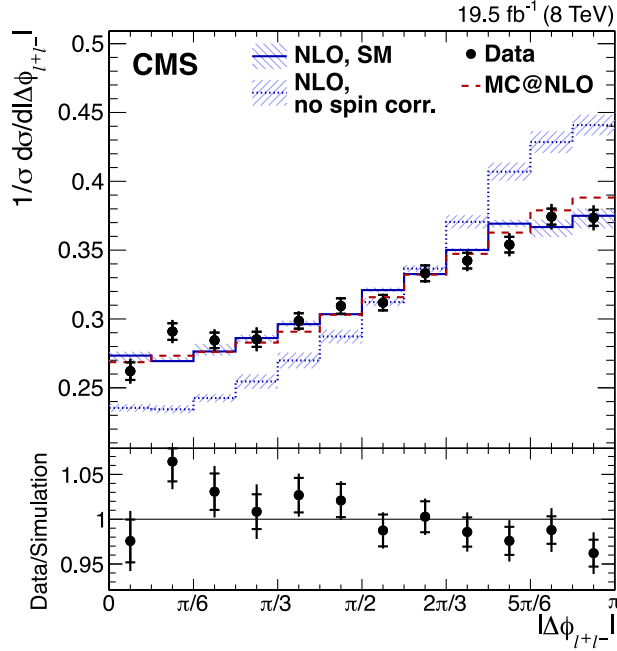
Fig. 42. Normalized differential cross section as a function of the azimuthal opening angle between the two charged leptons in a t\bar{t} dilepton final state ( |\Delta\phi_{\ell^+\ell^-}| ) from data (points); parton-level predictions from MC@NLO (dashed histograms); and theoretical predictions at NLO with (SM) and without (no spin corr.) spin correlations (solid and dotted histograms, respectively). The ratio of the data to the MC@NLO prediction is shown in the lower panel. The inner and outer vertical bars on the data points represent the statistical and total uncertainties, respectively. The hatched bands represent variations of \mu_R and \mu_F simultaneously up and down by a factor of 2. Source: Figure from Ref. [440].
