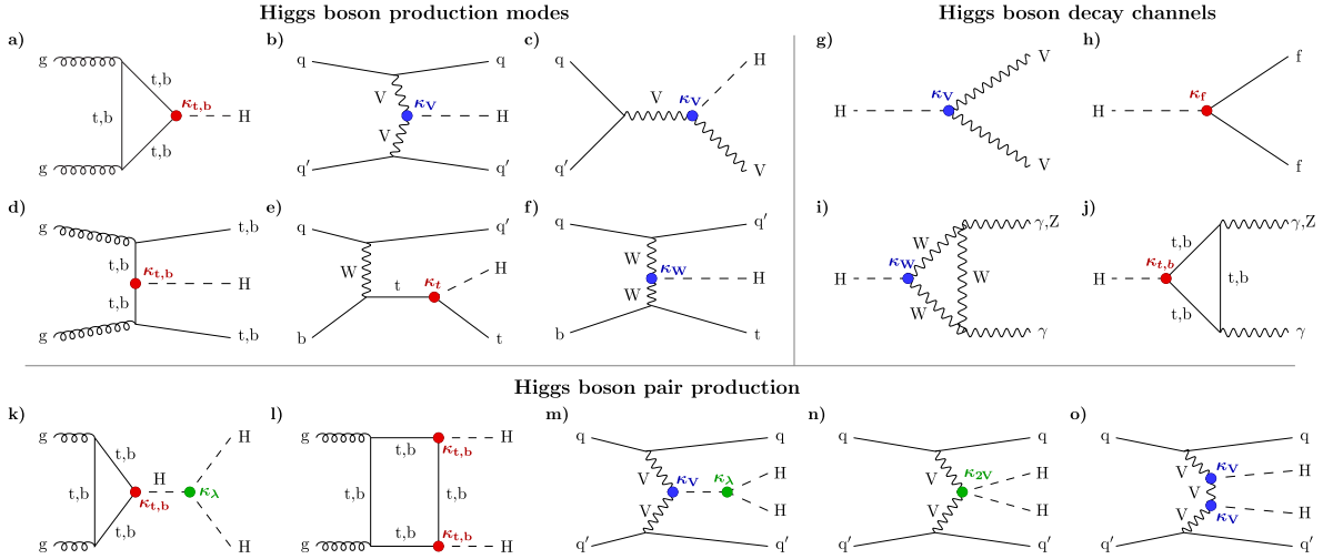
Fig. 54. Higgs boson production in (a) gluon-gluon fusion (ggH), (b) vector boson fusion (VBF), (c) associated production with a W or Z ( V ) boson (VH), (d) associated production with a top or bottom quark pair ( ttH or bbH ), (e, f) associated production with a single top quark ( tH ); with Higgs boson decays into (g) heavy vector boson pairs, (h) fermion-antifermion pairs, and (i, j) photon pairs or Z\gamma ; Higgs boson pair production: (k, l) via gluon-gluon fusion, and (m, n, o) via vector boson fusion. The corresponding Higgs boson interactions are labelled with the coupling modifiers \kappa , and highlighted in different colours for Higgs-fermion interactions (red), Higgs-gauge-boson interactions (blue), and multiple Higgs boson interactions (green). The distinction between a particle and its antiparticle is dropped.
