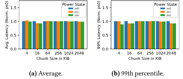
Figure 6. SSD2 random read latency (queue depth 1).
