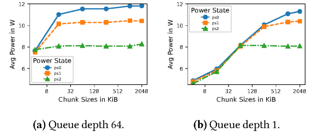
Figure 3. SSD2 random write average power under different power states.
