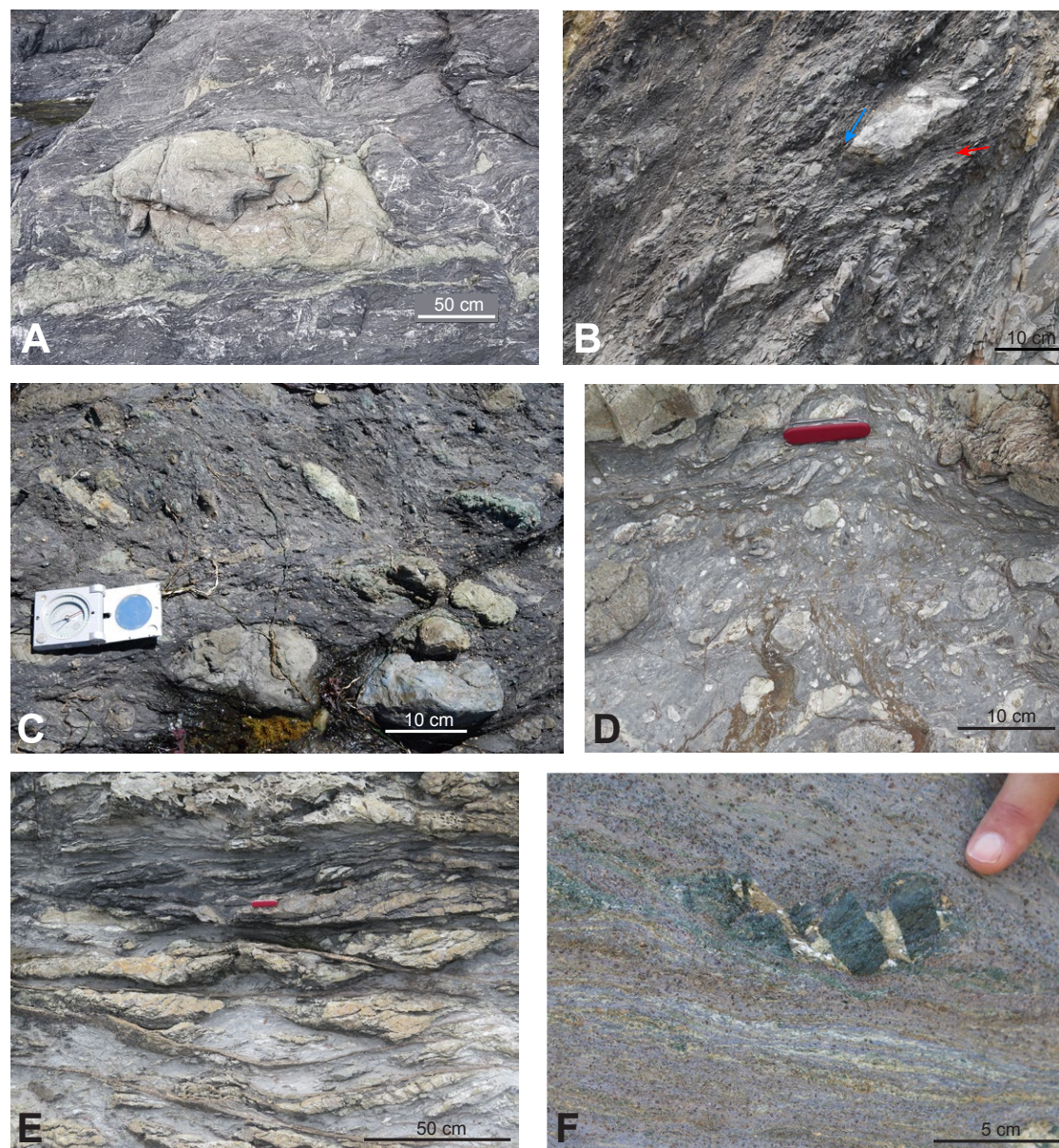
Figure 7. Block-in-matrix mélanges. (A) Basalt block with cataclasites developed along block margin within shale matrix, Upper Mugli mélangé, Japan. 190 °C (Phillips et al., 2020a). (B) Brittle fault gouge in graywacke sandstone and shale, Franciscan Complex, Cayucos, California (35.4493°N, 120.9513°W) (Platt, 2015). This is an exhumation-related normal fault in rocks buried to ~15 km depth during Late Cretaceous subduction. Note disrupted quartz vein. Gouge fabric dips gently left (red arrow), and brittle shear bands dip more steeply left (blue arrow). The structures in this fault zone are characteristic of brittle faults formed in a wide variety of environments, and it is difficult to identify geologic signatures that could indicate they were responsible for slow earthquakes (cf. Fig. 6A). (C) Blocks of graywacke sandstone, blueschist (bottom right), and greenstone (top right) in scaly clay mélangé, San Simeon, California (35.6008°N, 121.1344°W). 100–150 °C, 0.5 GPa (Ukar and Cloos, 2014). (D) Random fabric block-in-matrix mélangé, Chrystalls beach, Otago, New Zealand (46.1897°S, 170.1155°E). <300 °C, 0.4–0.6 GPa (Fagereng et al., 2011). (E) Sheared block-in-matrix mélangé, Chrystalls beach, Otago, New Zealand (46.1897°S, 170.1155°E). The shears are occupied by fiber-lineated quartz veins (see Fig. 5B). These structures were cited as a possible source of tremor and slow slip (Fagereng et al., 2011). (F) Eclogite blocks (green) in blueschist with dilational fractures, Kini beach, Syros, Greece, cited by Kotowski and Behr (2019) as a slow-slip signature. Photos in B–F are by John Platt.
