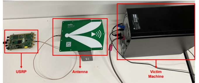
Fig. 2: Experimental setup: signal measurement equipment USRP B210
