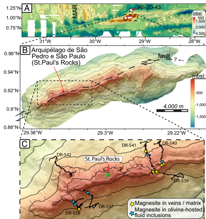
Fig. 1. (A) Map of the St. Paul's transform fault area compiled using bathymetric data collected during the COLMEIA cruise (34). MAR = Mid-Atlantic Ridge. Star indicates the location of dredge Ali-20-43 containing vesicular alkali basalt. (B) Newly processed map acquired during cruise AL170602. Dashed line indicates location of transform fault. Dashed box indicates map area in panel C. (C) Detailed view of bathymetry, HOV dive tracks, and locations where magnesite-bearing rocks (yellow stars) and fluid inclusions (blue stars) were sampled with HOV Deep Rover .
