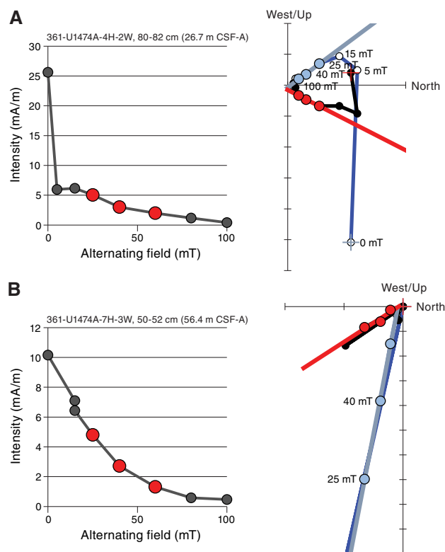
Figure F27. A, B. Alternating field demagnetization results for two representative samples from Hole U1474A. Left panels show the loss in NRM with progressing demagnetization, right panels show orthogonal projections of the demagnetization paths. Black (white) symbols mark the projections on the horizontal (vertical) plane. Red and blue circles indicate which demagnetization steps were used for PCA. The sample in A originates from the Brunhes and has an inclination of -41^\circ and declination of 70^\circ , whereas the sample in B is from the Matuyama Chron and has an inclination of 46^\circ and declination of 173^\circ . Note that the declinations of these examples are not corrected for core orientation.
