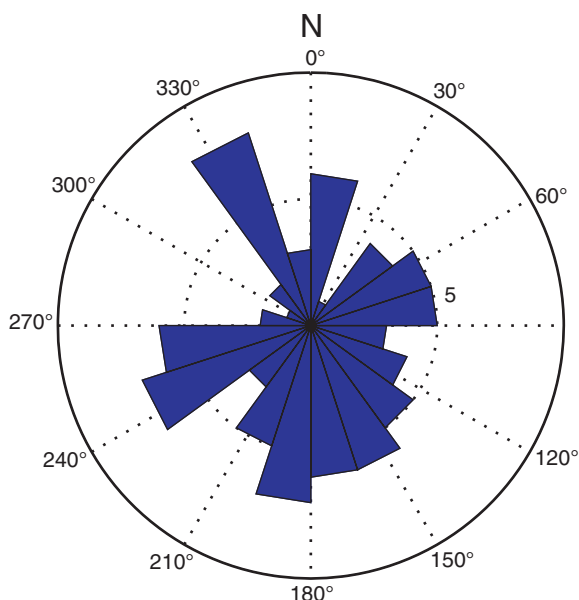
Figure F26. Rose diagram of declinations of maximum magnetic susceptibility ( V_1 ) corrected for core orientations plotted downhole. See Figure F25E.
