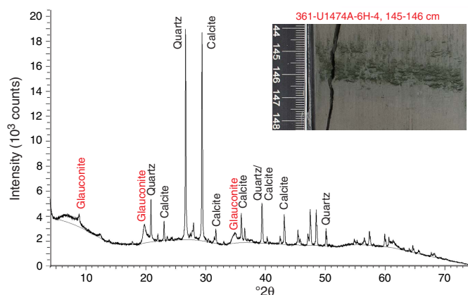
Figure F11. XRD diffractogram of bulk powders from diagenetic altered layers, Hole U1474A. Analysis indicates the presence of quartz and calcite, as well as glauconite.
