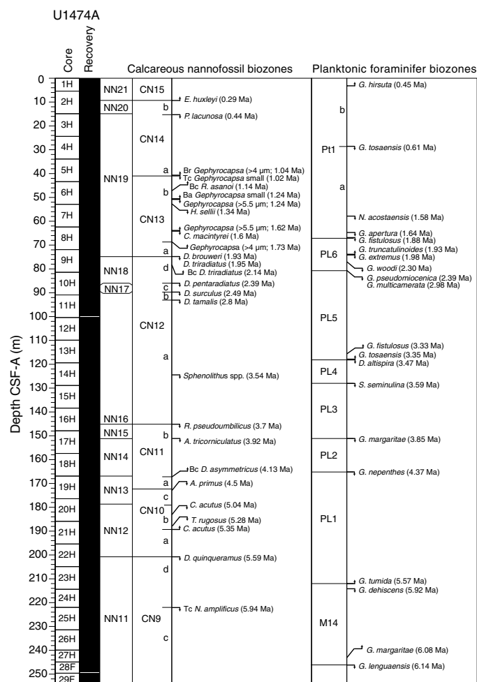
Figure F19. Biochronology at Site U1474 with calcareous nannofossils and the locations of significant planktonic foraminifer events. Upward arrows indicate the base: base reentrance (Br), base common (Bc), and base acme (Ba) occurrences for nannofossils and base occurrences for planktonic foraminifers. Downward arrows indicate the top and top common (Tc) occurrences. Biochronology is based entirely on sampling in Hole U1474A.
