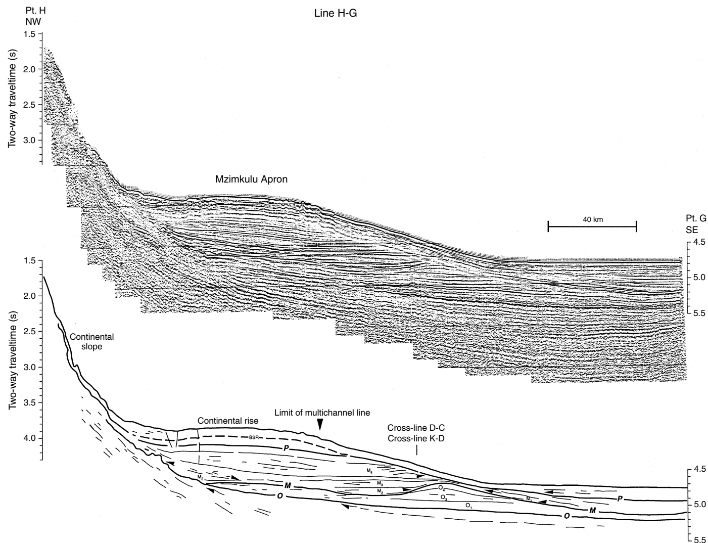
Figure F4. Precruise interpretation of seismic Line H–G (Niemi et al., 2000) near Site U1474 (see Figure F3 for location), extending from the continental slope, across the continental rise, and into the Natal Valley abyssal plain. P = Pliocene, M = Miocene, O = Oligocene.
