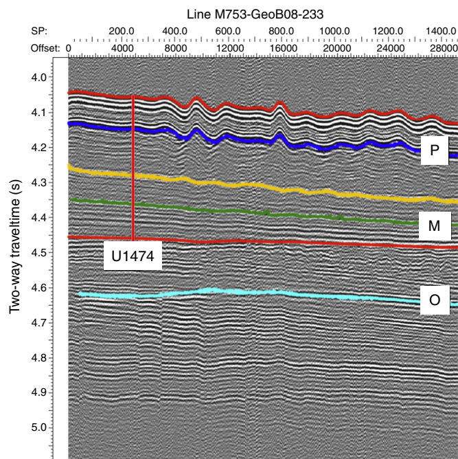
Figure F5. Precruise interpretation of seismic Line M753-GeoB08-233 at Site U1474. SP = shotpoint.
