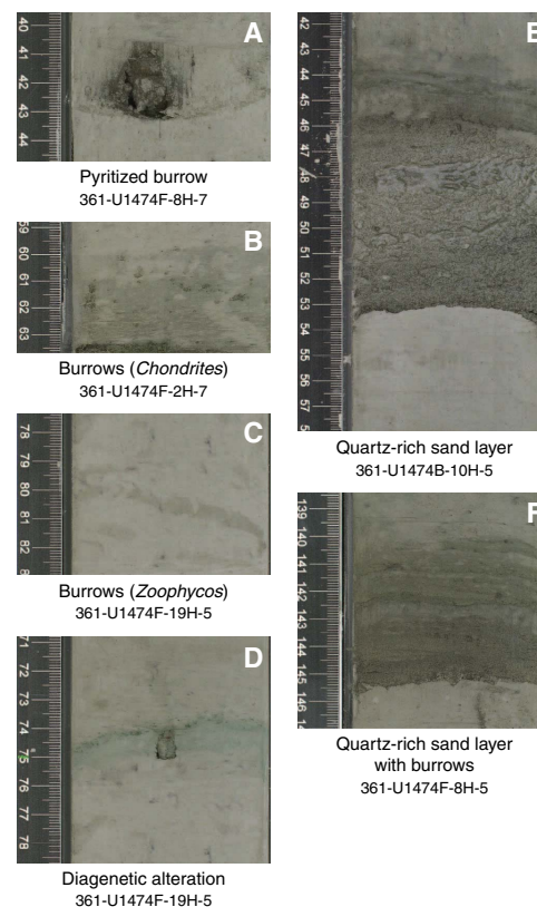
Figure F10. A–F. Representative sedimentary structures and lithologic accessories, Site U1474.
