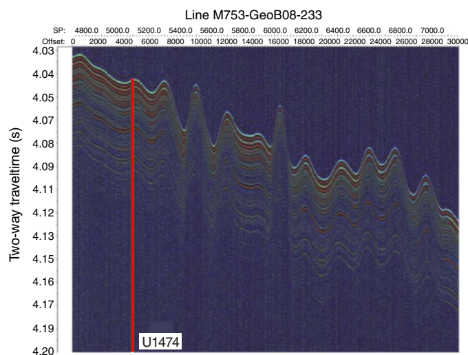
Figure F6. Parasound Line M753-GeoB08-233 showing parallel reflectors at Site U1474. Labels on the vertical axis are chosen to represent ~10 m (13.3 ms two-way traveltime).
