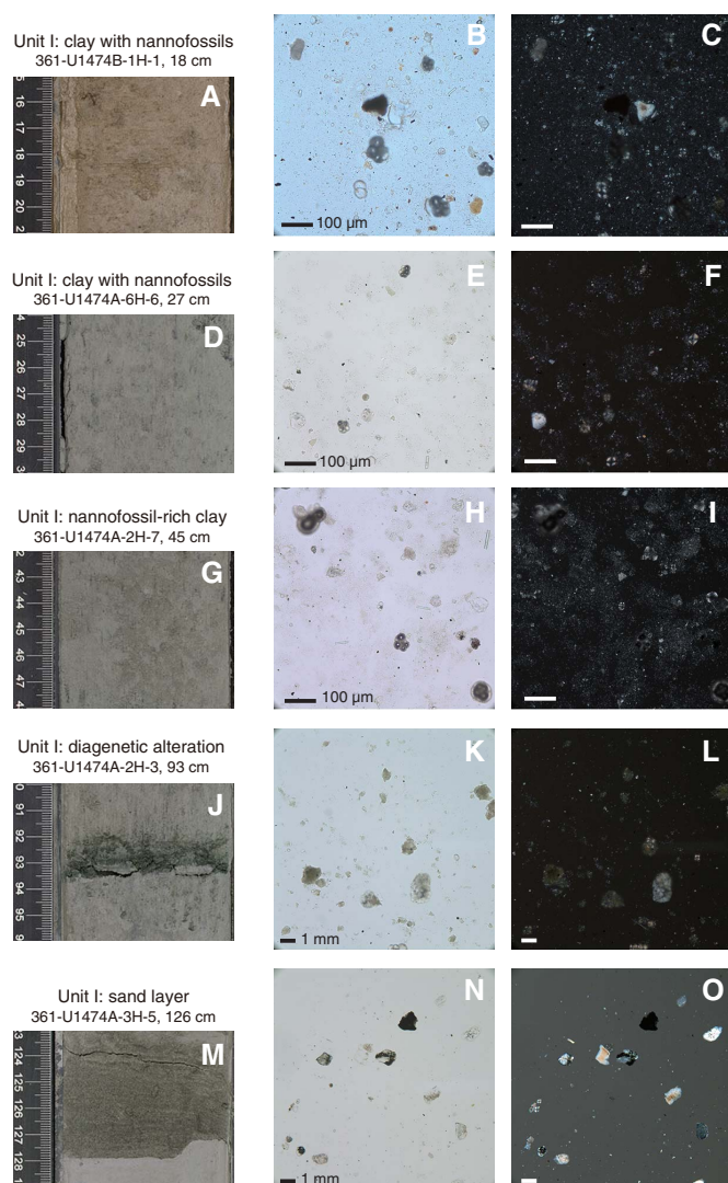
Figure F9. A–O. Representative lithologies per interval. Section-half (left) surfaces and smear slide photomicrographs taken under plane-polarized (middle) and cross-polarized (right) light, Site U1474.
