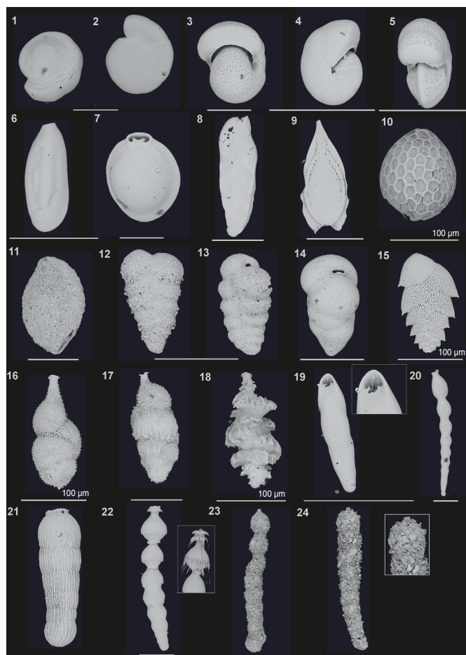
Figure F23. Most common benthic foraminifers, Hole U1474A. Scale bar = 200 \mu\text{m} unless otherwise indicated. 1, 2. Gyrodinoides soldanii (4H-5, 70–72 cm). 3. Melonis affinis (4H-5, 70–72 cm). 4, 5. Melonis barleeianum (4H-5, 70–72 cm). 6. Quinqueloculina bradyana (4H-CC). 7. Pyrgo anomala (6H-CC). 8. Bolivinita quadrilatera (5H-CC). 9. Fissurina formosa (5H-CC). 10. Oolina hexagona (7H-CC). 11. Sigmoilopsis schlumbergeri (4H-4, 70–72 cm). 12, 13. Textularia agglutinans (4H-5, 70–72 cm; 4H-CC). 14. Karrerella bradyi (4H-2, 70–72 cm). 15. Bolivina alata (4H-5, 70–72 cm). 16. Uvigerina proboscidea (6H-CC). 17. Uvigerina bradyana (5H-CC). 18. Siphonovigenerina porrecta (6H-CC). 19. Pleurostomella alternans (4H-CC). 20. Mylostomella fijiensis (7H-CC). 21. Chrysalogonium breviloculum (4H-5, 70–72 cm). 22. Siphonodosaria lepidula (4H-CC). 23. Martinotiella variabilis (4H-5, 70–72 cm). 24. Reophax sp. (4H-5, 70–72 cm).
