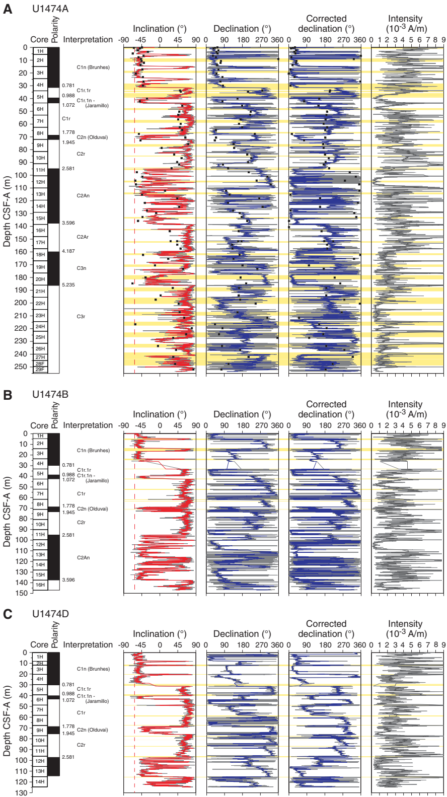
Figure F28. Downhole paleomagnetic results, Site U1474. Inclination, declination, corrected declination, and intensity after 25 mT AF demagnetization are plotted according to their individual CSF-A depth scales. Inclination: gray line = continuous SRM data, red line = 10-point smoothed record, vertical dashed line = present-day inclination. Declination: gray line = data, blue line = 10-point smoothed record, yellow shaded horizontal bars = core disturbance intervals. Polarity chron ages after Gradstein et al. (2012). A. Hole U1474A. Black squares = ChRM obtained by PCA of discrete sample demagnetization data. B. Hole U1474B. C. Hole U1474D. (Continued on next page.)
