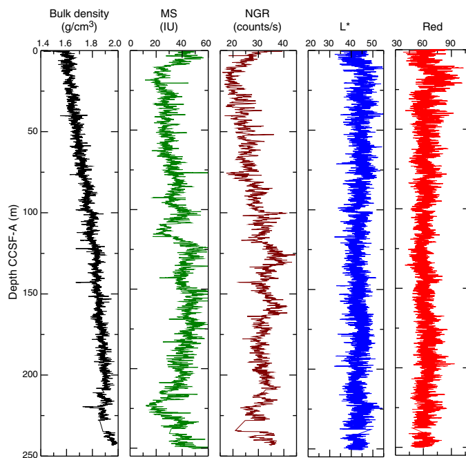
Figure F18. Spliced bulk density, WRMSL magnetic susceptibility, NGR, sediment L^* , and red color band records, Site U1474.
