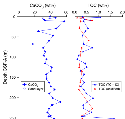
Figure F38. Calcium carbonate and TOC profiles, Hole U1474A. Carbonate content of sandy layers are plotted separately. Organic carbon was measured by two methods: subtraction of carbonate content from total carbon content (TC – IC) and direct measurement after acidification of carbonate.
