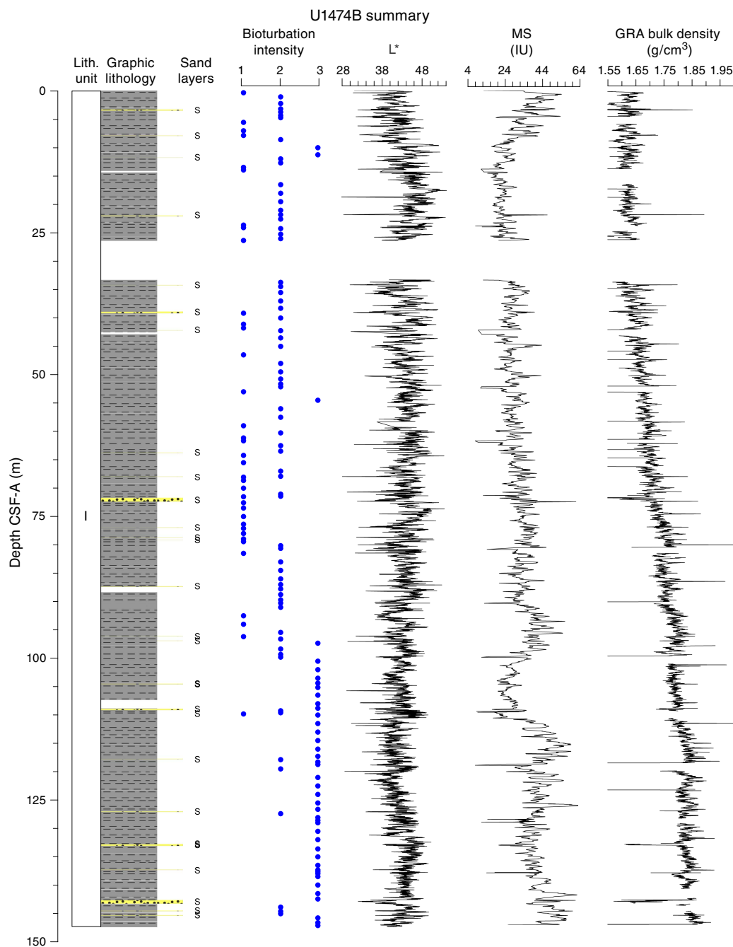
Figure F8 (continued). B. Hole U1474B. (Continued on next page.)
