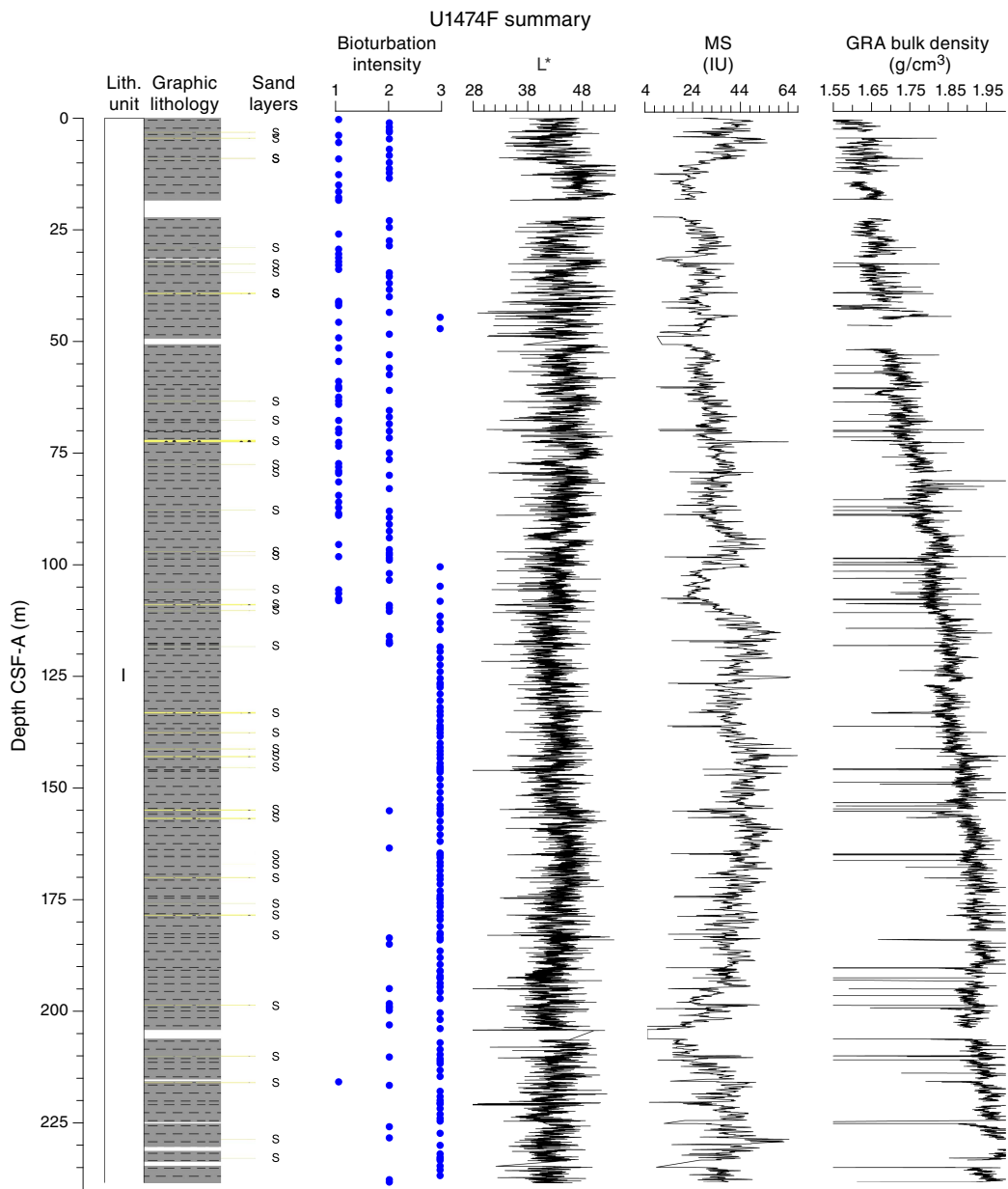
Figure F8 (continued). E. Hole U1474F.
