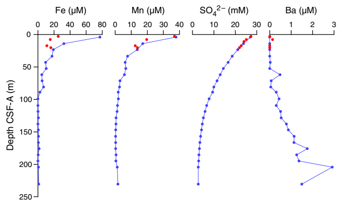
Figure F35. Dissolved iron, manganese, sulfate, and barium profiles, Holes U1474A (blue) and U1474B (red).
