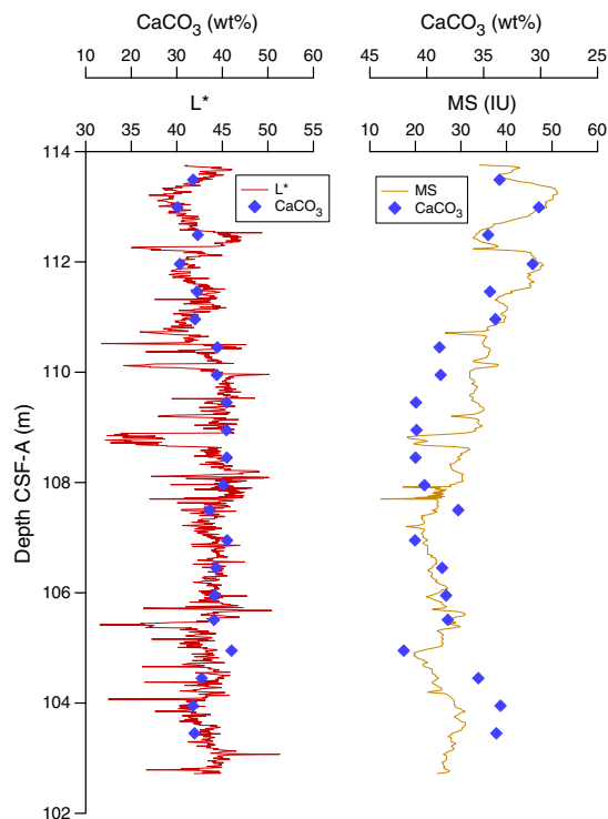
Figure F40. Calcium carbonate vs. MS (right) and L* (left), Cores 361-U1474F-12H and 13H.
