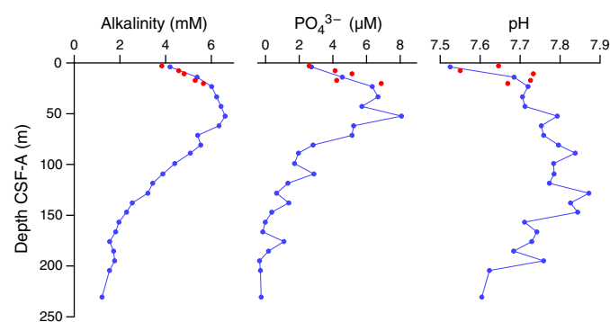
Figure F34. Alkalinity, dissolved phosphate, and pH profiles, Holes U1474A (blue) and U1474B (red).
