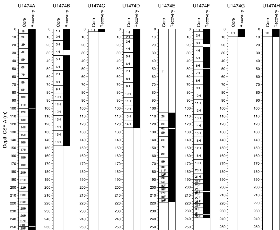
Figure F7. Core recovery, Holes U1474A–U1474H.
