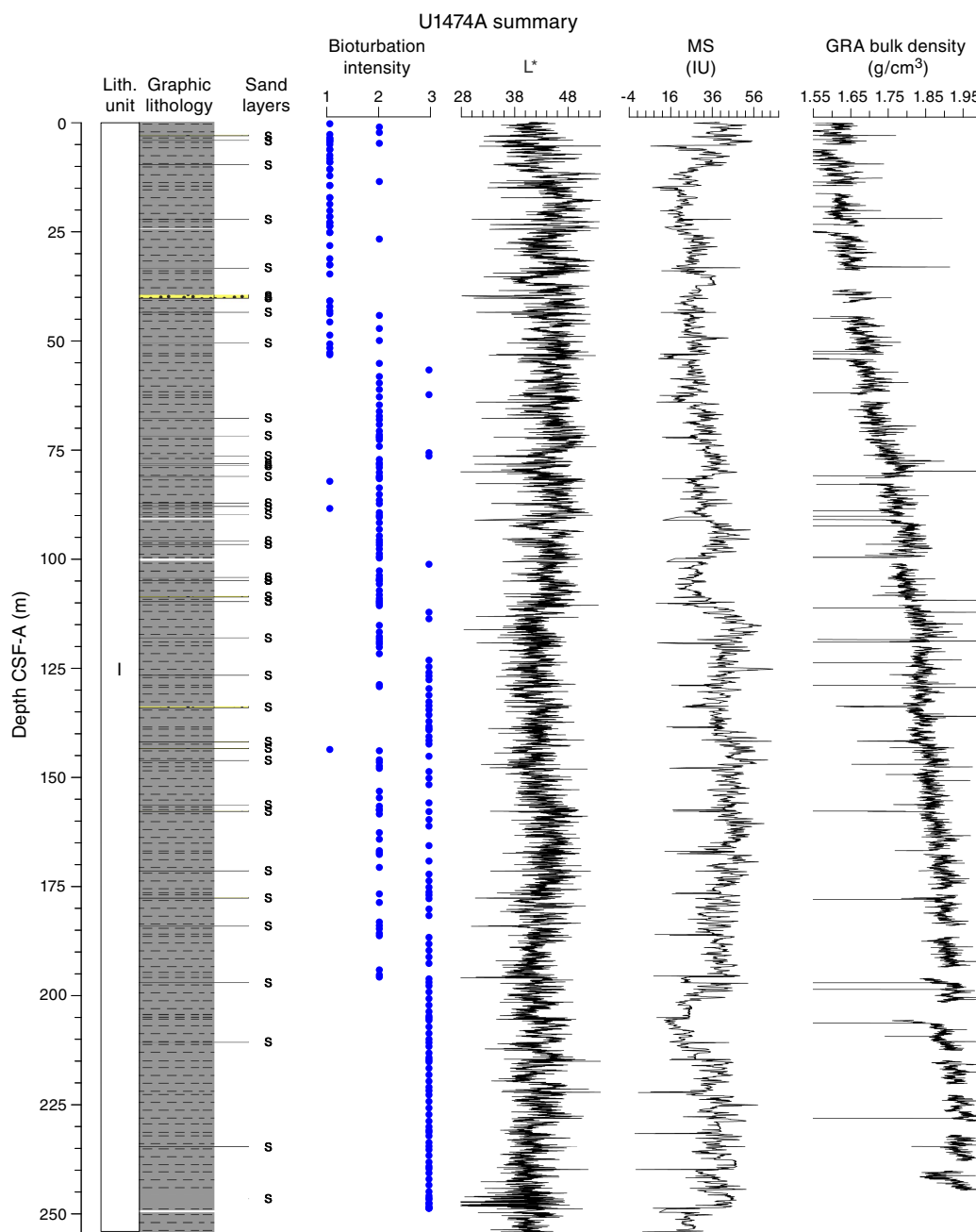
Figure F8. Lithostratigraphic summary with selected physical property and geochemical data. Holes U1474C and U1474H are composed of only one core each and are presented in the visual core descriptions (see Core descriptions ). Bioturbation intensity: 1 = slight, 2 = moderate, 3 = strong. A. Hole U1474A. (Continued on next four pages.)
