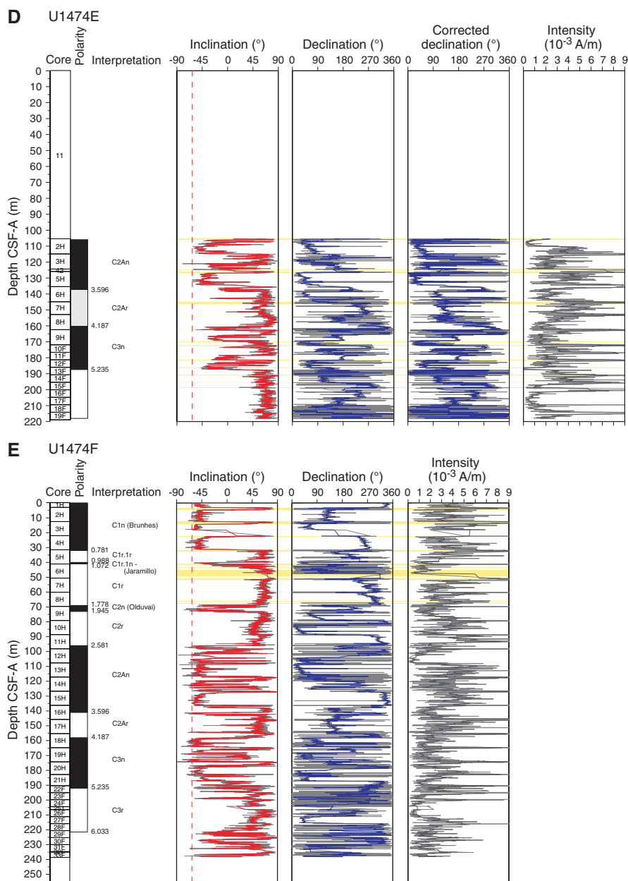
Figure F28 (continued). D. Hole U1474E. E. Hole U1474F.
