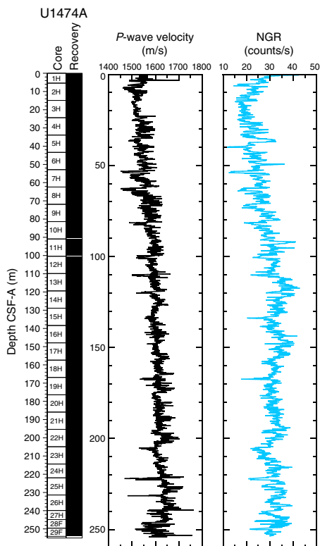
Figure F15. P -wave velocity and NGR, Hole U1474A.
