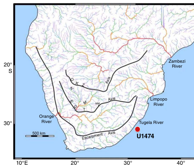
Figure F3. Drainage system of southern Africa adapted from Moore et al. (2009). Colors denote stream rank from 1 (purple) to 5 (red). For reference, Rank 5 streams are considered medium streams in the terminology of Strahler (1952). The major river divides are interpreted by Moore et al. (2009) to reflect epeirogenic uplift axes, progressively younger from inland toward the margin. OKZ = Ovambo-Kalahari-Zimbabwe, EGT = Etosha-Griqualand-Transvaal. M = Molopo River, N = Nossob River, MM = Mahura Muhlta.
