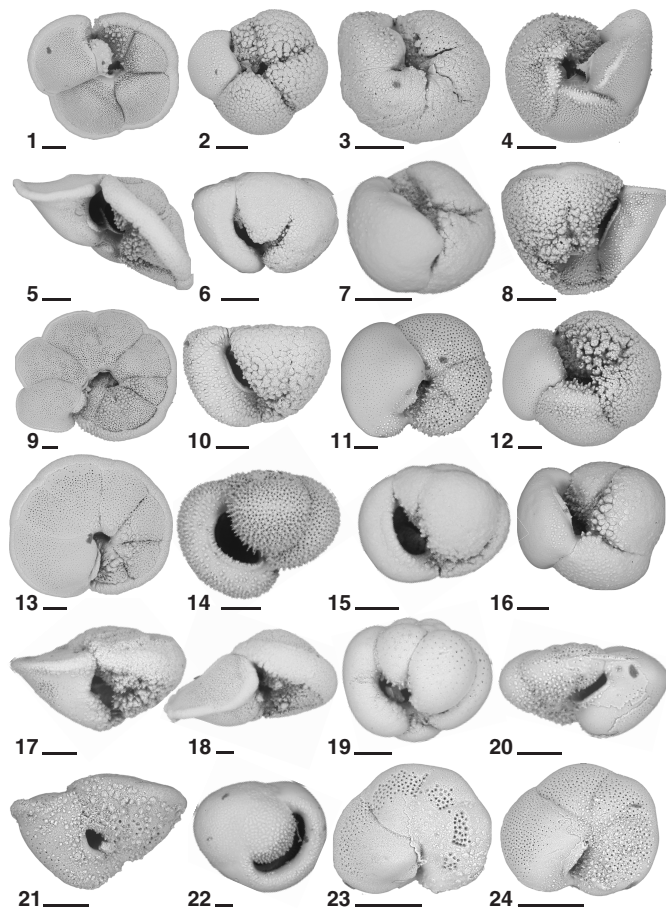
Figure F21. Planktonic foraminifers, Hole U1474A. Scale bars = 100 \mu m. 1. Globorotalia menardii (1H-4, 70–72 cm). 2. Globorotalia crassula (9H-2, 70–72 cm). 3. Globorotalia tosaensis (5H-7, 70–72 cm). 4. Globorotalia truncatulinoides (1H-4, 70–72 cm). 5. Globorotalia flexuosa (2H-6, 70–72 cm). 6, 7. Globoconella sphericomiozea (12H-4, 70–72 cm). 8. Globorotalia truncatulinoides (1H-4, 70–72 cm). 9. Globorotalia multicamerata (9H-6, 70–72 cm). 10. Globoconella puncticulata (12H-4, 70–72 cm). 11. Globorotalia scitula (1H-4, 70–72 cm). 12. Globorotalia crassaformis (1H-4, 70–72 cm). 13. Globorotalia pseudomiocenica (9H-6, 70–72 cm). 14, 15. Globorotalia inflata (3H-4, 70–72 cm). 16. G. inflata (1H-4, 70–72 cm). 17. Globoconella conomiozea (24H-CC). 18. Globorotalia tumida (2H-6, 70–72 cm). 19. Pulleniatina primalis (24H-CC). 20. Globorotalia cibaoensis (28H-4, 70–72 cm). 21. Globorotalia merotumida (28H-CC). 22. Pulleniatina obliquiloculata (1H-4, 70–72 cm). 23. Globorotalia linguaensis (28H-4, 70–72 cm). 24. Globorotalia paralangaensis (27H-1, 70–72 cm).
