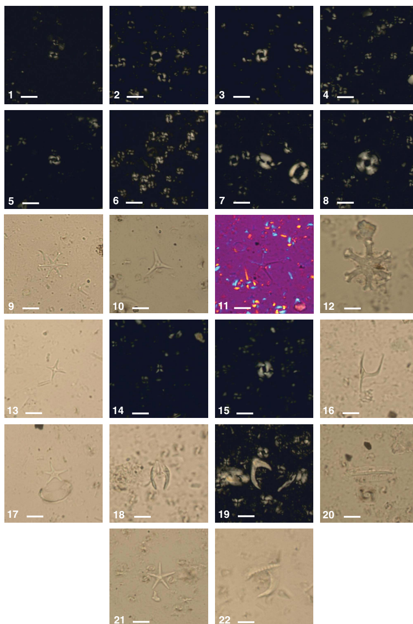
Figure F20. Calcareous nannofossils, Hole U1474A. Scale bars = 5 µm. 1. Emiliania huxleyi (mudline). 2. Pseudoemiliania lacunosa (6H-3, 75 cm). 3. Reticulofenestra asanoi (4H-4, 75 cm). 4. small Gephyrocapsa spp. (<4 µm) (2H-4, 70 cm). 5. Gephyrocapsa oceanica ( Gephyrocapsa spp. >5.5 µm) (mudline). 6. Gephyrocapsa caribbeanica ( Gephyrocapsa spp. 4–5.5 µm) (3H-5, 75 cm). 7. Helicosphaera sellii (7H-5, 75 cm). 8. Calcidiscus macintyreii (8H-2, 75 cm). 9. Discoaster brouweri (11H-3, 75 cm). 10. Discoaster triradiatus (24H-3, 70 cm). 11. Discoaster pentaradiatus under lambda plate (12H-3, 75 cm). 12. Discoaster surculus (23H-3, 75 cm). 13. Discoaster tamalis (12H-3, 75 cm). 14. Sphenolithus abies (17H-3, 75 cm). 15. Reticulofenestra pseudoumbilicus (17H-3, 75 cm). 16. Amaurolithus tricorniculatus (20H-2, 75 cm). 17. Discoaster asymmetricus (12H-3, 75 cm). 18. Amaurolithus primus (20H-2, 75 cm). 19. Ceratolithus acutus (20H-5, 75 cm). 20. Triquetrorhabdulus rugosus (23H-2, 75 cm). 21. Discoaster quinquedramus (23H-4, 75 cm). 22. Nicklithus amplificus (25H-1, 75 cm).
