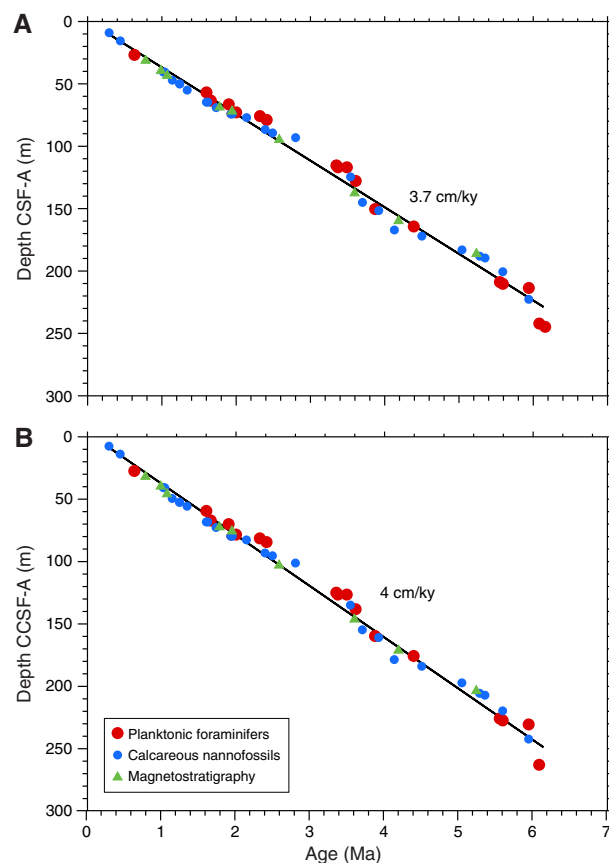
Figure F41. Age-depth relationships for Site U1474 based upon calcareous nannofossils, planktonic foraminifers, and magnetostratigraphic boundaries. The difference in apparent sedimentation rate between the two depth scales reflects the expansion of the spliced composite record in the CCSF-A scale relative to that of the curated sediment thickness (CSF-A scale). Regression lines are a linear fit to all data and forced through the origin, indicating a sedimentation rate of (A) 3.7 cm/ky and a long-term sedimentation rate of (B) 4 cm/ky.
