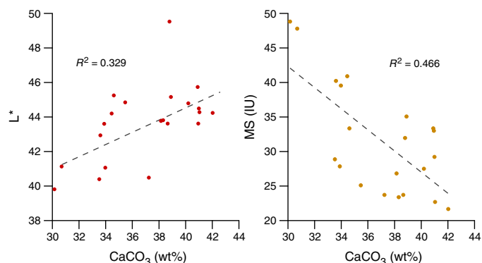
Figure F40. Calcium carbonate vs. MS (right) and L* (left), Cores 361-U1474F-12H and 13H.
