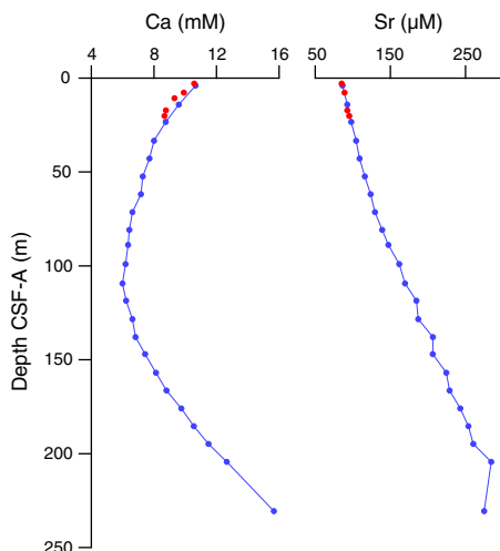
Figure F36. Dissolved calcium and strontium profiles, Holes U1474A (blue) and U1474B (red).
