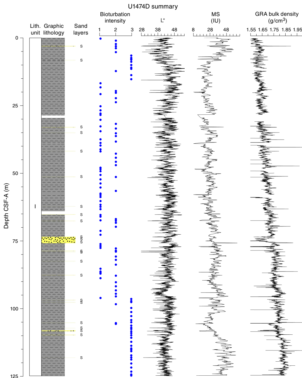
Figure F8 (continued). C. Hole U1474D. (Continued on next page.)
