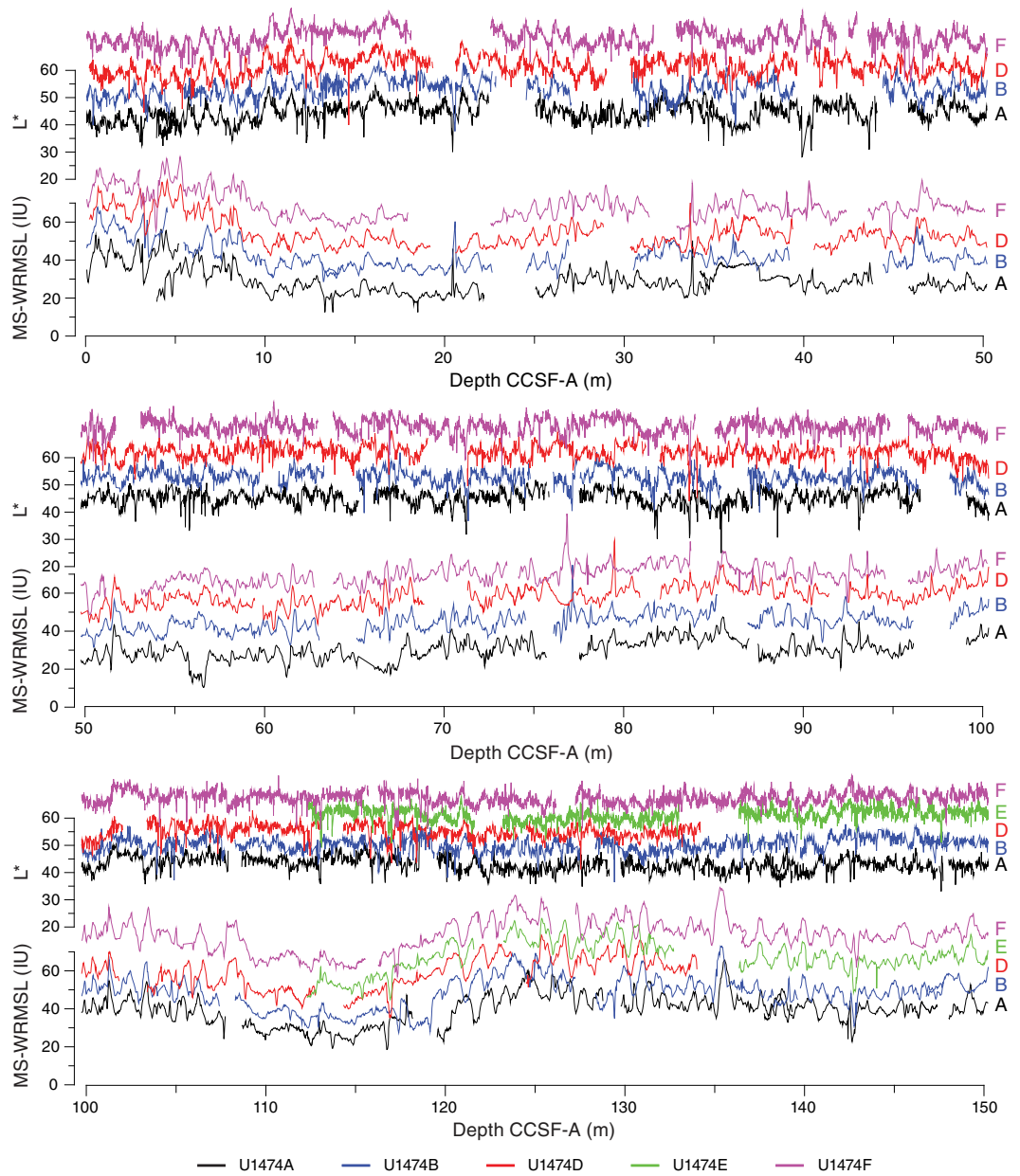
Figure F30. Magnetic susceptibility (MS-WRMSL) and L* records, Site U1474. Compositing of the sequences relied principally on MS-WRMSL data. The flattened traces below 220 m CCSF-A indicate the presence of a sucked-in section accompanying partial strokes. (Continued on next page.)
