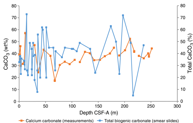
Figure F13. Comparison of \text{CaCO}_3 content determined using measurements on discrete samples and biogenic carbonate proportions estimated in smear slides, Hole U1474A. Low \text{CaCO}_3 abundances (less than ~25%) correspond to samples taken from sand layers.
