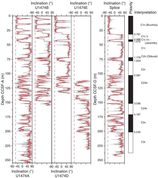
Figure F29. Inclination summary, Site U1474. Dashed lines = present-day inclination.
