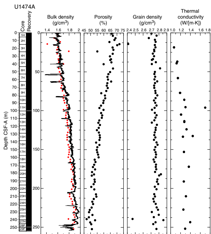
Figure F16. Bulk density (black line = WRMSL measurements, red circles = MAD measurements), porosity, grain density, and thermal conductivity, Hole U1474A.
