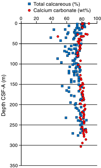
Figure F12. Comparison of \text{CaCO}_3 content determined using measurements on discrete samples and biogenic carbonate proportions estimated in smear slides, Holes U1475A–U1475F.
