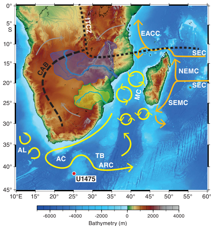
Figure F1. Location map of Site U1475 with main surface currents (arrows) in the southwest Indian Ocean and atmospheric circulation over southern Africa during austral summer (December, January, February) with approximate position of the Intertropical Convergence Zone (ITCZ) and Congo Air Boundary (CAB) (dashed lines; adapted from Reason et al., 2006). AC = Agulhas Current, ARC = Agulhas Return Current, SEC = South Equatorial Current, SEMC = South East Madagascar Current, NEMC = North East Madagascar Current, EACC = East Africa Coastal Current, TB = Transkei Basin. Purple shading = Zambezi Catchment, green shading = Limpopo Catchment, gray double-headed arrows = main pathways of moisture supply to the African continent from the northwest Atlantic (through Congo) and the northwest and southwest Indian Ocean.
