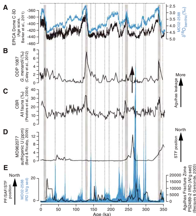
Figure F6. Millennial-scale multiproxy reconstruction of CASQ sediment Core MD02-2588 from the southern Agulhas Plateau (Ziegler et al., 2013), near the STF, along with other published records for comparison. A. Benthic \delta^{18}\text{O} record of Agulhas Plateau Record MD02-2588 (blue) and Antarctic temperature record from EPICA Dome C deuterium (timescale from Barker et al., 2011). B. Concentration of Globorotalia menardii at ODP Site 1087 in the southern Benguela region as a qualitative indicator of Agulhas leakage (Caley et al. 2012). C. Agulhas leakage fauna abundance in the Cape Basin (Peeters et al., 2004). D. Authigenic uranium in Core MD96-2077 in the south-west Indian Ocean. Peaks in authigenic uranium are used to infer local increases in productivity and a northward shift of the STF (Bard and Rickaby, 2009). E. Ice-rafted debris (IRD) record from Core MD02-2588 (blue) and lower resolution IRD record from Core PS2489-2 from the Agulhas Fracture Zone (Gersonde et al. 2003). IRD abundance peaks are also indicative of northward shifts in the SAF.
