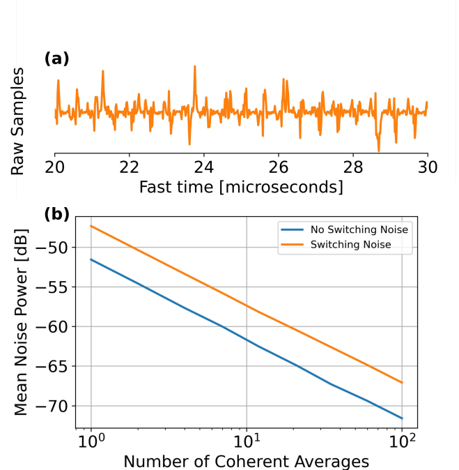
Fig. 6. (a) Noise from a switching power supply presents in the raw time-domain samples as spikes at a rate of 2 MHz (the power supply switching frequency). (b) Effect of this is to increase the initial single-pulse noise floor. While the noise floor can still be reduced by coherent integration, starting at a lower noise floor is desirable to increase SNR for a given coherent integration time. Data collected on a B205mini.
