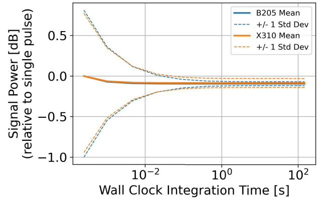
Fig. 3. Signal coherence testing was performed for both SDRs in a loopback configuration. Mean signal power dips only slightly relative to the single recording (unstacked) mean. This indicates good coherence of the system.
