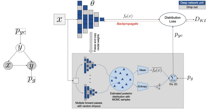
Fig. 1: Left: Directed graphical model during training. Right: Overall training strategy of BUNDL using the observed data x and given labels \hat{y} in every epoch.
