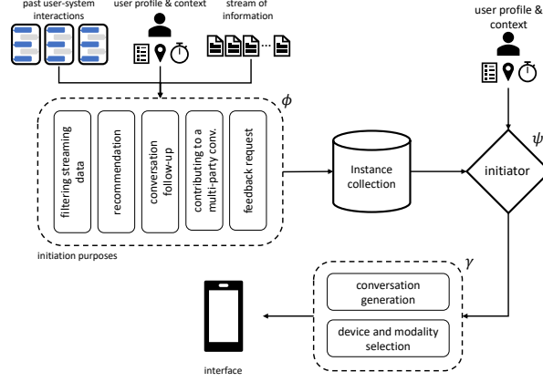
Fig. 2. A generic pipeline for conversation initiation in CIS systems by Wadhwa and Zamani [74].
