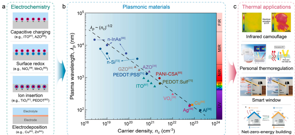
Fig. 2. Mechanisms and applications of electrochemically tunable plasmonic materials. (a) Four electrochemical mechanisms for controlling material properties [57–64]. (b) Carrier density and plasma wavelength for various plasmonic materials [38,65–72]. (c) Representative emerging thermal applications [52–56].
