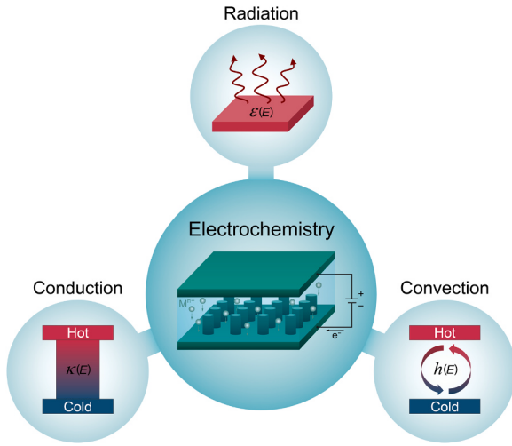
Fig. 1. Electrochemically dynamic thermal metamaterials.
