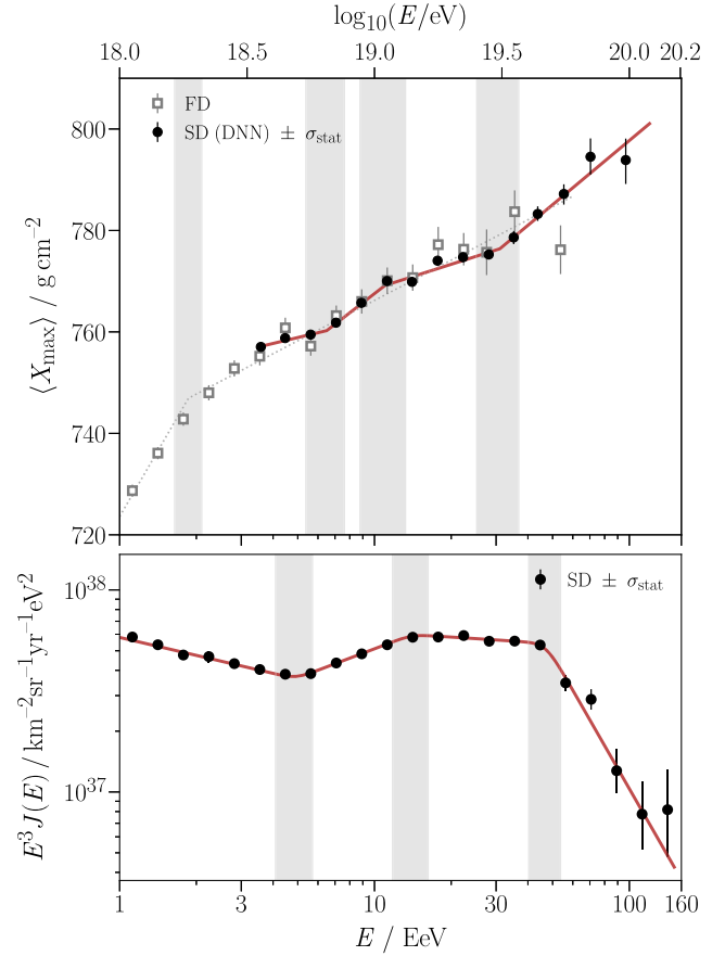
FIG. 3. Positions of breaks in the elongation rate compared to energy spectrum features. Top: Evolution of \langle X_{\max} \rangle as a function of energy for the SD (black) and the FD (gray) [45]. The red line indicates the elongation model found using the SD, and the dotted gray line using the FD. Bottom: Combined energy spectrum [51] as measured using the SD 1500 m array and the low energy 750 m infill array of the Observatory. Gray regions indicate the uncertainties in the energy of the found breaks and features.
