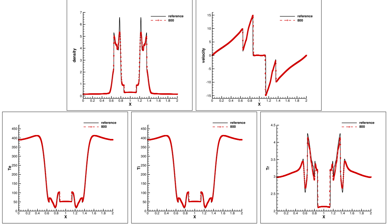
Figure 5.3: The numerical results for Example 5.3 at T = 0.038 by the fifth order finite difference scheme solving the 1D 3-T RH equations (3.1)-(3.2) on the 800 grid. Left and Top: density, Right and Top: velocity, Left and Bottom: electron temperature, Middle and Bottom: ion temperature, Right and Bottom: radiation temperature.
