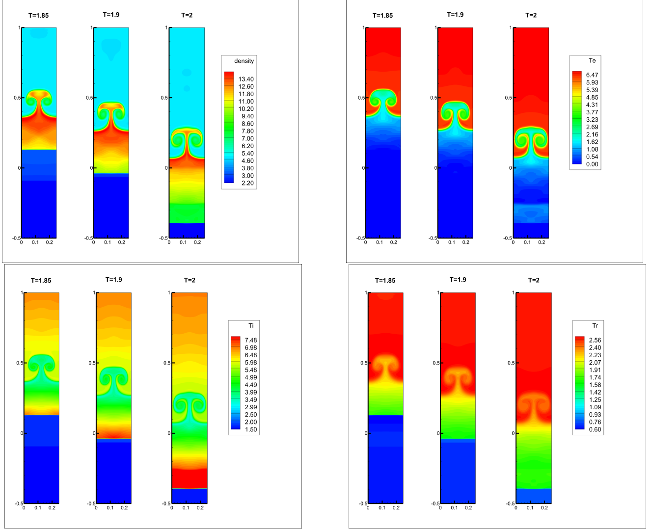
Figure 5.12: The numerical results for Example 5.9 by the fifth order finite difference scheme solving the 2D 3-T RH equations (4.1)-(4.2) with w_{ei} = w_{er} = 0.001 and \kappa_e = \kappa_i = \kappa_r = 0.002 at the different times on the 200 \times 1200 grid. Left and Top: density, Right and Top: electron temperature, Left and Bottom: ion temperature, Right and Bottom: radiation temperature.
