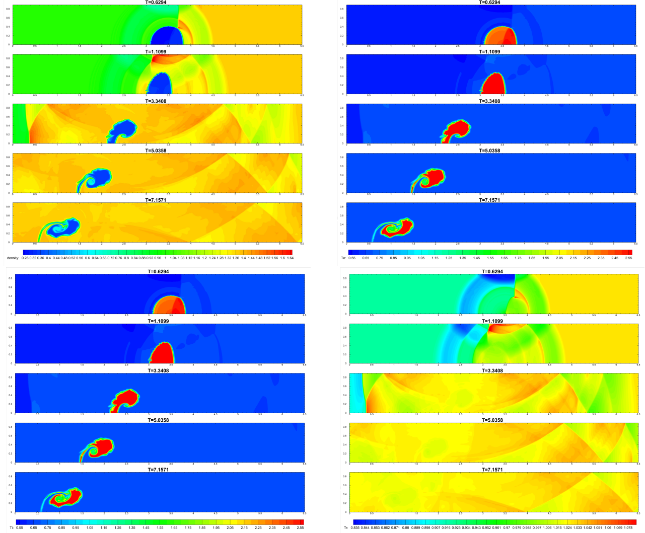
Figure 5.6: The numerical results for Example 5.6 by the fifth order finite difference scheme solving the 2D 3-T RH equations (4.1)-(4.2) at different times on the 800 \times 288 grid. Left and Top: density, Right and Top: electron temperature, Left and Bottom: ion temperature, Right and Bottom: radiation temperature.
