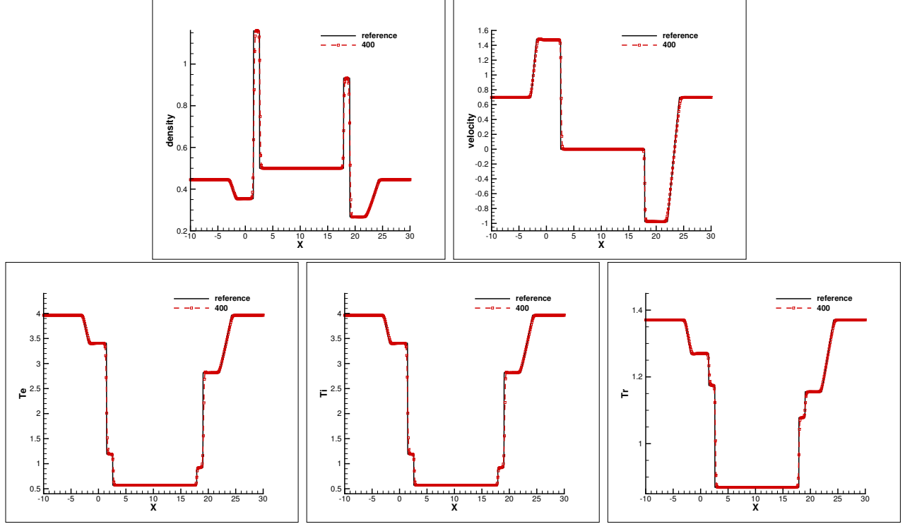
Figure 5.1: The numerical results for Example 5.2 at T = 1 by the fifth order finite difference scheme solving the 1D 3-T RH equations (3.1)-(3.2) without the diffusion and energy-exchange terms on the 400 grid. Left and Top: density, Right and Top: velocity, Left and Bottom: electron temperature, Middle and Bottom: ion temperature, Right and Bottom: radiation temperature.
