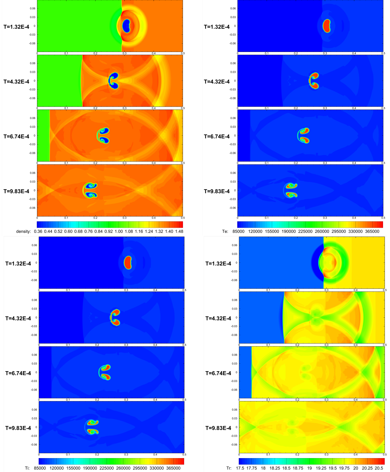
Figure 5.8: The numerical results for Example 5.7 by the fifth order finite difference scheme solving the 2D 3-T RH equations (4.1)-(4.2) with w_{ei} = w_{er} = 0 and \kappa_e = \kappa_i = \kappa_r = 0 at the different times on the 800 \times 288 grid. Left and Top: density, Right and Top: electron temperature, Left and Bottom: ion temperature, Right and Bottom: radiation temperature.
