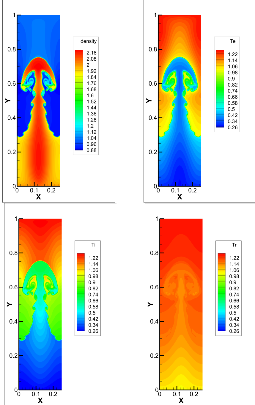
Figure 5.10: The numerical results for Example 5.8 by the fifth order finite difference scheme solving the 2D 3-T RH equations (4.1)-(4.2) at T = 1.95 on the 200 \times 1200 grid. Left and Top: density, Right and Top: electron temperature, Left and Bottom: ion temperature, Right and Bottom: radiation temperature.
