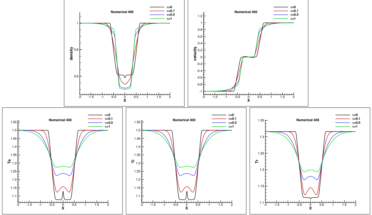
Figure 5.4: The numerical results for Example 5.4 at T = 0.2 by the fifth order finite difference scheme solving the 3-T RH equations (3.1)-(3.2) with the different \kappa_e, \kappa_i, \kappa_r on the 400 grid. Left and Top: density, Right and Top: velocity, Left and Bottom: electron temperature, Middle and Bottom: ion temperature, Right and Bottom: radiation temperature.
