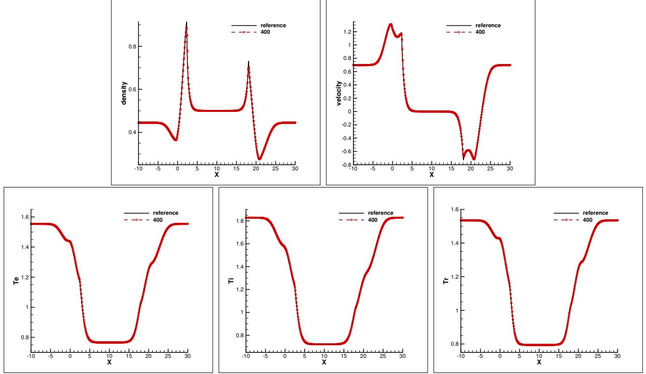
Figure 5.2: The numerical results for Example 5.2 at T = 1 by the fifth order finite difference scheme solving the 1D 3-T RH equations (3.1)-(3.2) with w_{ei} = w_{er} = 1 and \kappa_e = \kappa_i = \kappa_r = 1 on the 400 grid. Left and Top: density, Right and Top: velocity, Left and Bottom: electron temperature, Middle and Bottom: ion temperature, Right and Bottom: radiation temperature.
