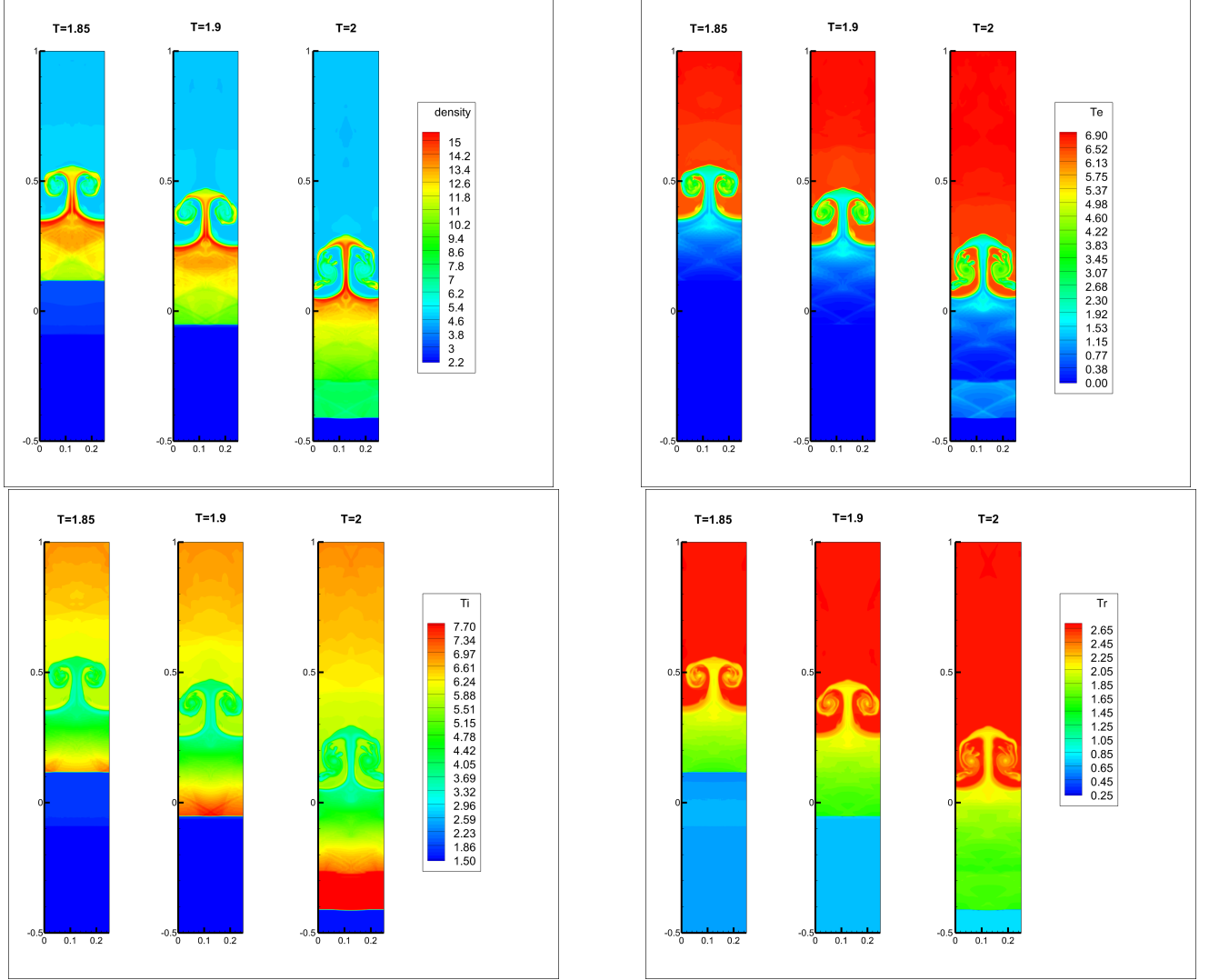
Figure 5.11: The numerical results for Example 5.9 by the fifth order finite difference scheme solving the 2D 3-T RH equations (4.1)-(4.2) with w_{ei} = w_{er} = 0 and \kappa_e = \kappa_i = \kappa_r = 0 at different times on the 200 \times 1200 grid. Left and Top: density, Right and Top: electron temperature, Left and Bottom: ion temperature, Right and Bottom: radiation temperature.
