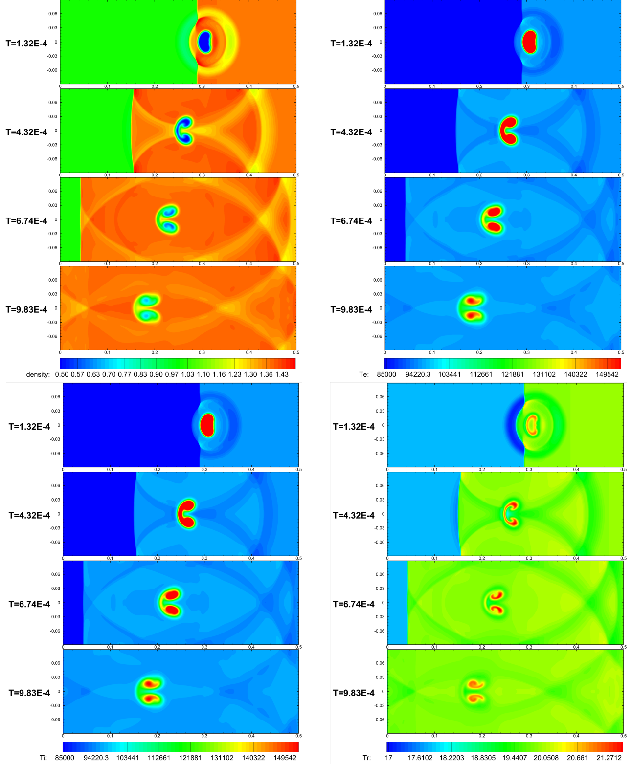
Figure 5.9: The numerical results for Example 5.7 by the fifth order finite difference scheme solving the 2D 3-T RH equations (4.1)-(4.2) with w_{ei} = 0.05 , w_{er} = 0 and \kappa_e = \kappa_i = \kappa_r = 0.05 at the different times on the 800 \times 288 grid. Left and Top: density, Right and Top: electron temperature, Left and Bottom: ion temperature, Right and Bottom: radiation temperature.
