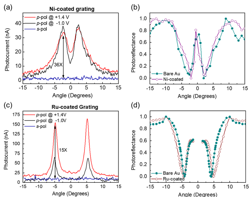
Figure 5. (a) Angle-dependent photocurrent spectra of Ni-coated gold grating nanostructure. (b) Photoreflectance spectra with and without nickel coating. (c) Angle-dependent photocurrent spectra of Ru-coated gold grating nanostructure. (d) Photoreflectance spectra with and without ruthenium coating.
