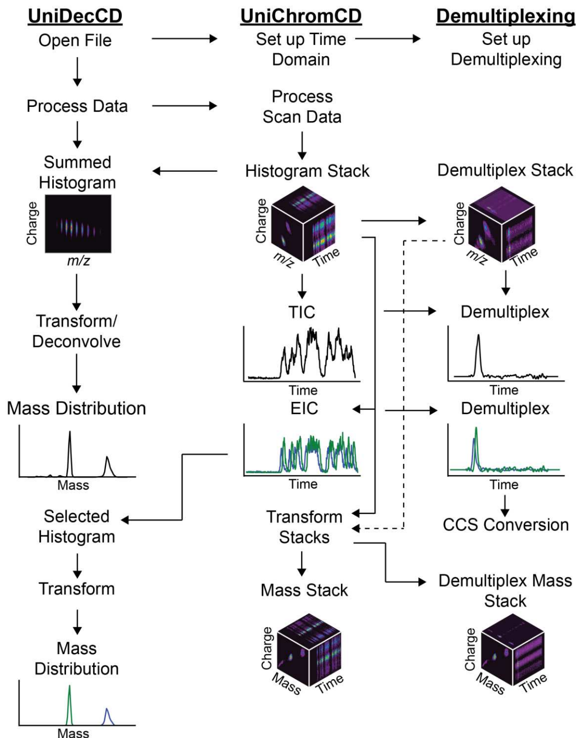
Figure 2. Flowchart showing the data flow and interactions between the different programming classes of UniChromCD. Files are opened using the existing UniDecCD code, but new elements in UniChromCD and the demultiplexing engine (DM) set up the required time-domain information and prepare the demultiplexing kernels. After the data is processed in UniDecCD, UniChromCD parses the processed data into a histogram stack and creates the TIC. EICs can be extracted from the summed histogram, which can then be processed with UniDecCD to yield extracted mass distributions. The entire histogram stack can also be transformed to convert the m/z axis to mass. At any point, the TIC, EIC, m/z histogram stack, or mass histogram stack can be demultiplexed. EICs from FT-IM data can be further converted from drift time into CCS. The dashed arrow is only dashed to make it easier to follow.
