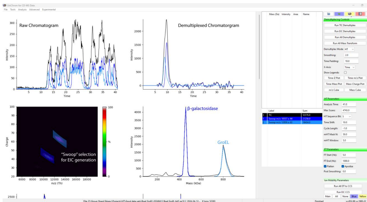
Figure 1. UniChromCD GUI with example data displayed. The raw chromatogram and EICs are displayed in the top left plot. Demultiplexed chromatograms/arrival time distributions are displayed in the top right plot. A 2D m/z vs. charge histogram of CD-MS data is displayed in the bottom left plot, and the mass distribution in the bottom right. Additional plots are not shown but can be accessed by scrolling down. The newly added green control panels include Demultiplexing Controls, HT Parameters, FT Parameters, and Ion Mobility Parameters and are shown to the far right.
