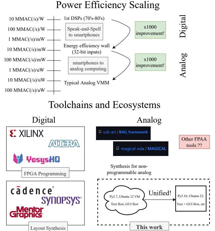
Fig. 1. The power and area efficiency gains of the analog domain motivate the need for analog computing applications. This figure highlights the disparity in ecosystems between the two computing paradigms, and shows how this work contributes to closing the gap.
