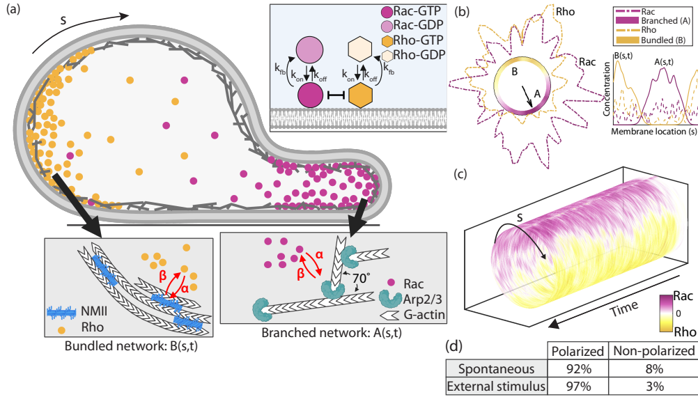
Fig 1. Model for spontaneous polarity in individual cells. (a) Side view schematic of front-rear polarity markers in a cell. Top inset: GTP-GDP cycling dynamics of Rho GTPases in the model. Bottom insets: Local, bidirectional crosstalk (red arrows) between Rho and actomyosin bundles (left) and Rac and Arp2/3 branched F-actin networks (right) ensures the simultaneous spatial organization of two distinct F-actin networks supporting the formation of a cell rear and front, respectively. (b) The outcome of one model realization shown with two representations: along circular boundary and along periodic 1D domain (inset). In the circular representation, heatmap plots of the branched (magenta) and bundled (yellow) F-actin networks are shown inside the cell. The GTPase concentrations, Rac (magenta) and Rho (yellow), are plotted outside the cell membrane. A front-rear polarity axis is drawn with a black arrow. Inset: same simulation output along the 1D periodic domain with continuous lines for F-actin structures and dashed lines for Rac/Rho molecules. (c) Rac and Rho concentrations in space and time averaged over 100 independent realizations – a cylinder slice corresponds to the concentrations at one fixed time point. (d) Summary of polarization probability for 100 realizations.
