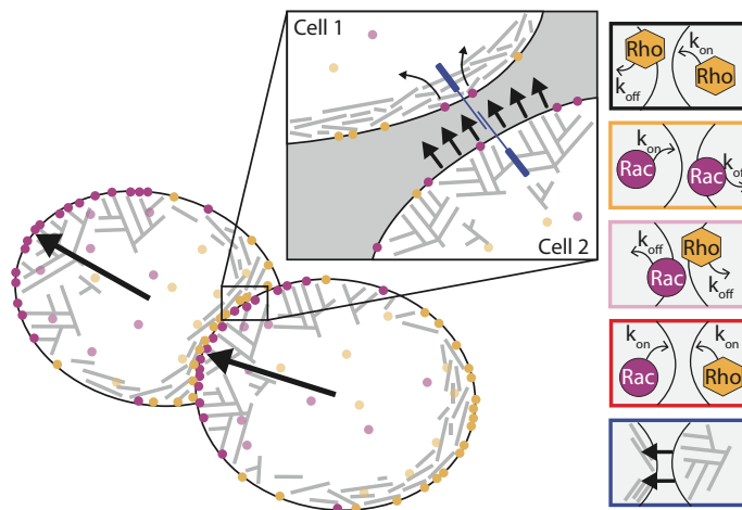
Fig 8. Illustration of the working principles underlying the set of intercellular interactions for collective orientation of polarity in a pair of cells. Inset illustrates our hypothesis that protrusive forces could drive enhanced dissociation of Rac in neighboring cell through mechanosensitive junction proteins.
