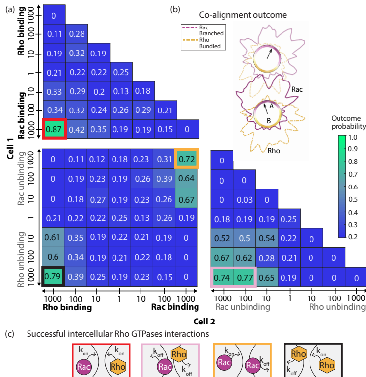
Fig 3. Probabilities of co-alignment arrangement under the assumption of intercellular regulation of Rho GTPase kinetics. (a) The co-alignment outcome probabilities for systematic combinations of amplified binding ( k_{on} , boldface) and/or unbinding ( k_{off} , gray) rates of Rac and/or Rho at the intercellular junction. The numerical value and box color represent the outcome probability for doublet co-alignment arrangement. The numbers along the axes indicate the amplification factor ( \gamma ) while the label indicates which rate, in which cell, was affected. Modifications done in cell 1 are shown along the y -axis, and cell 2 along the x -axis. The outlined boxes indicate successful interactions, and the color corresponds to the interaction motif in (c). (b) Sample doublet simulation resulting in co-alignment arrangement. Different opacity is used to distinguish between the cells. (c) Emergent successful intercellular pathways based on Rho GTPase signaling.
