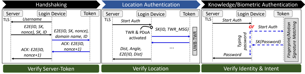
Figure 6: UWB-Auth authentication protocol verifies the legitimacy of the token, and verifies that the user can prove their identity. UWB-Auth th
