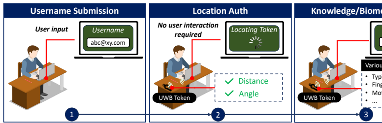
Figure 4: The user interactions in UWB-Auth during regular login.
