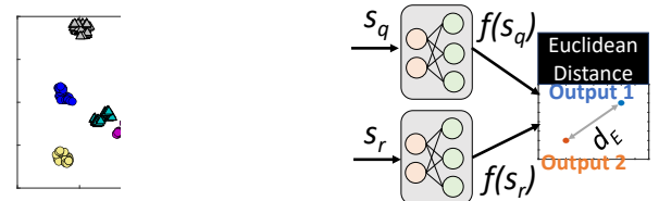
Figure 11: (Left) Feature visualization using t-SNE [51] of signatures written by 10 different users; (b) (Right) The forward process of Siamese network to compute signature similarity.
